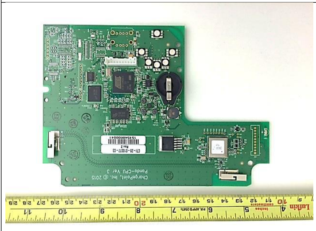
PCB Main Board- Bottom View
