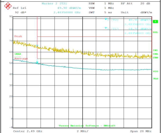
802.11g 2462M-Restricted Band 2483.5-2500MHz
