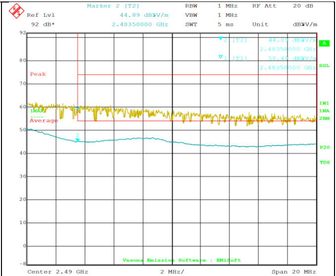
802.11b 2462M-Restricted Band 2483.5-2500MHz
