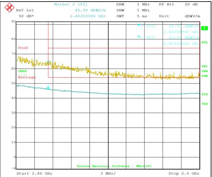
802.11n20 2462M-Restricted Band 2483.5-2500MHz
