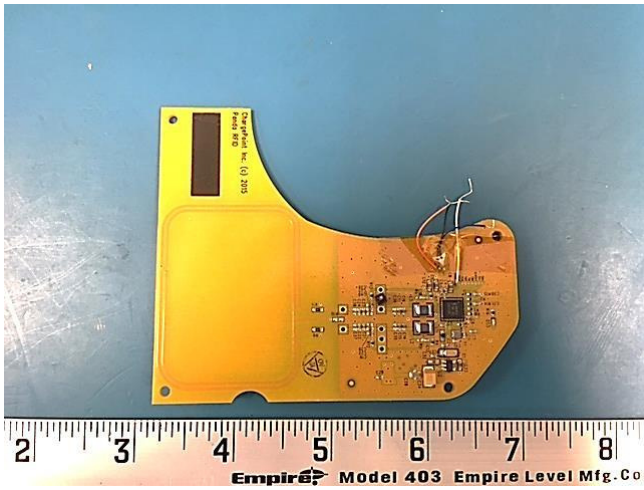
PCBA1 RFID - View 1
