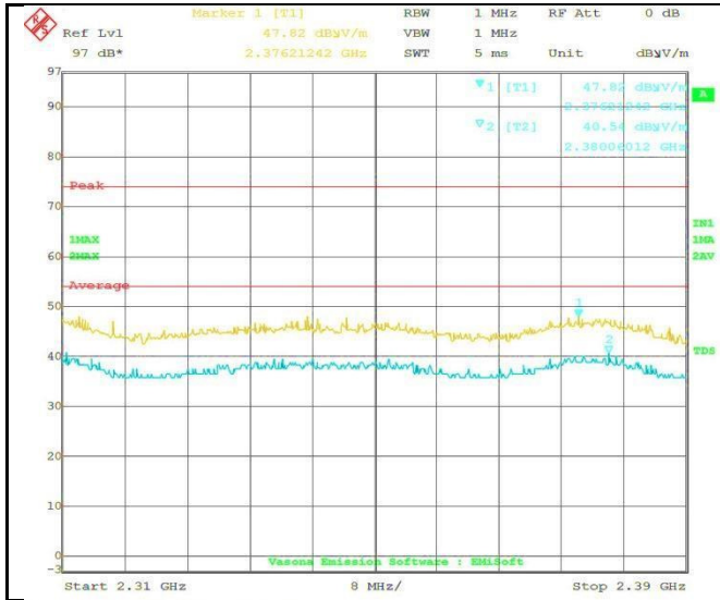
Restricted Band Low BLE
