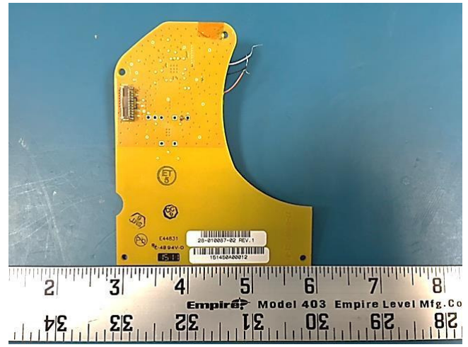
PCBA1 RFID - View 2
