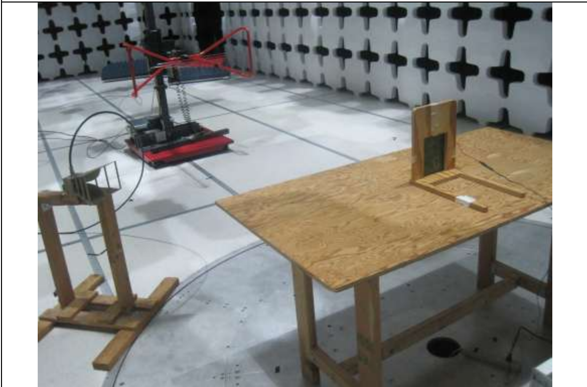
Radiated Emission Test Setup (30MHz – 1GHz) – Rear View
