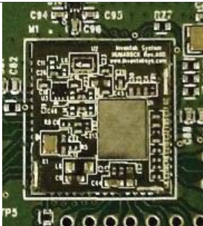
EUT Radio without shielding
