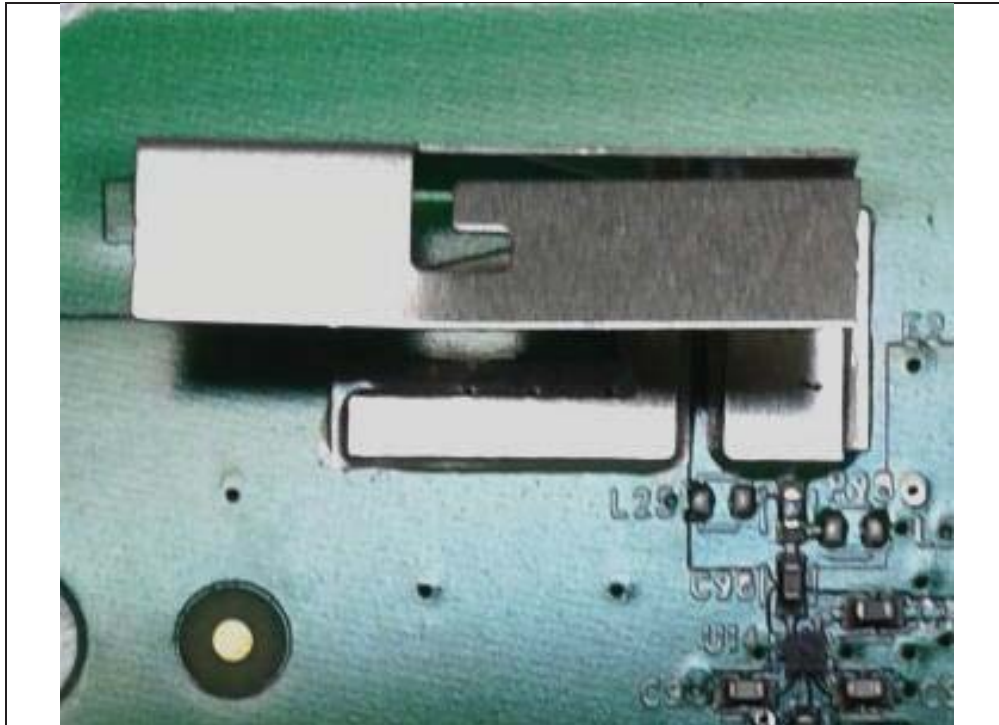
Antenna 1
