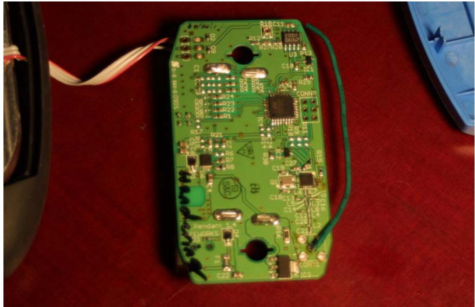
Radio and antenna are located in lower right corner of circuit board.
