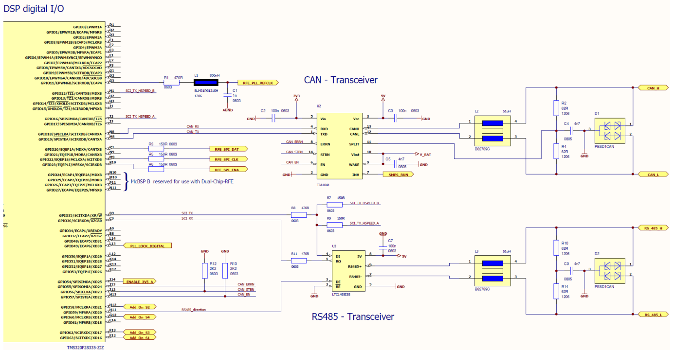
Figure 10: UMRR-0Axxxx DSP board schematics: CAN and RS485 transceivers
