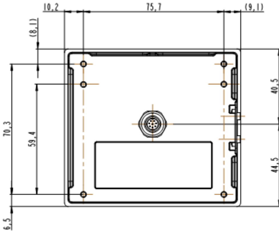
Figure 6: Sensor Rear Side.
