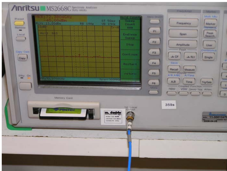
Connection between external mixer and local output from the Spectrum Analyzer
