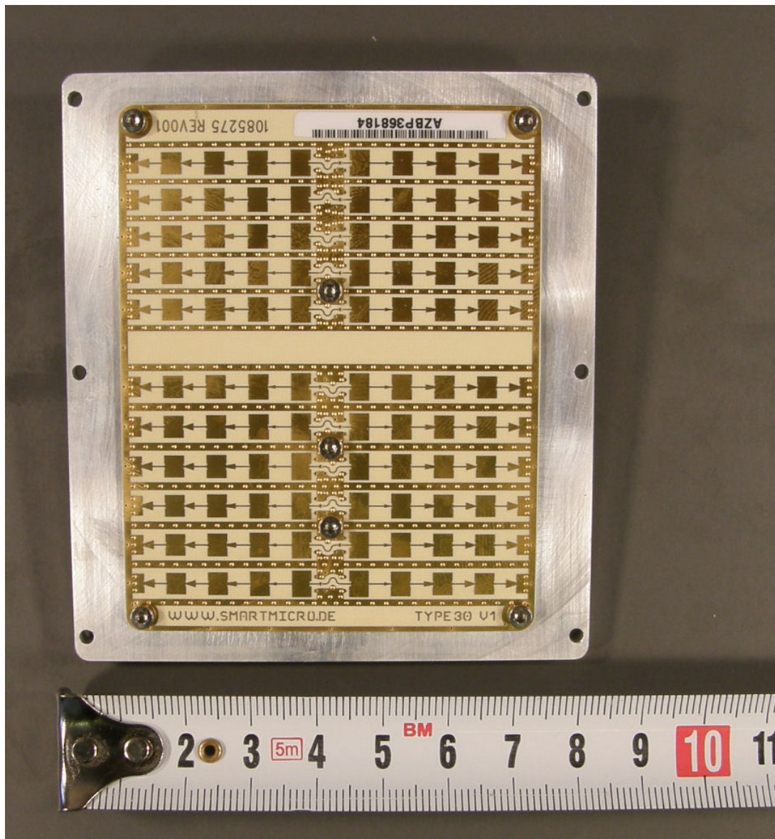
Antenna (front)
