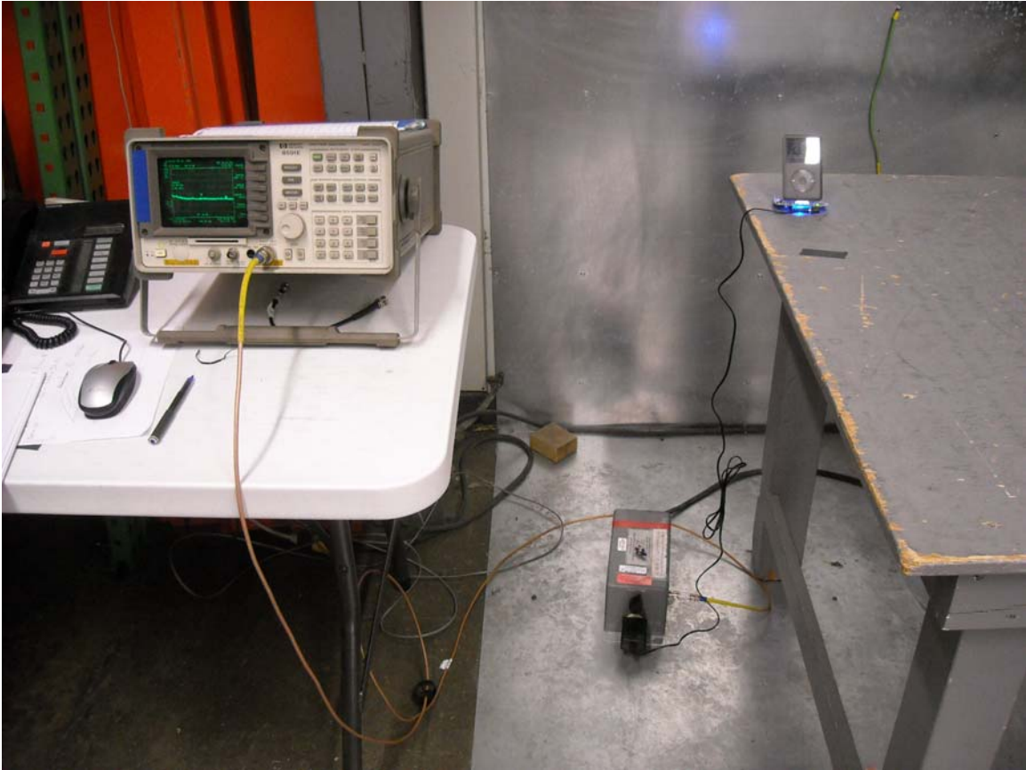
AC mains conducted EMI with a representative iPod configuration
