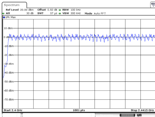
2402-2441 MHz
