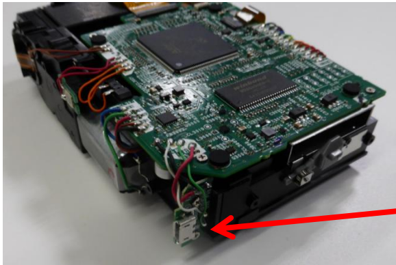
USB connector board
