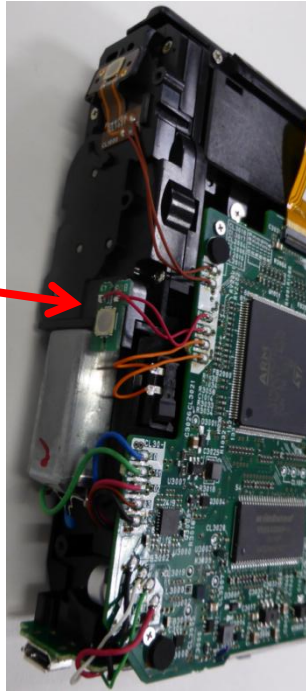
Side button board
