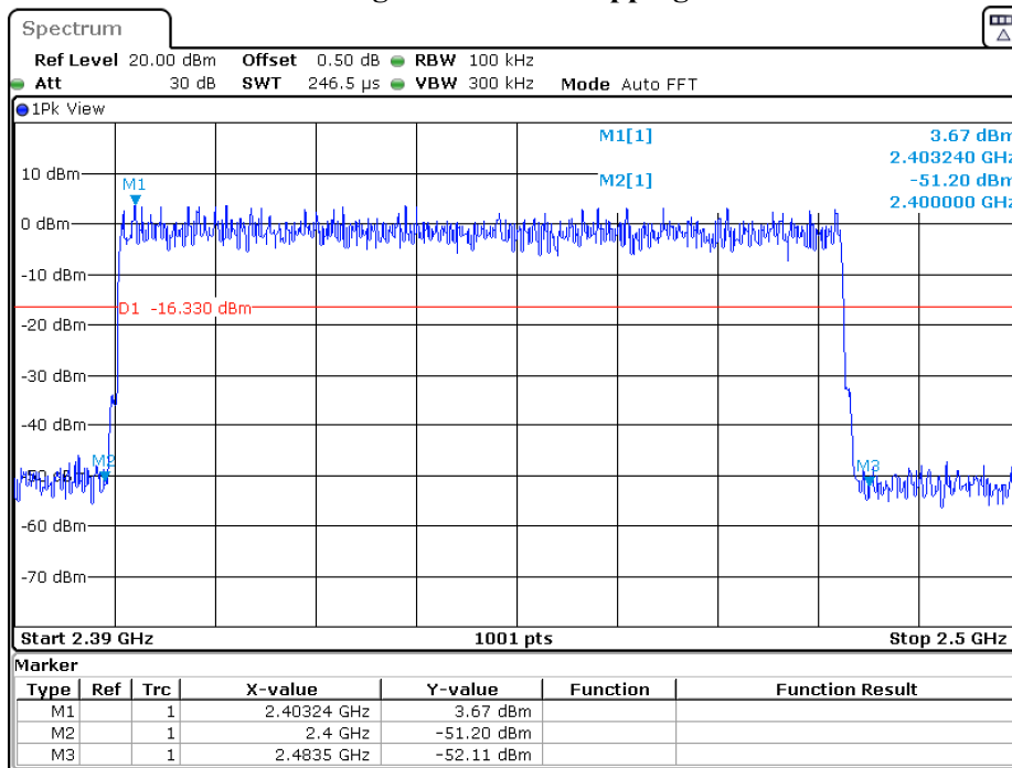
Figure Channel Hopping
