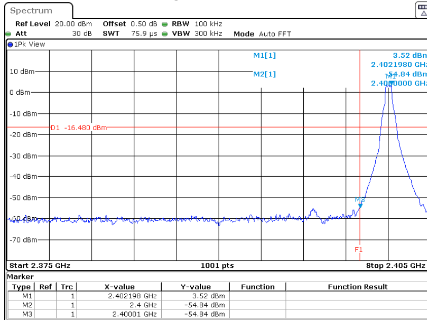
Figure Channel 00
