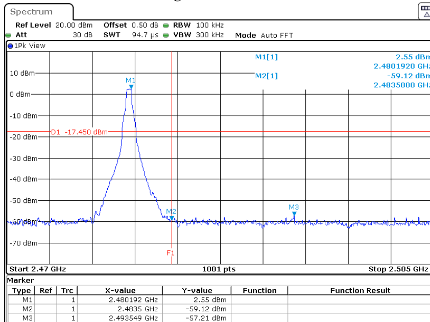
Figure Channel 78
