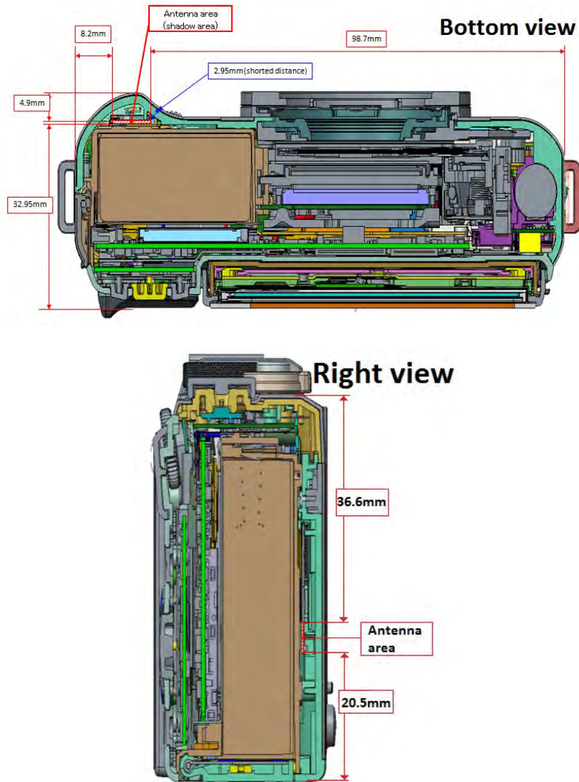
Fig.11 Antenna location
