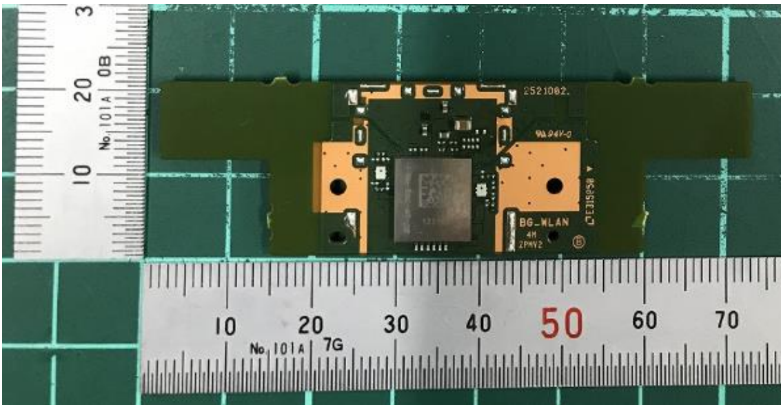
WLAN_FT_B
