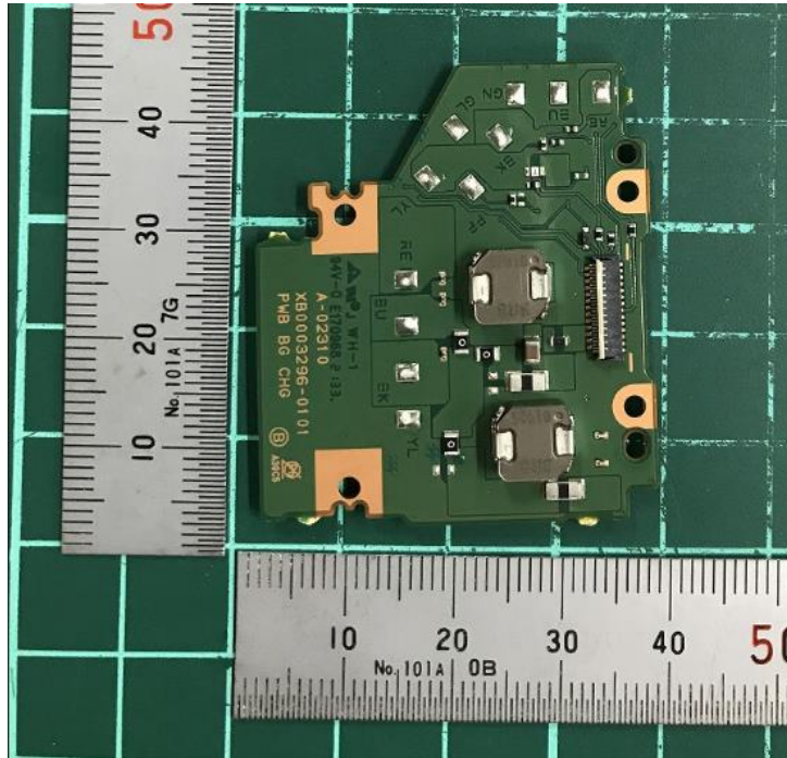
CHG_B
