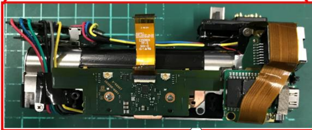
WLAN PCB
