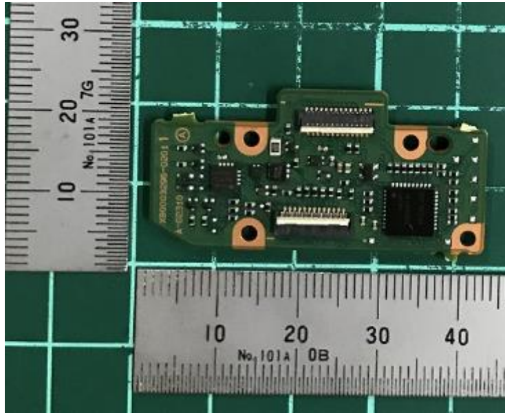
MIC_B
