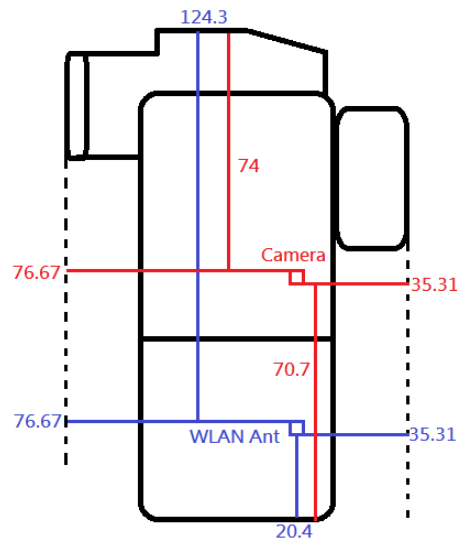
Photograph 8. Antenna position of EUT (Left view)
