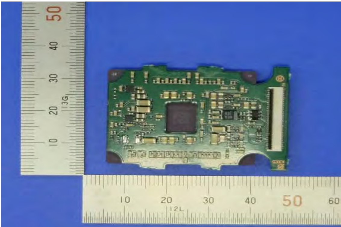
Internal View of EUT-2 (CMOS)
