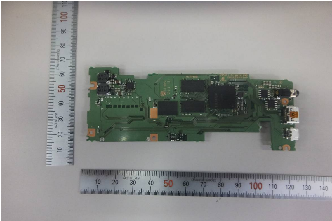
Internal View of EUT-4 (Main)
