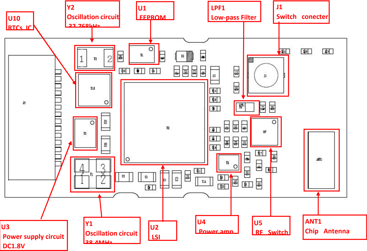
DWM-W078 parts layout drawi 2011/12/14
