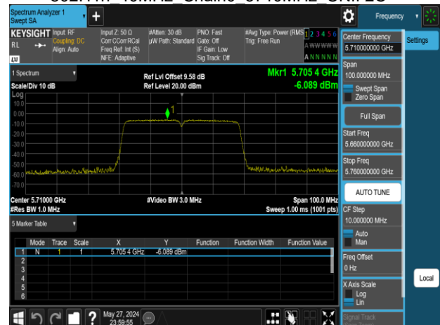
802.11n 40MHz Chain0 5710MHz UNII 2C
