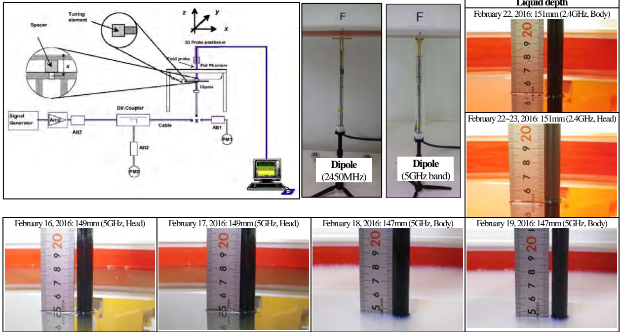
Test setup for the Daily check
