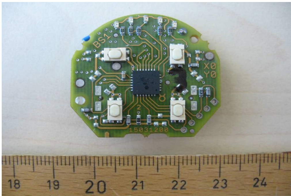
Photo 4: Transmitter
