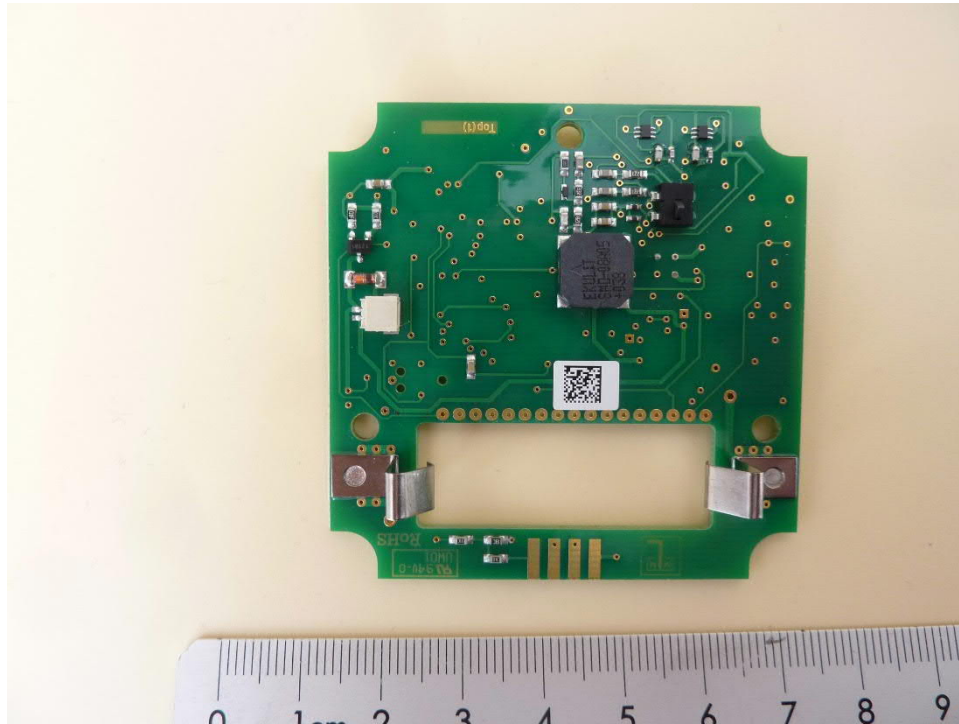
201474_pcb05: PCB top view
