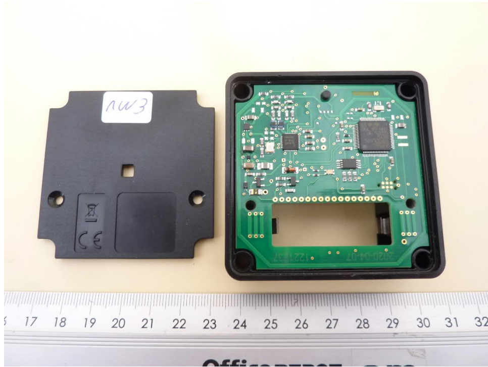
201474_pcb01: EUT inside view 1
