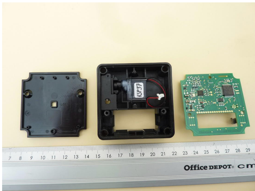
201474_pcb02: EUT inside view 2
