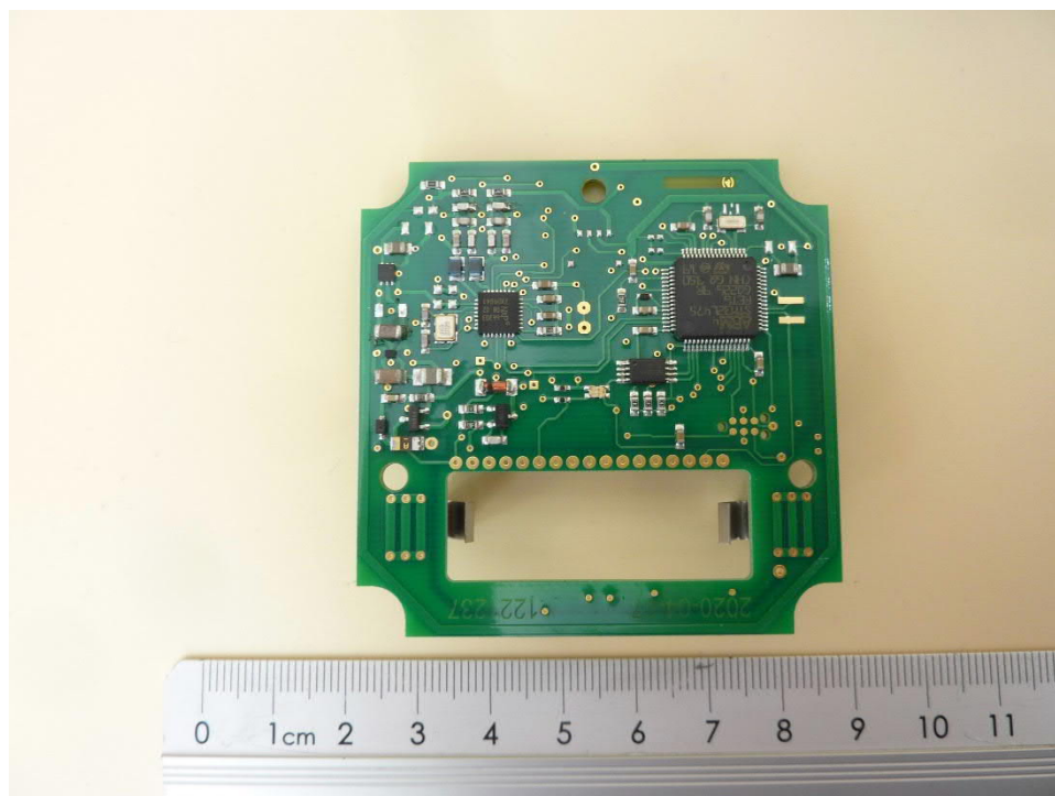
201474_pcb04: PCB bottom view
