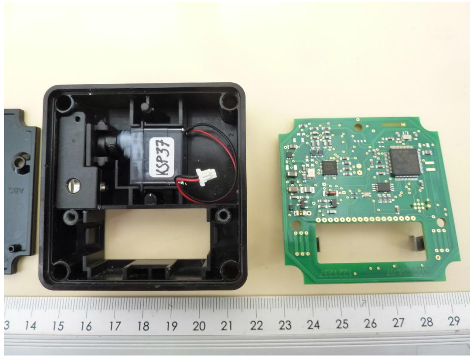
201474_pcb03: EUT inside view 3
