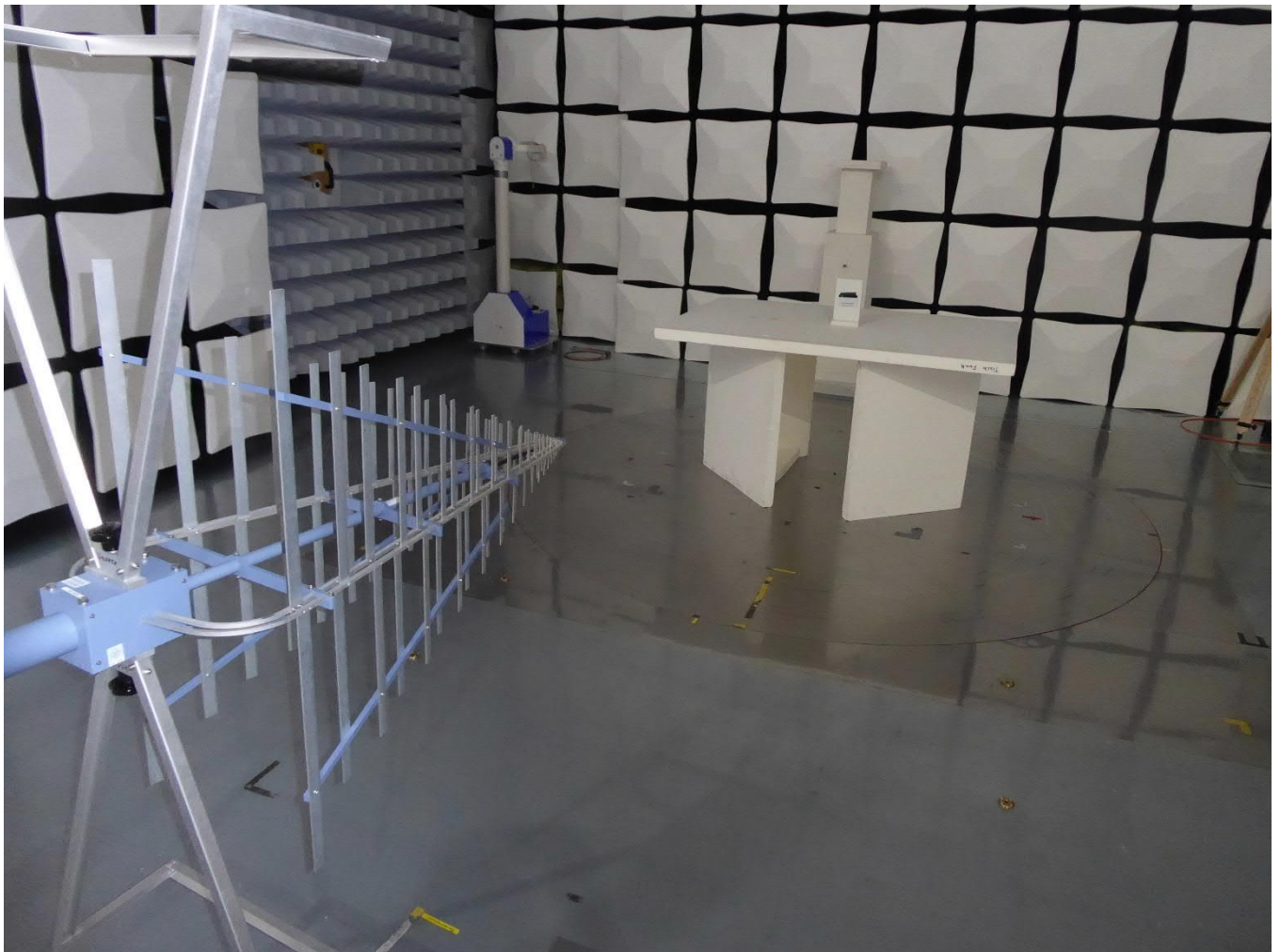
221308_03: Final measurement 30 - 1000 MHz
