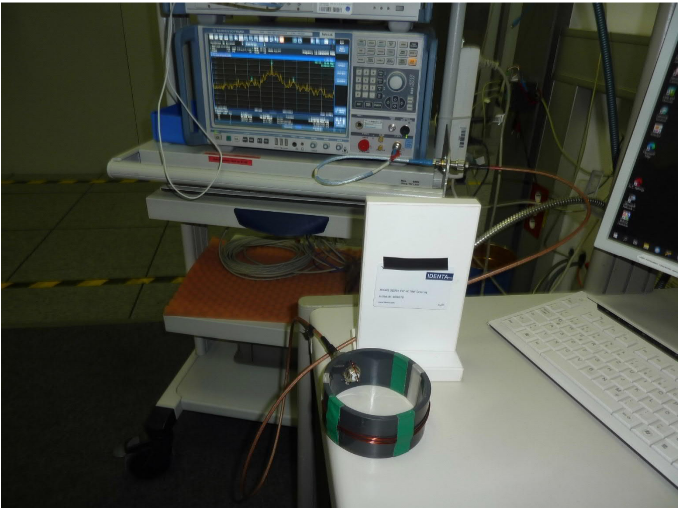
221308_05: Measurement 99 % bandwidth
