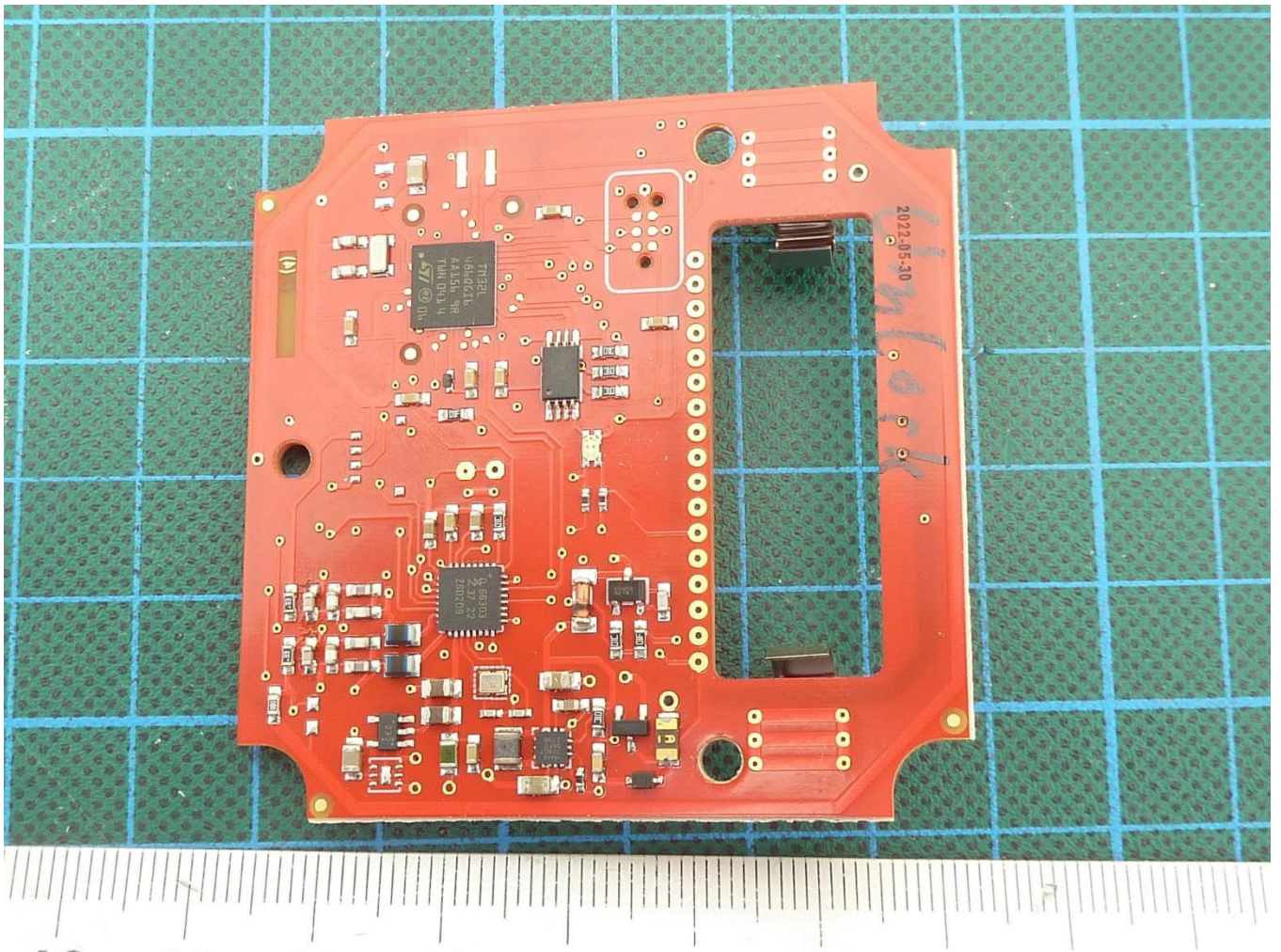
221308_eut08:PCB bottom view
