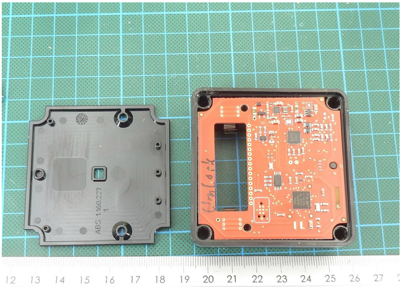
221308_eut05:EUT inside view 1
