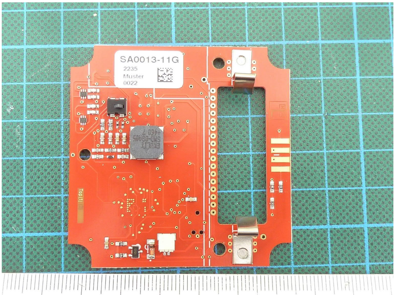
221308_eut07:PCB top view
