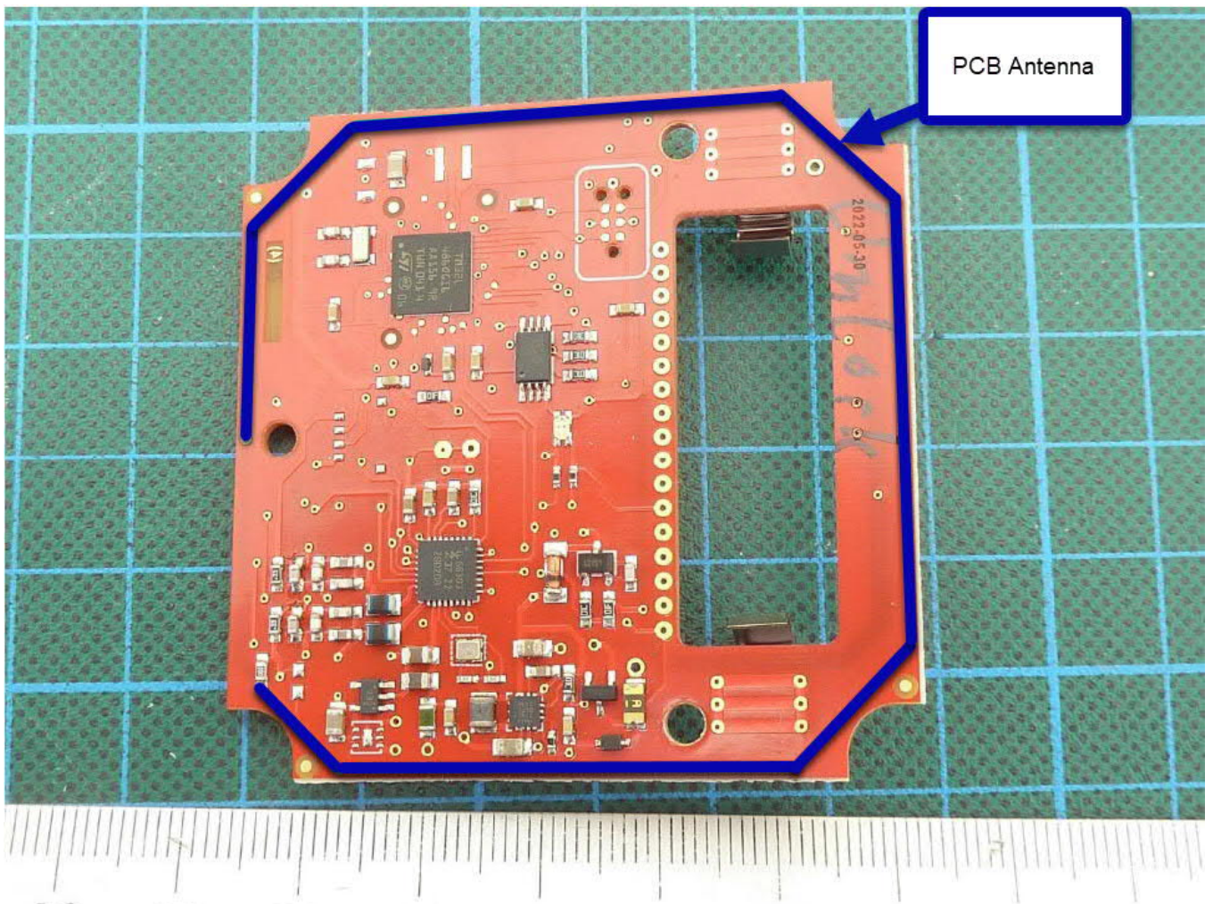
221308_eut09:PCB bottom view antenna
