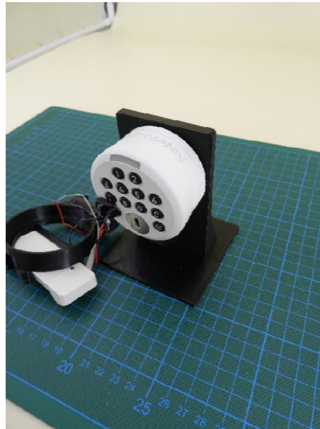
Modified EUT with mounted RFID reader for tests, view 2
