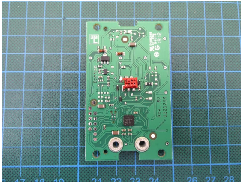
Keypad TA03 – PCB and keypad, view 2
