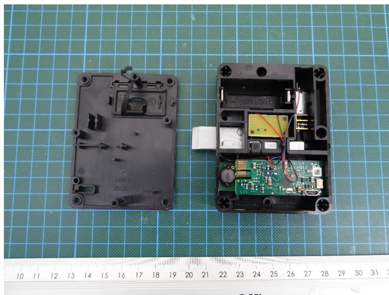
Lock M410 TA pro – cabinet opened
