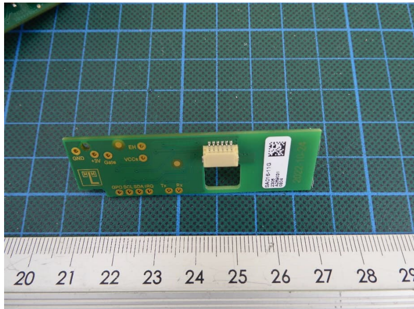
Lock M410 TA pro – PCB 2, view 1
