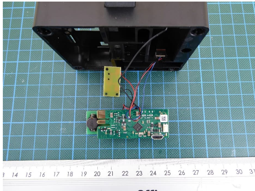
Lock M410 TA pro – PCB 1, view 1
