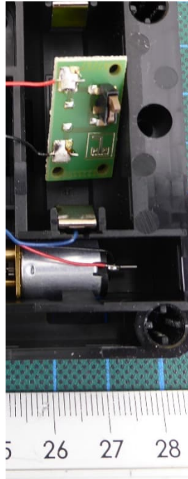
Lock M410 TA03 pro – PCB 3
