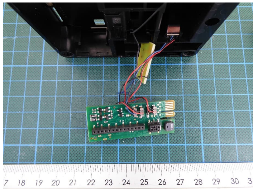
Lock M410 TA pro – PCB 1, view 2
