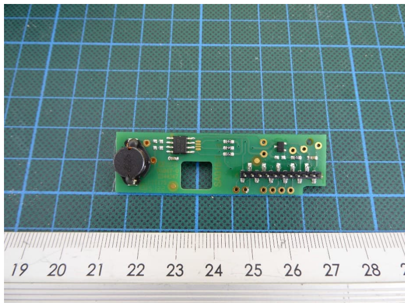
Lock M410 TA pro – PCB 2, view 2
