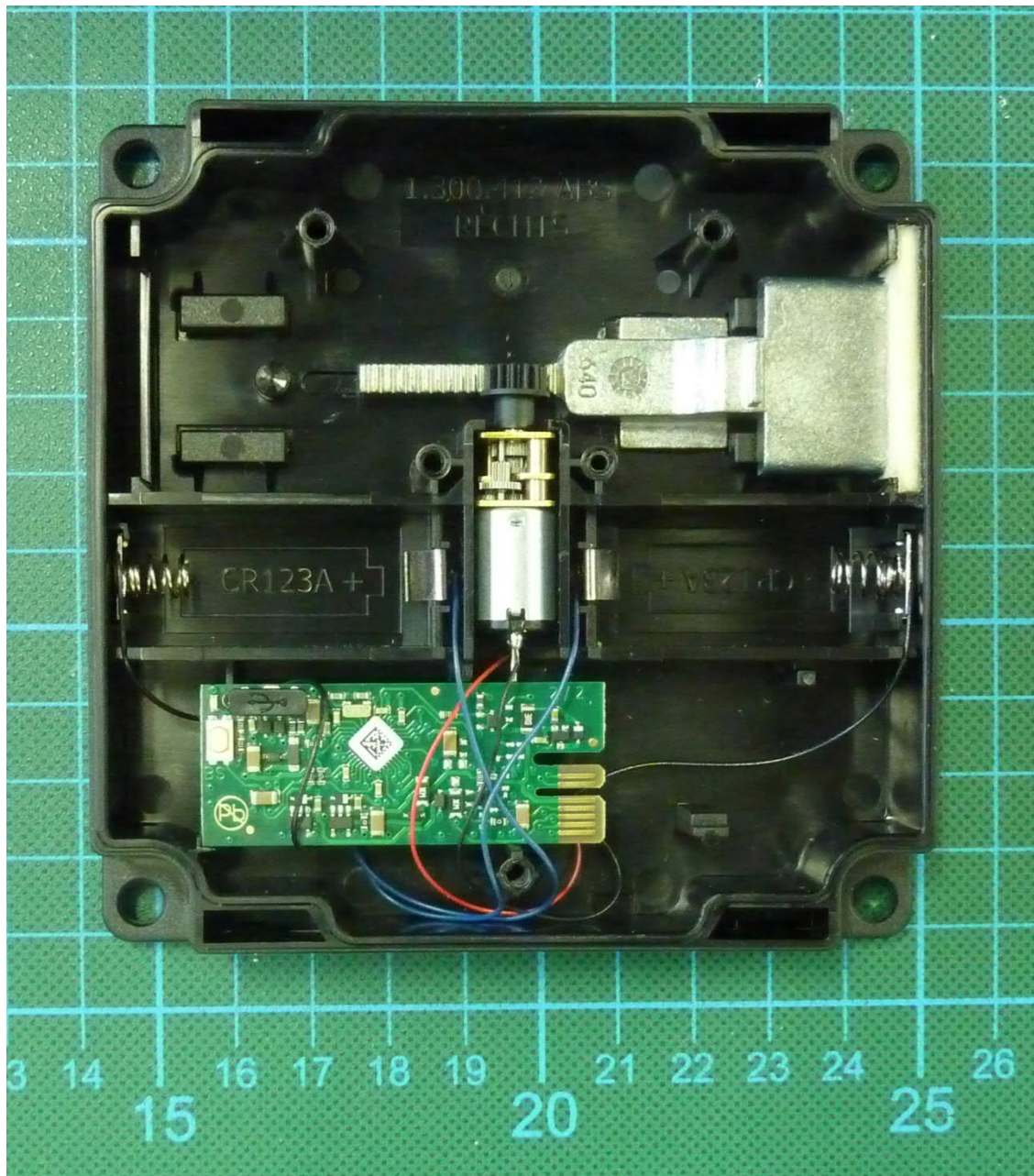
Lock M610 TA – Internal view
