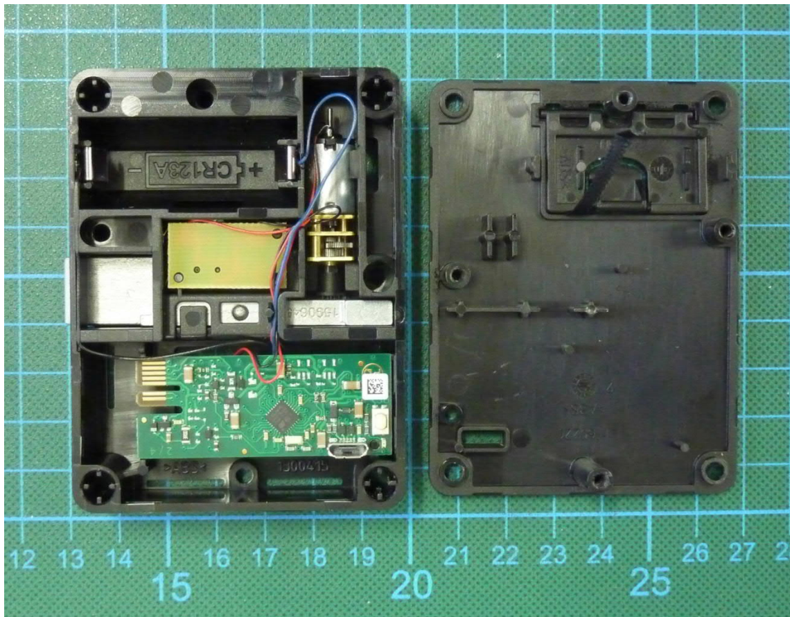
Lock M410 TA – cabinet opened
