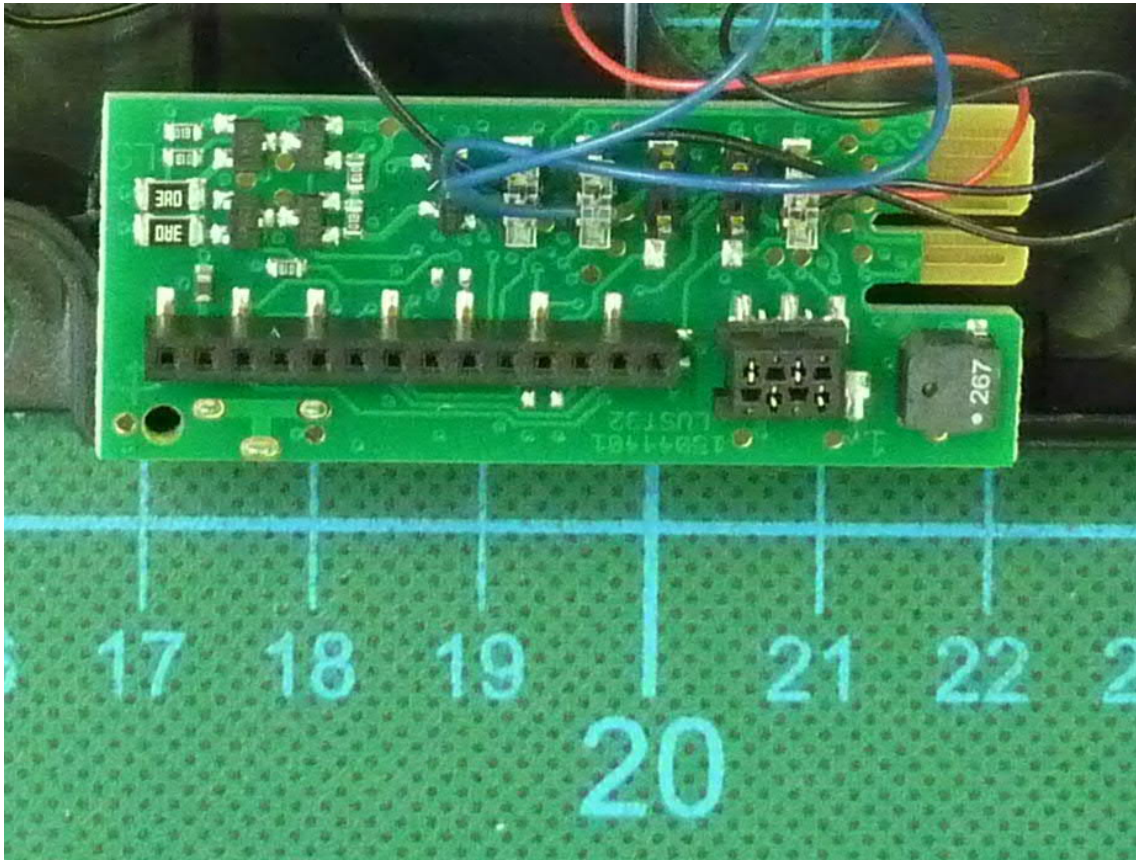
Lock M610 TA – PCB, view 2
