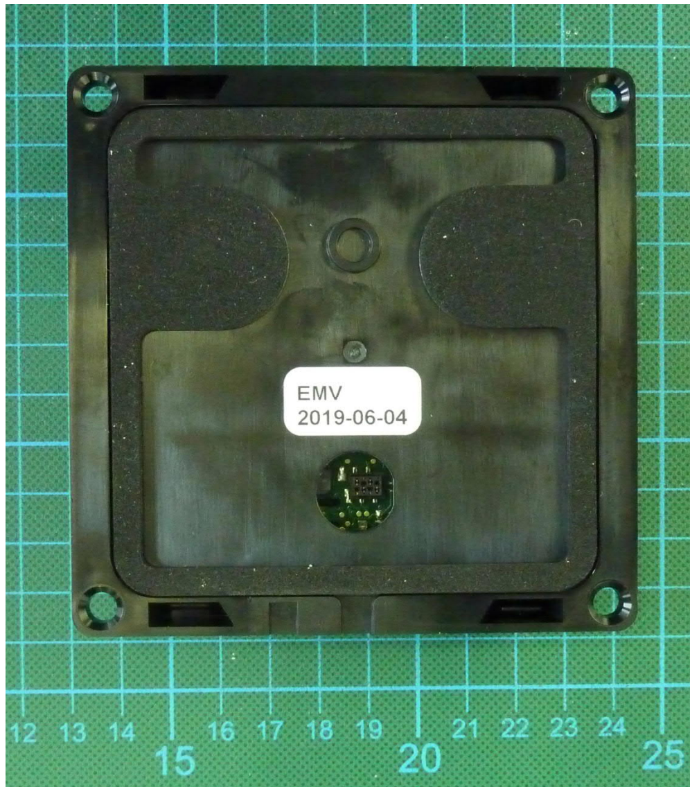
Lock M610 TA – Bottom view
