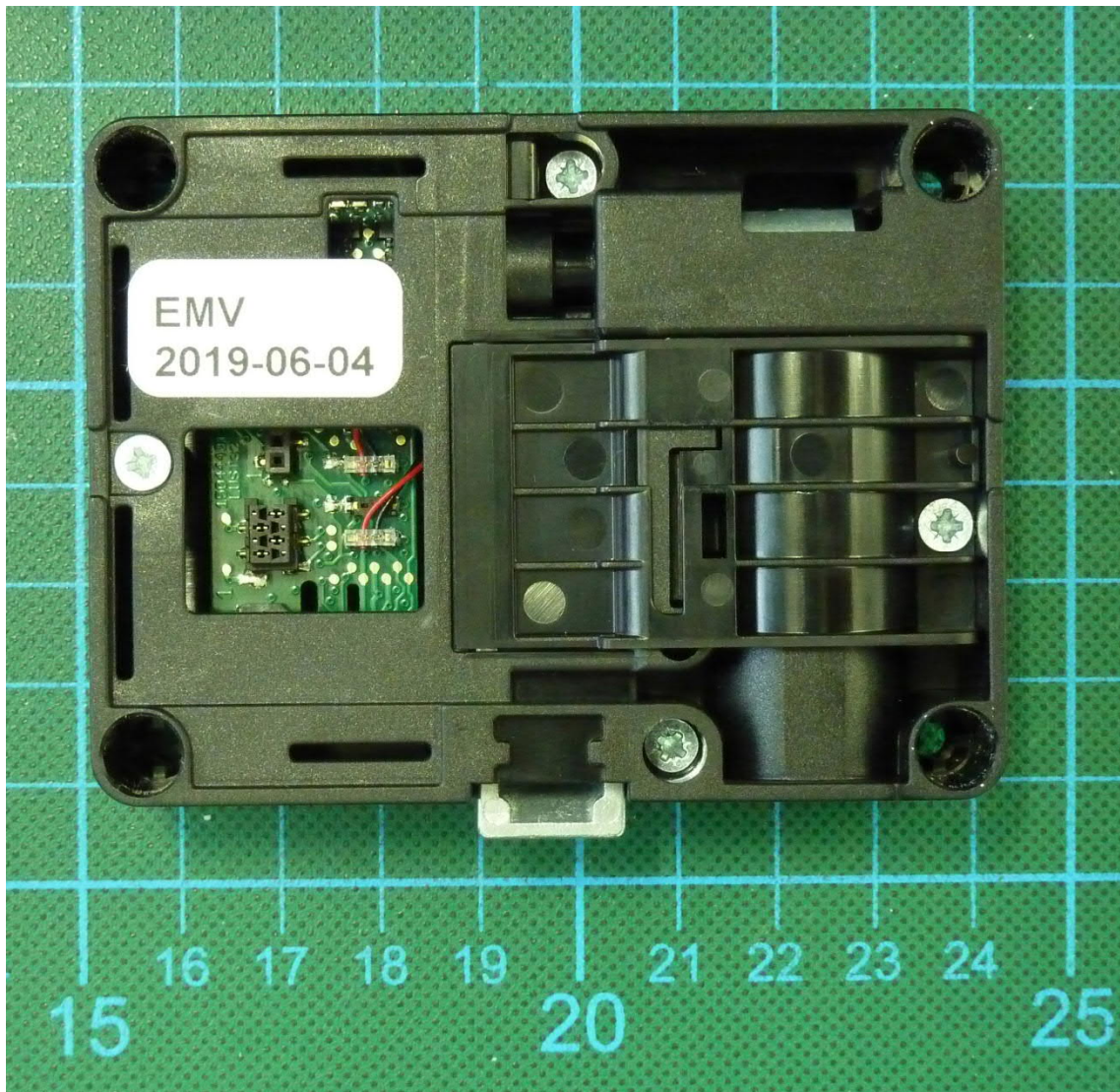
Lock M410 TA – bottom view
