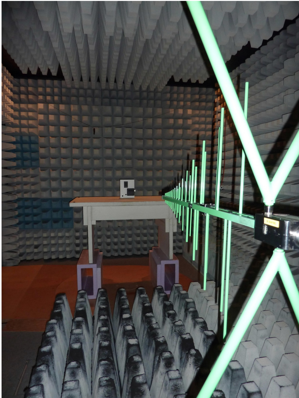
Keypad TA03 with lock M610 Test setup – preliminary measurement
