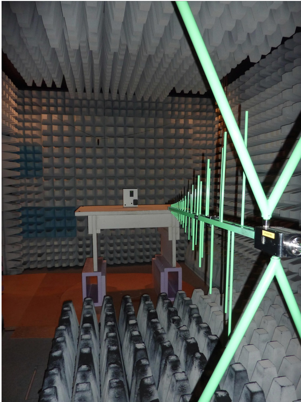
Keypad TA03 with lock M410 Test setup – preliminary measurement
