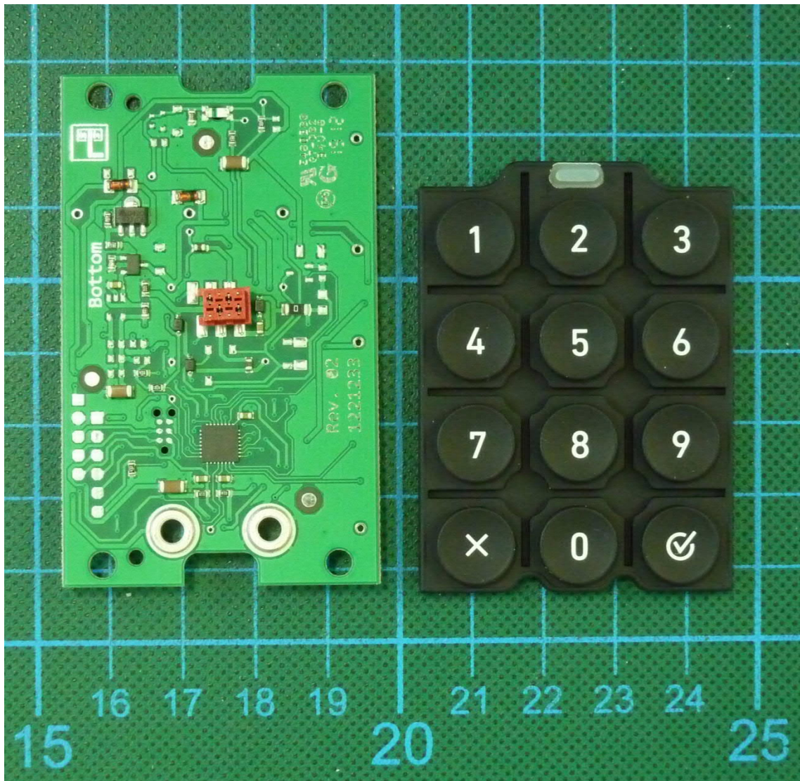
Keypad TA03 – PCB and keypad, view 1
