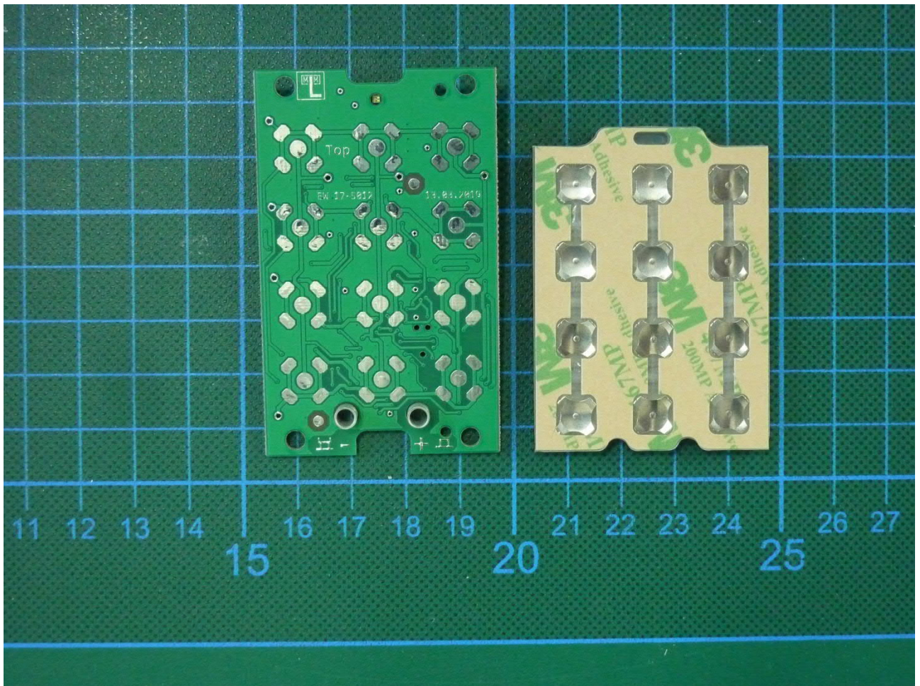
Keypad TA03 – PCB and keypad, view 2
