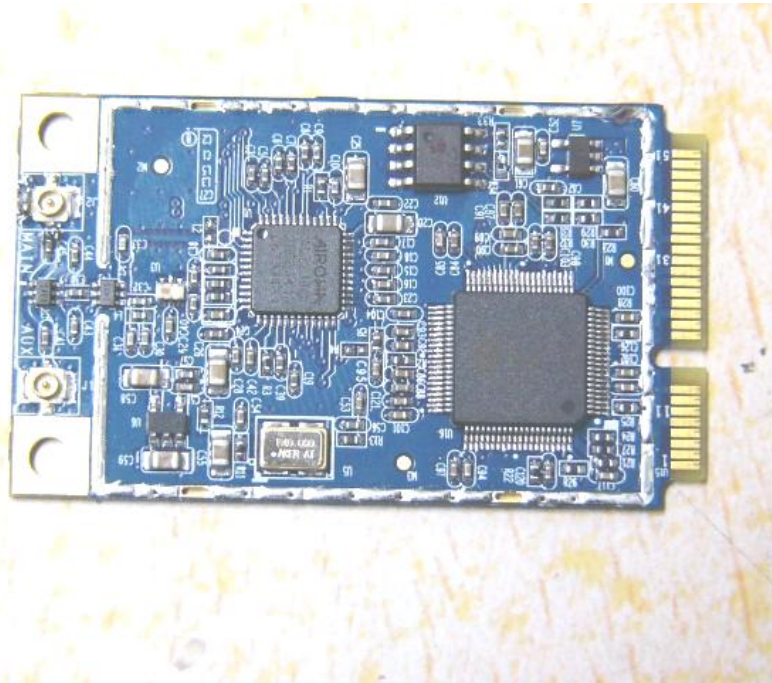
Main & RF board solder side
