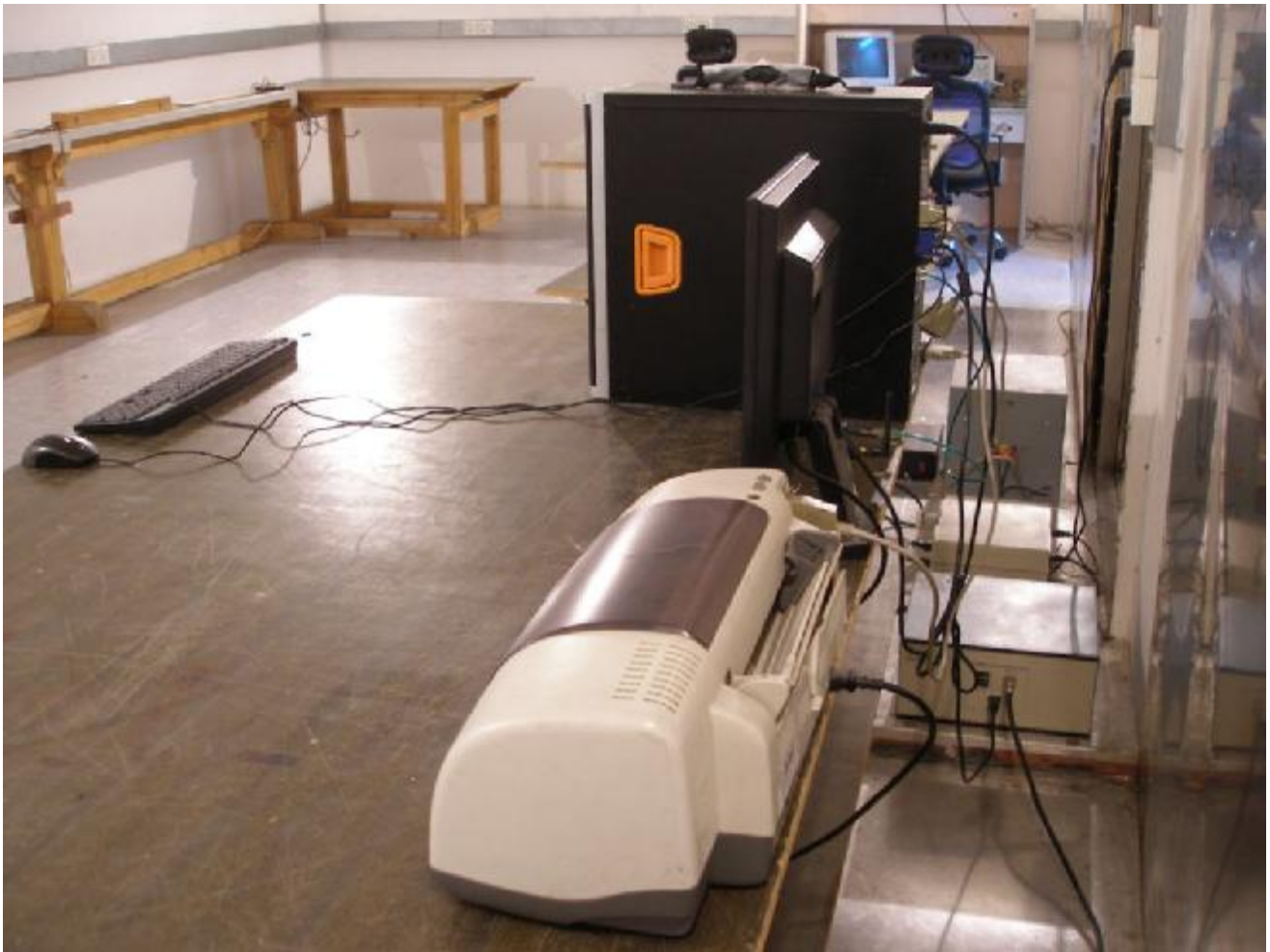
Conducted emission test view
