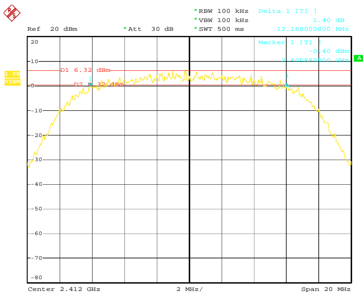
IEEE 802.11b 6dB Bandwidth (CH Low)
