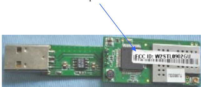
EUT Bottom View/Proposed FCC ID Label Location
