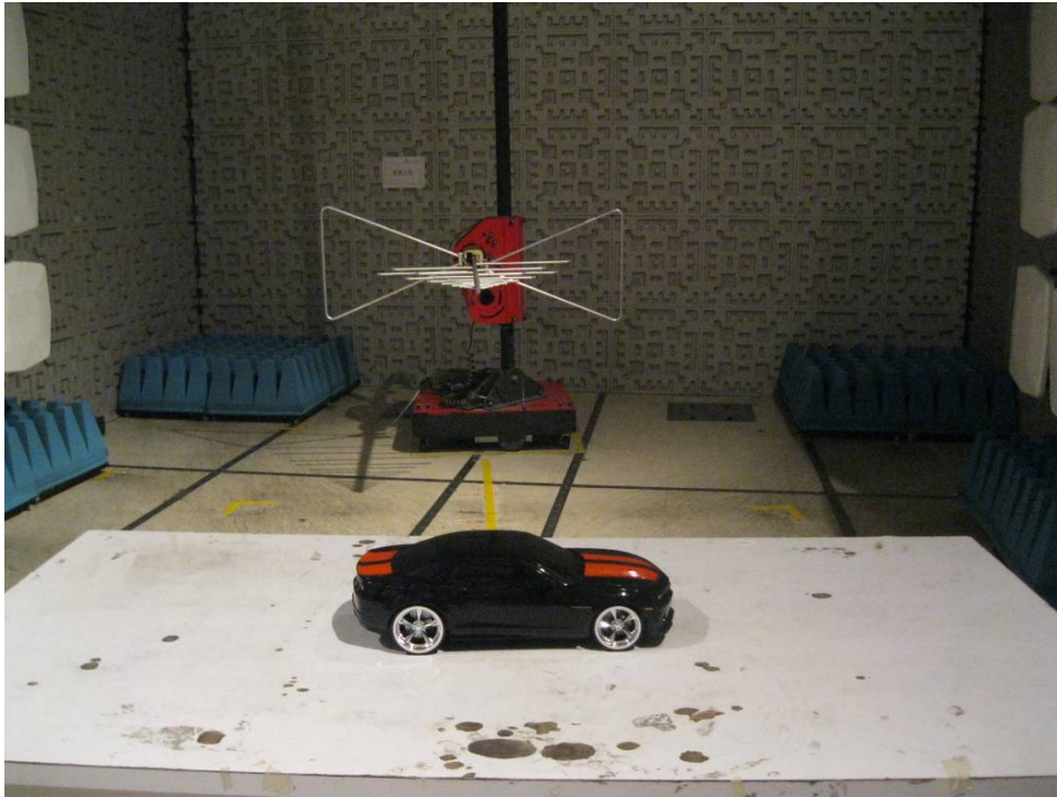
RADIATED EMISSION TEST SETUP-1
