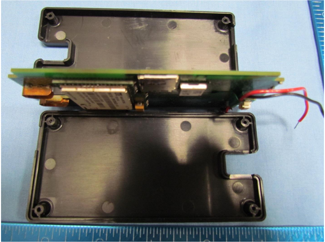
iTAG3G - Internal Side 2 View
