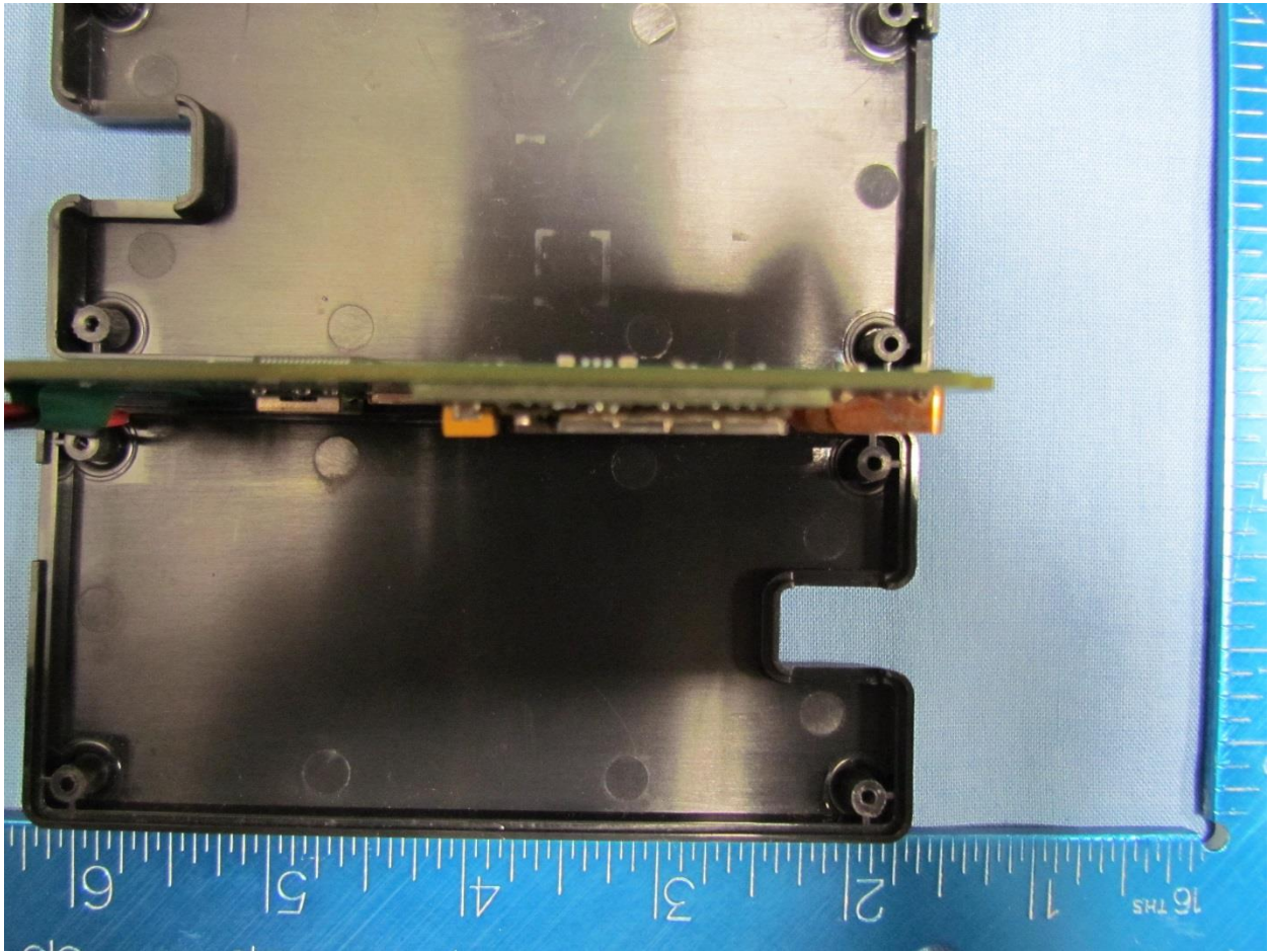
iTAG3G - Internal Side 1 View
