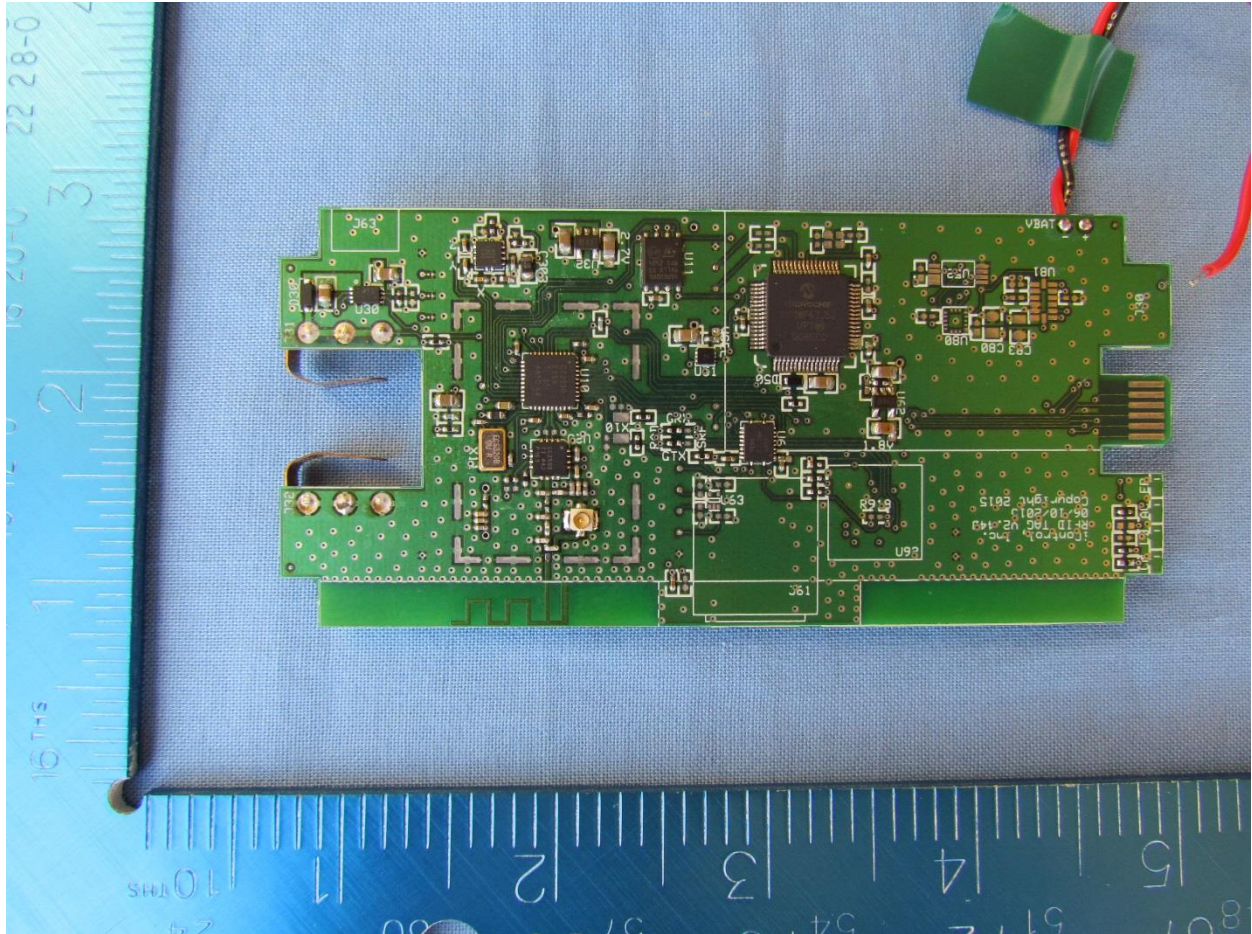
iTAG3G - Internal Bottom View
