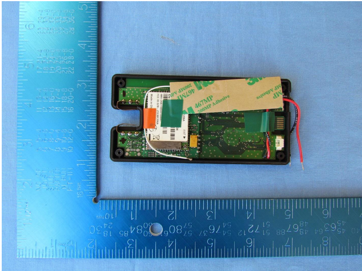
iTAG3G - Open Case
