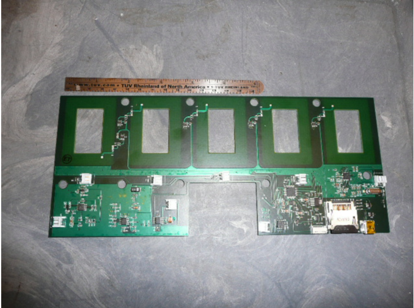
Figure 2 – Bottom side of board
