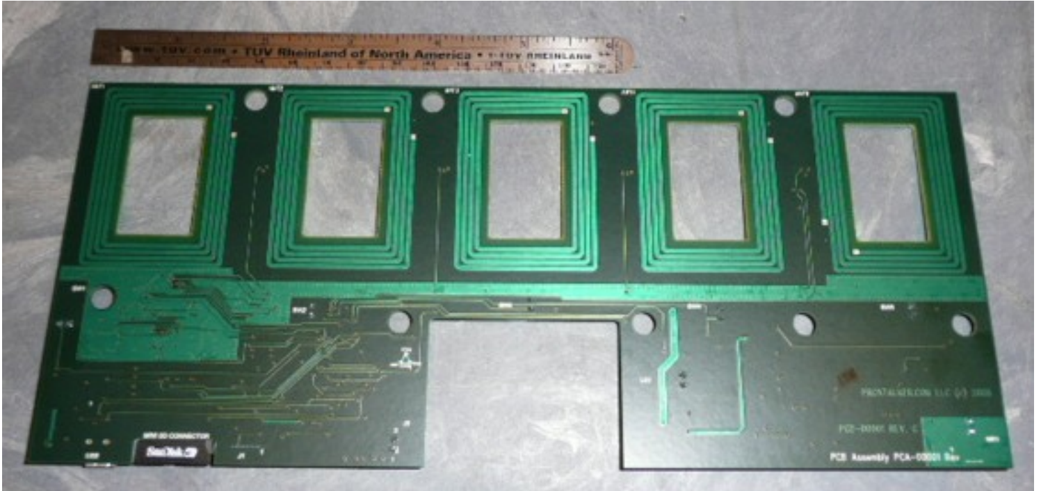
Figure 1 – The Transmitting antennae are the 5 identical rectangular loops (top side)
