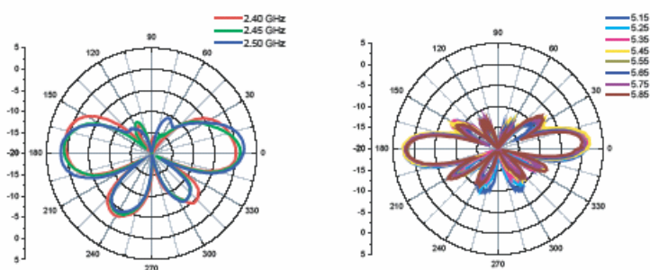
V-plane Co-polarization Pattern
