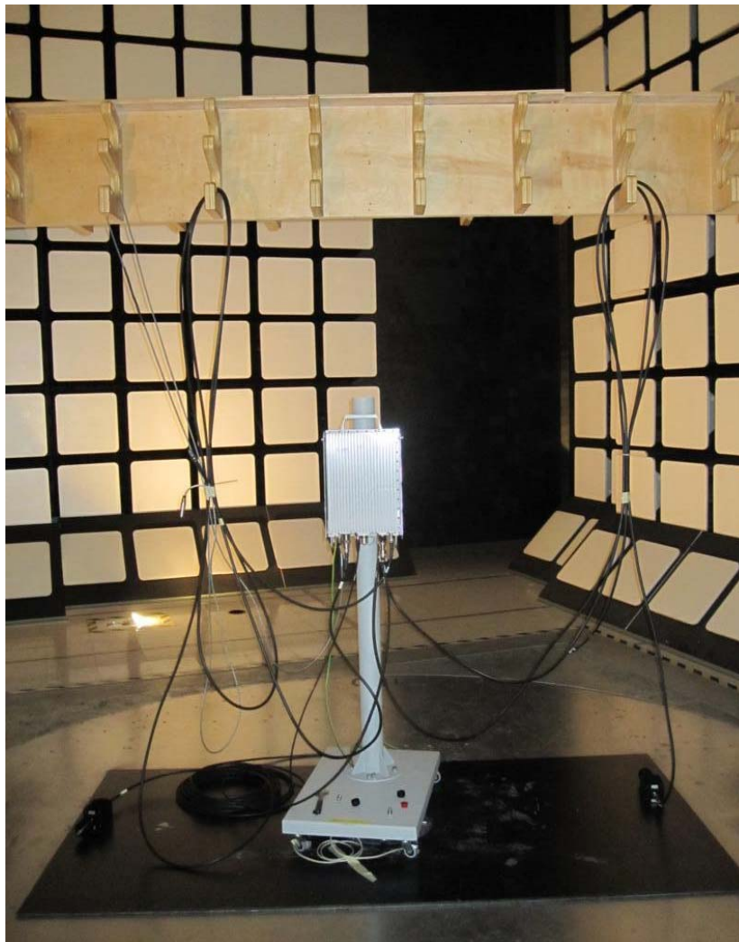
Figure 6-100: Radiated Emissions Set Up Photo
