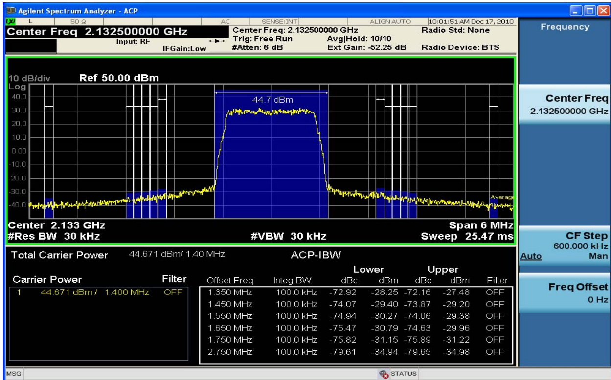
Figure 6-65 Spurious Emissions 2132.5MHz TX2_16QAM 1.4MHz Band Edge (ACP 650kHz – 2MHz)
