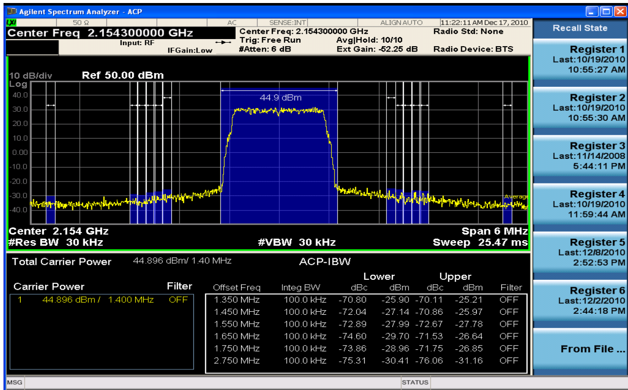
Figure 6-79 Spurious Emissions 2154.3MHz TX1_64QAM 1.4MHz Band Edge (ACP 650kHz – 2MHz)
