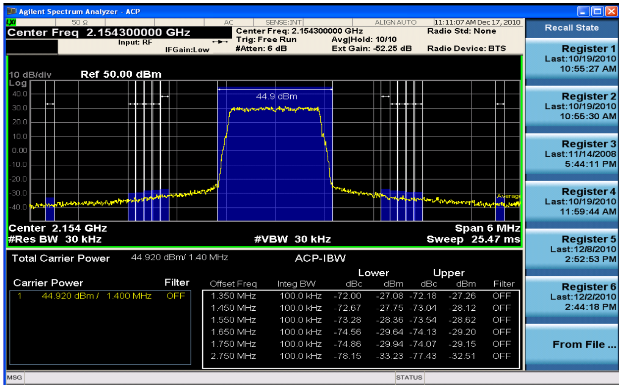
Figure 6-75 Spurious Emissions 2154.3MHz TX1_16QAM 1.4MHz Band Edge (ACP 650KHz – 2MHz)
