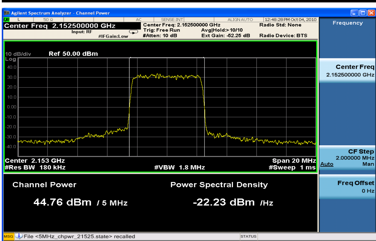
Figure 6-24 : 5MHz BW Channel Power TX1_64QAM at 2152.5 MHz
