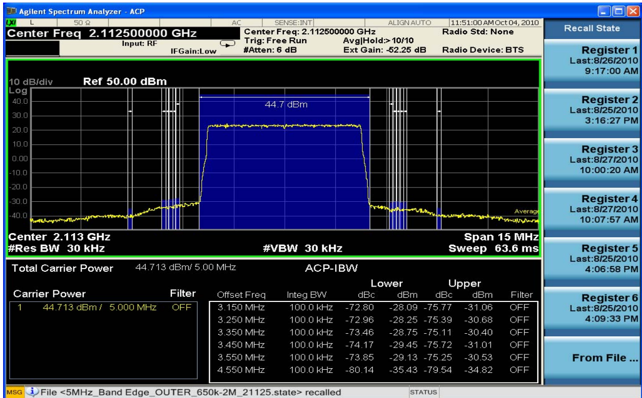
Figure 6-91 Spurious Emissions 2112.5MHz TX2_QPSK 5MHz Band Edge (ACP 650kHz – 2MHz)
