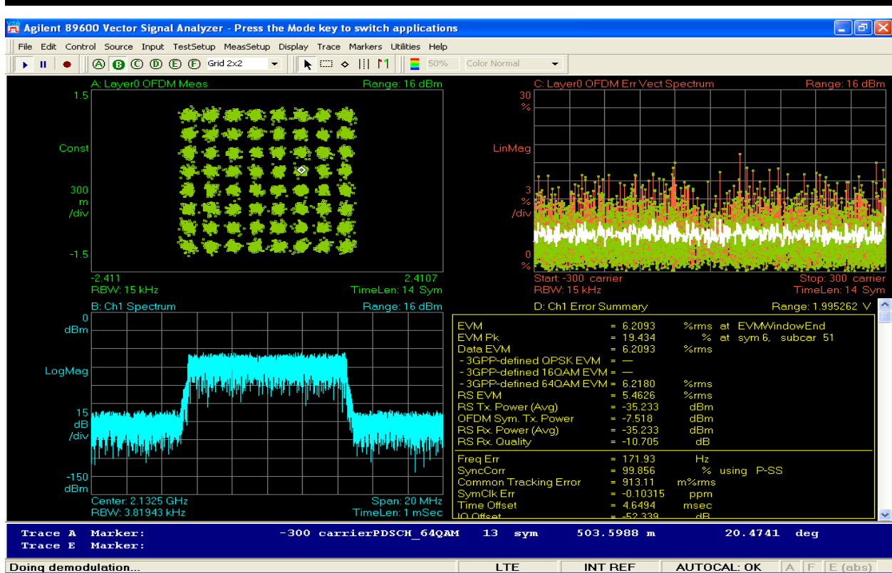
Figure 6-40 : 10MHz BW Modulation TX1_64QAM at 2132.5 MHz
