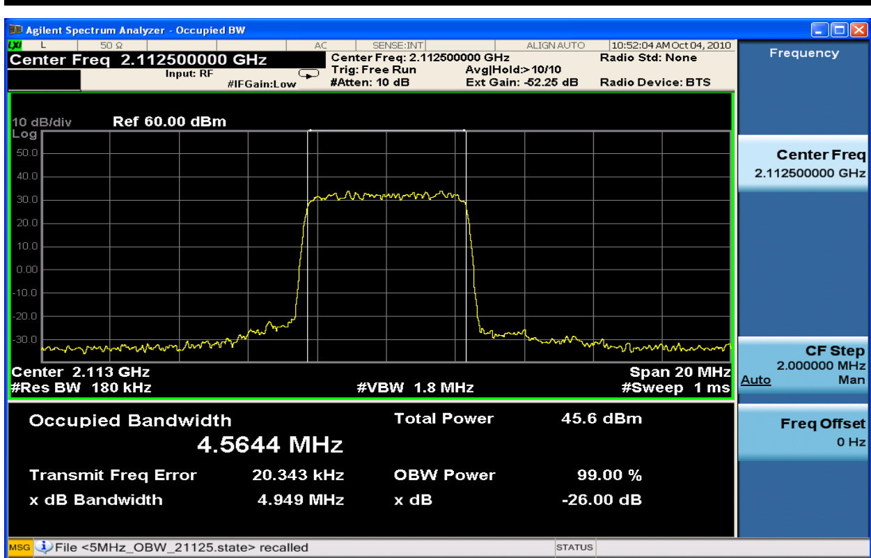
Figure 6-51: 5MHz Occupied Bandwidth TX1_QPSK at 2112.5 MHz
