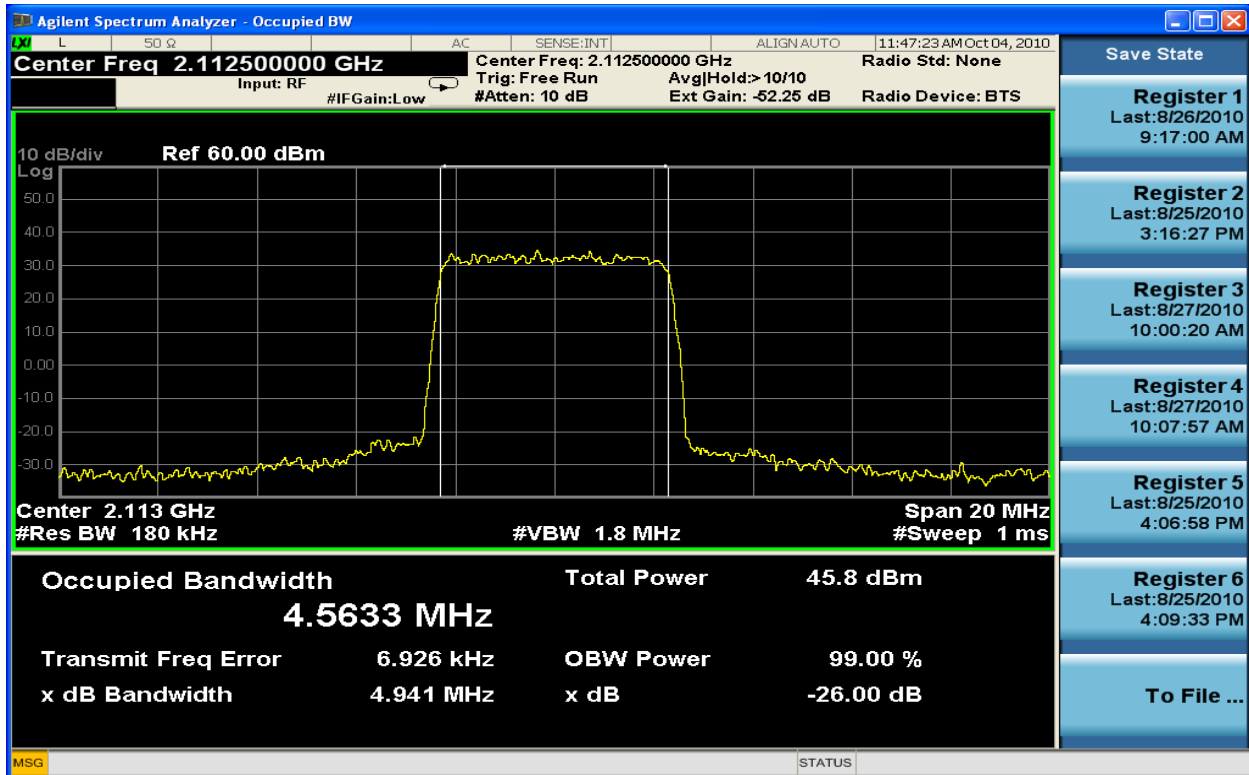
Figure 6-54: 5MHz Occupied Bandwidth TX2_16QAM at 2112.5 MHz
