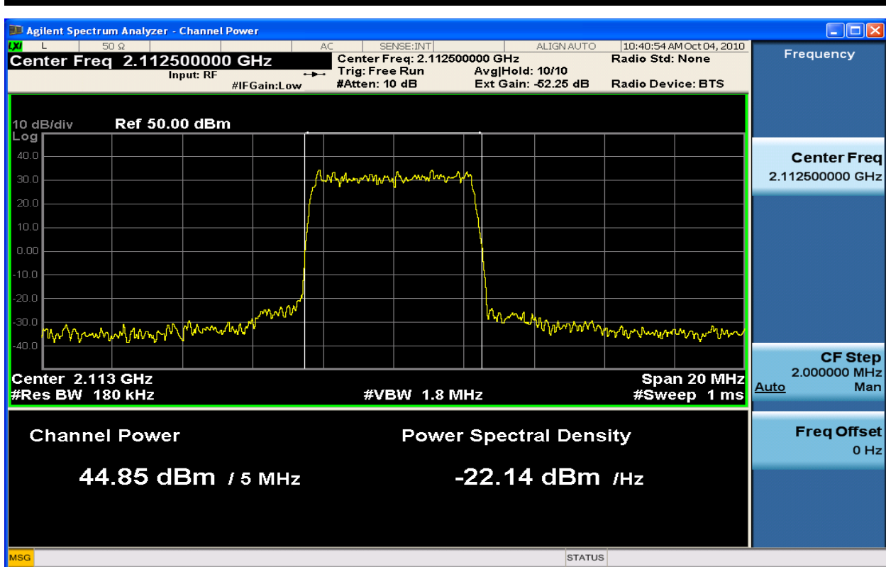
Figure 6-4: 5MHz BW Channel Power TX1_16QAM at 2112.5 MHz
