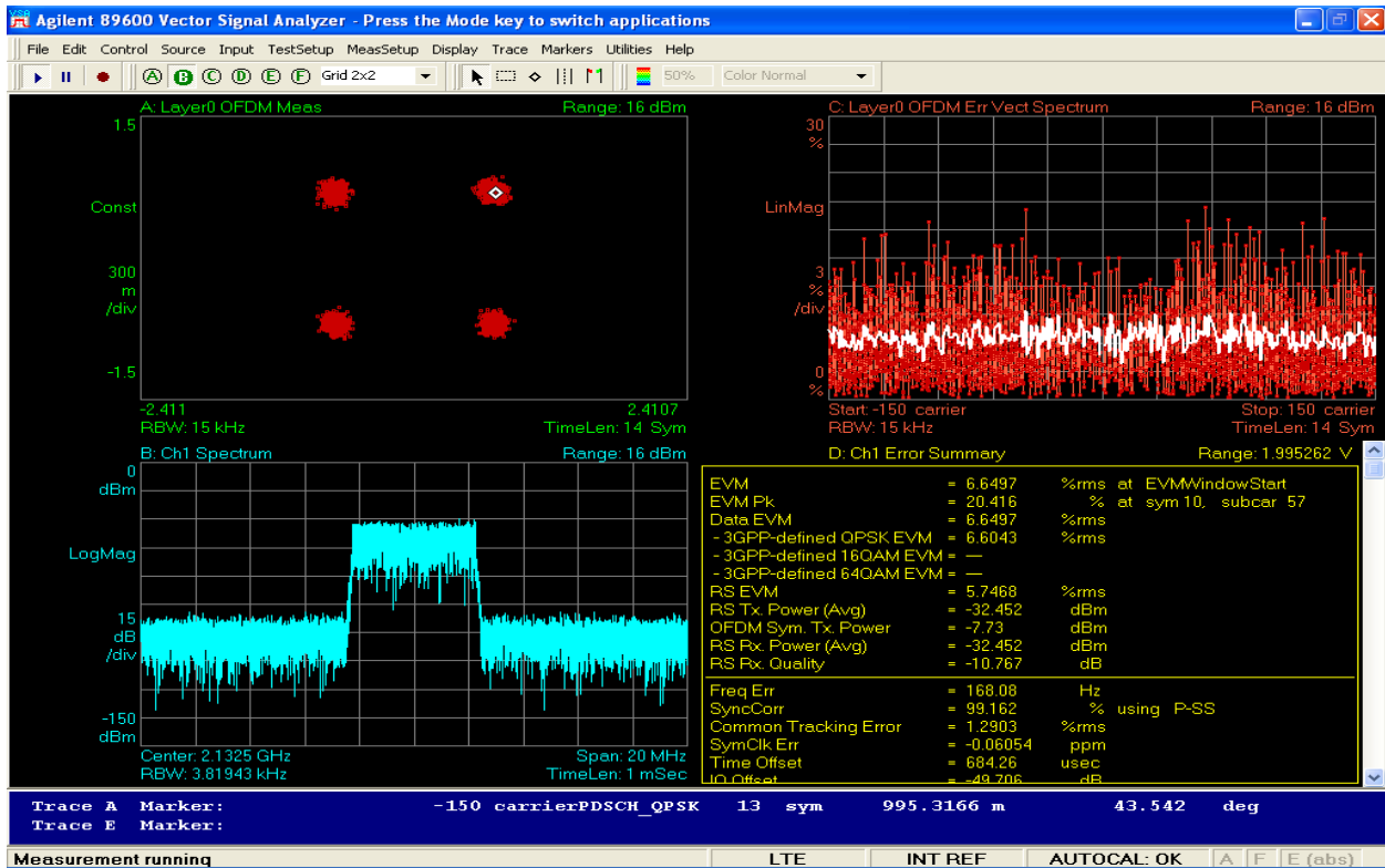
Figure 6-10: 5MHz BW Modulation TX2_QPSK at 2132.5MHz
