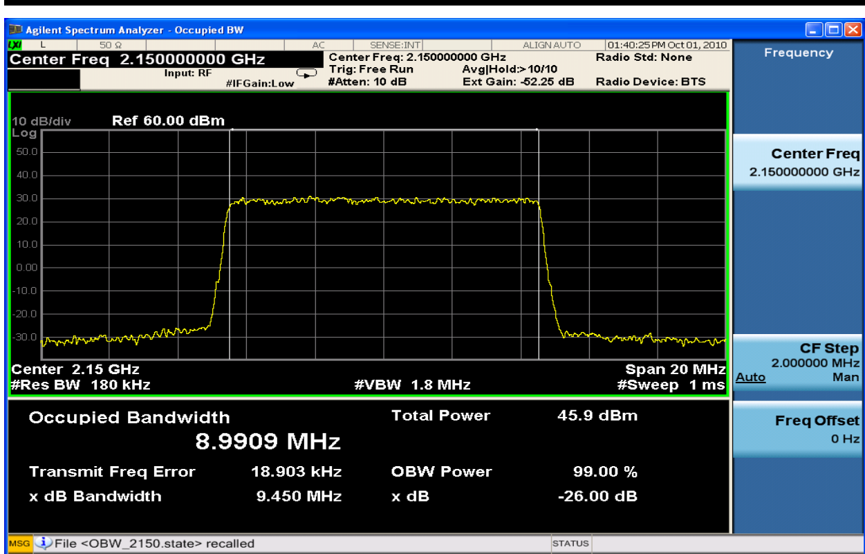
Figure 6-83: 10MHz Occupied Bandwidth TX1_16QAM at 2150.0 MHz
