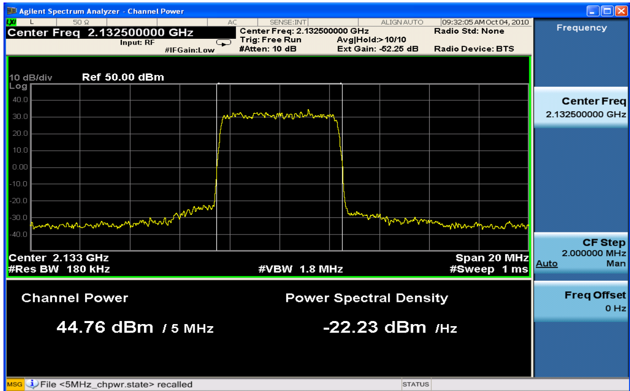
Figure 6-13 : 5MHz BW Channel Power TX1_16QAM at 2132.5 MHz
