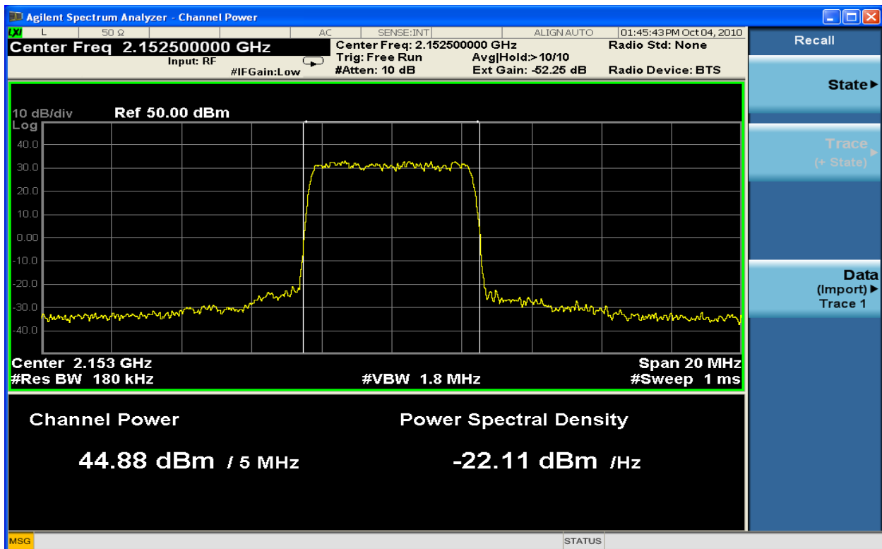
Figure 6-23 : 5MHz BW Channel Power TX2_16QAM at 2152.5 MHz
