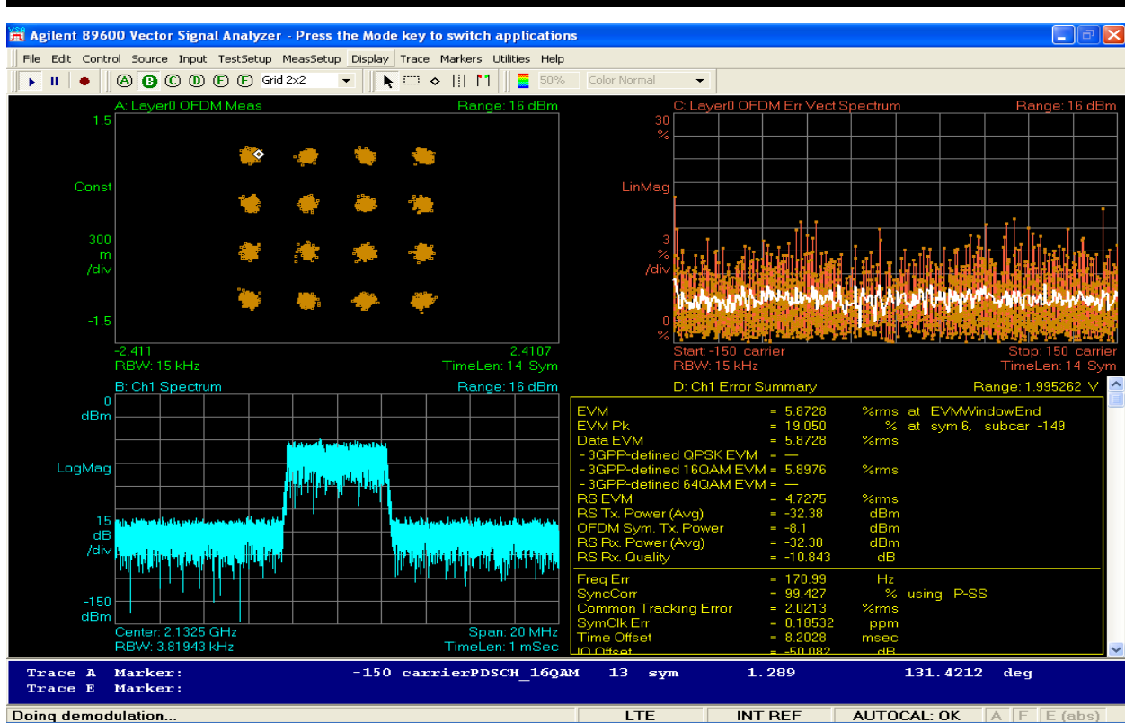
Figure 6-14: 5MHz BW Modulation TX2_16QAM at 2132.5MHz
