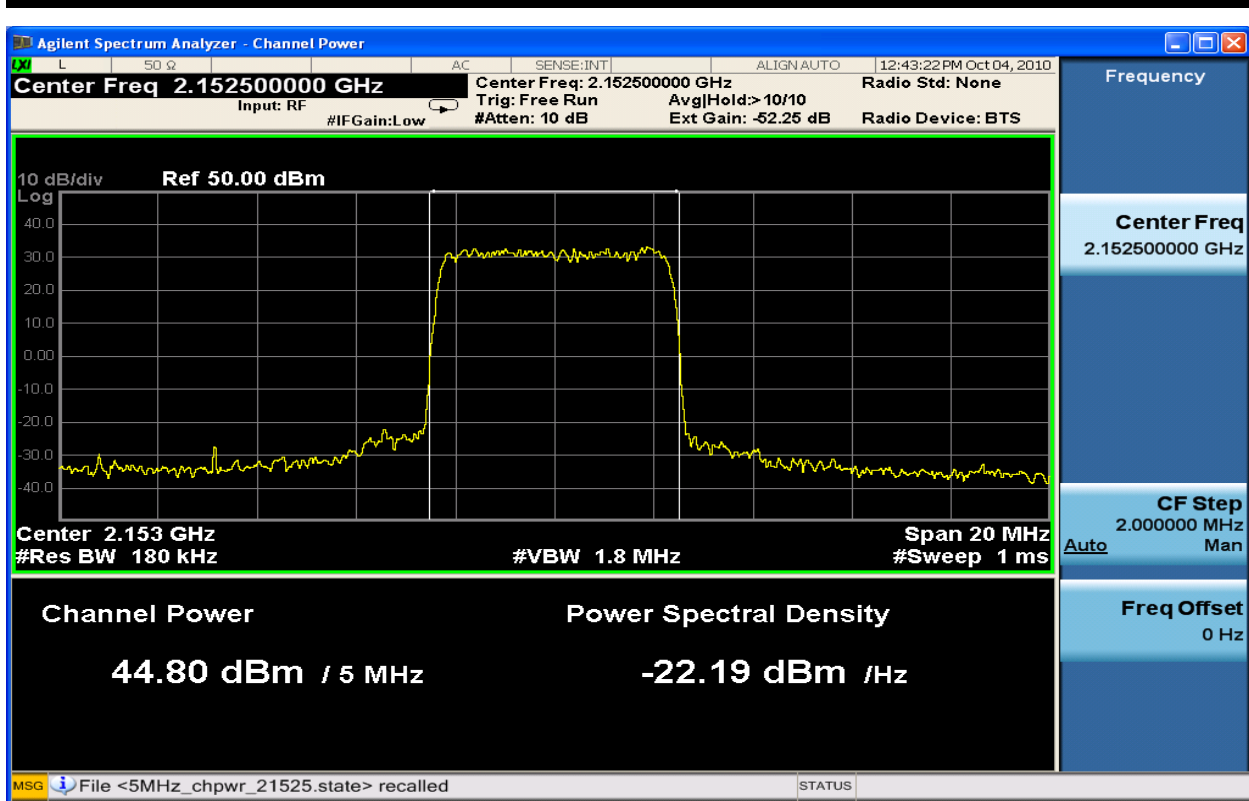
Figure 6-22 : 5MHz BW Channel Power TX1_16QAM at 2152.5 MHz
