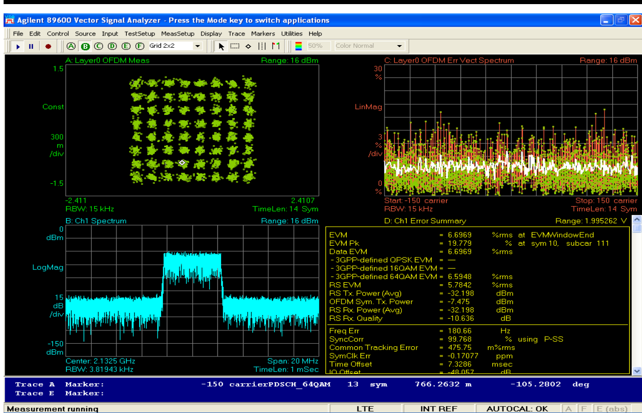
Figure 6-16: 5MHz BW Modulation TX1_64QAM at 2132.5MHz
