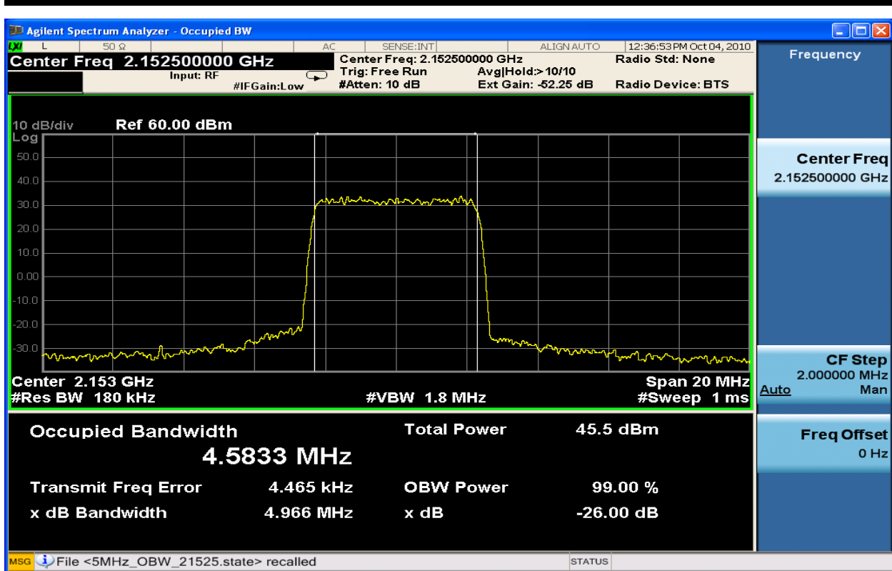
Figure 6-63: 5MHz Occupied Bandwidth TX1_QPSK at 2152.5 MHz
