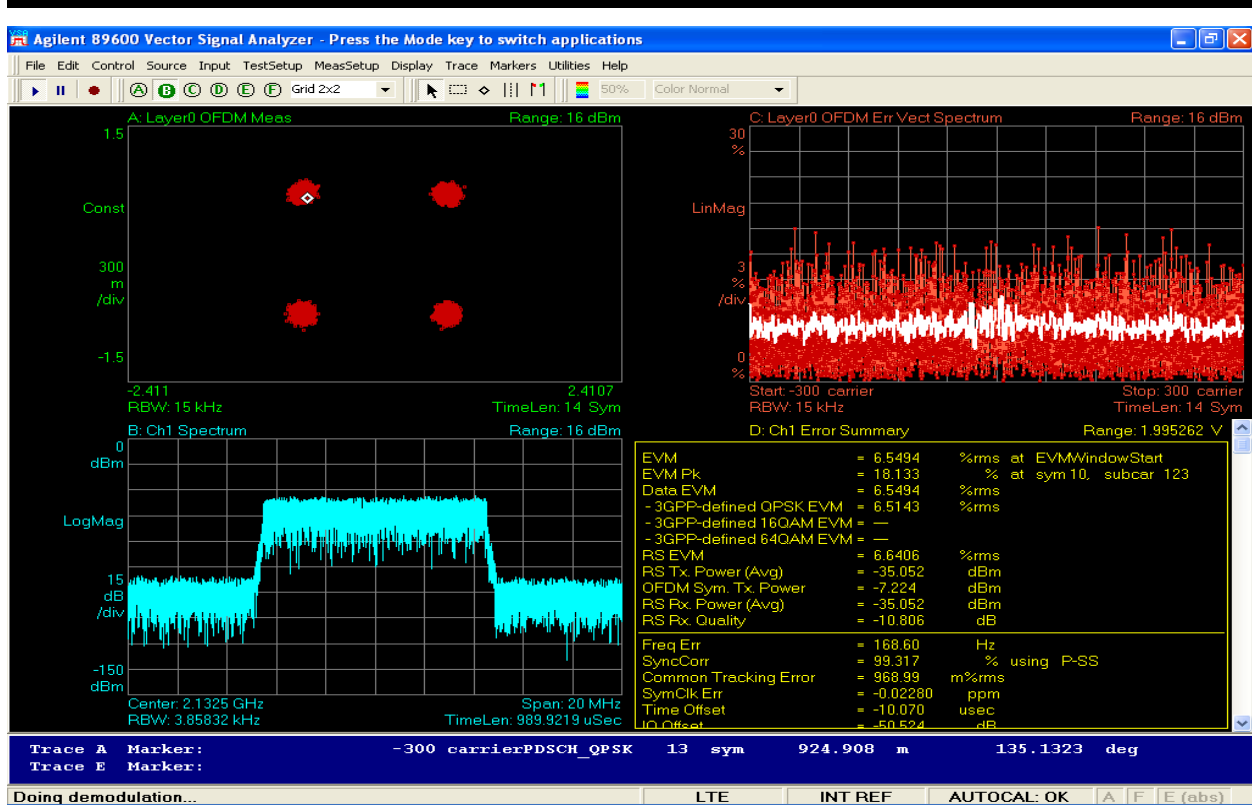
Figure 6-32 : 10MHz BW Modulation TX1_QPSK at 2132.5 MHz
