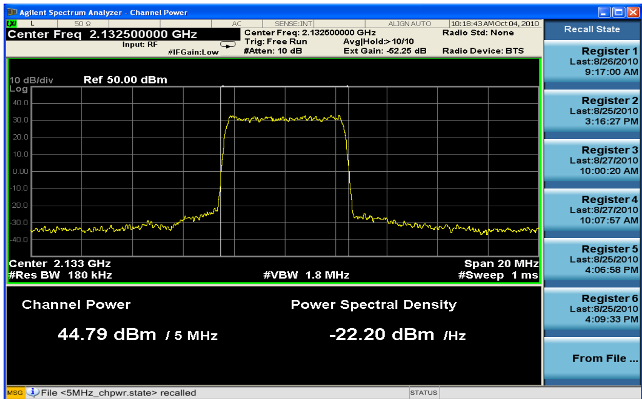
Figure 6-19 : 5MHz BW Channel Power TX2_64QAM at 2132.5 MHz
