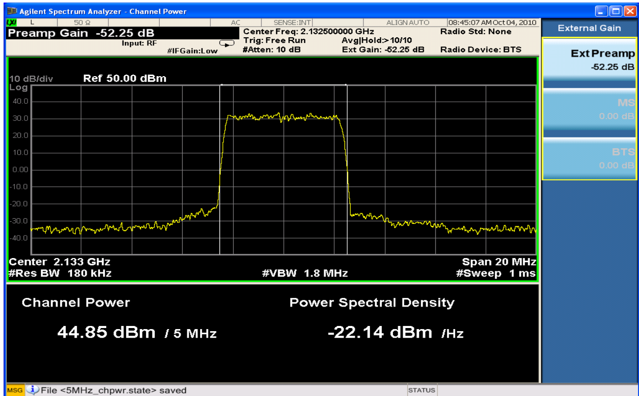
Figure 6-17 : 5MHz BW Channel Power TX1_64QAM at 2132.5 MHz
