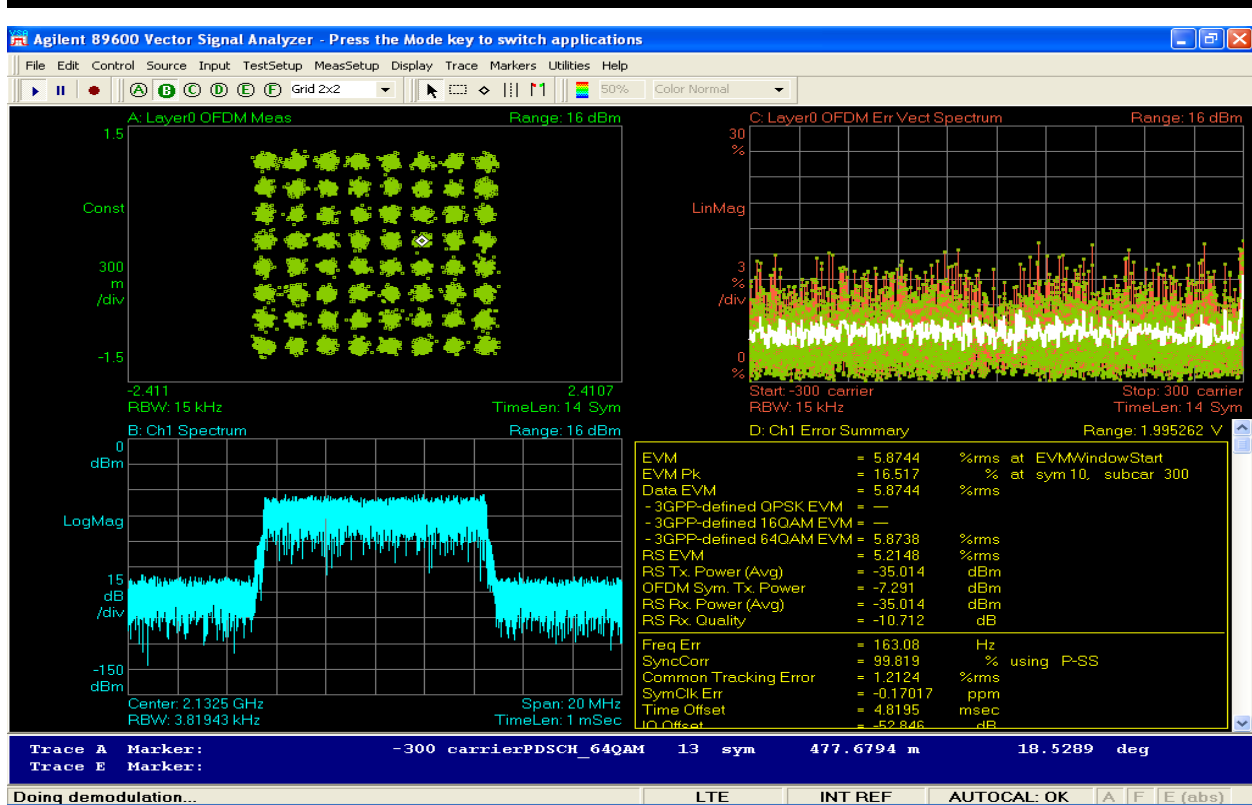
Figure 6-42 : 10MHz BW Modulation TX2_64QAM at 2132.5MHz
