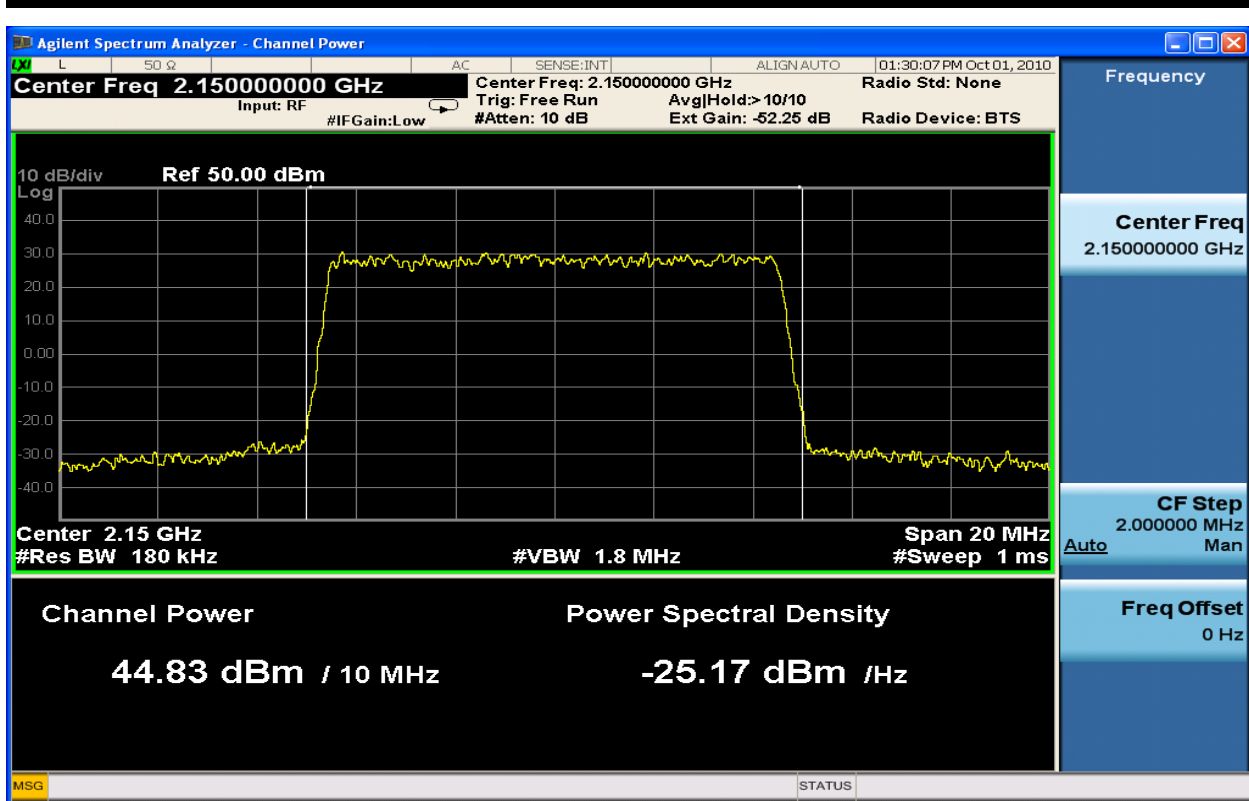
Figure 6-44 : 10MHz BW Channel Power TX1_QPSK at 2150.0 MHz
