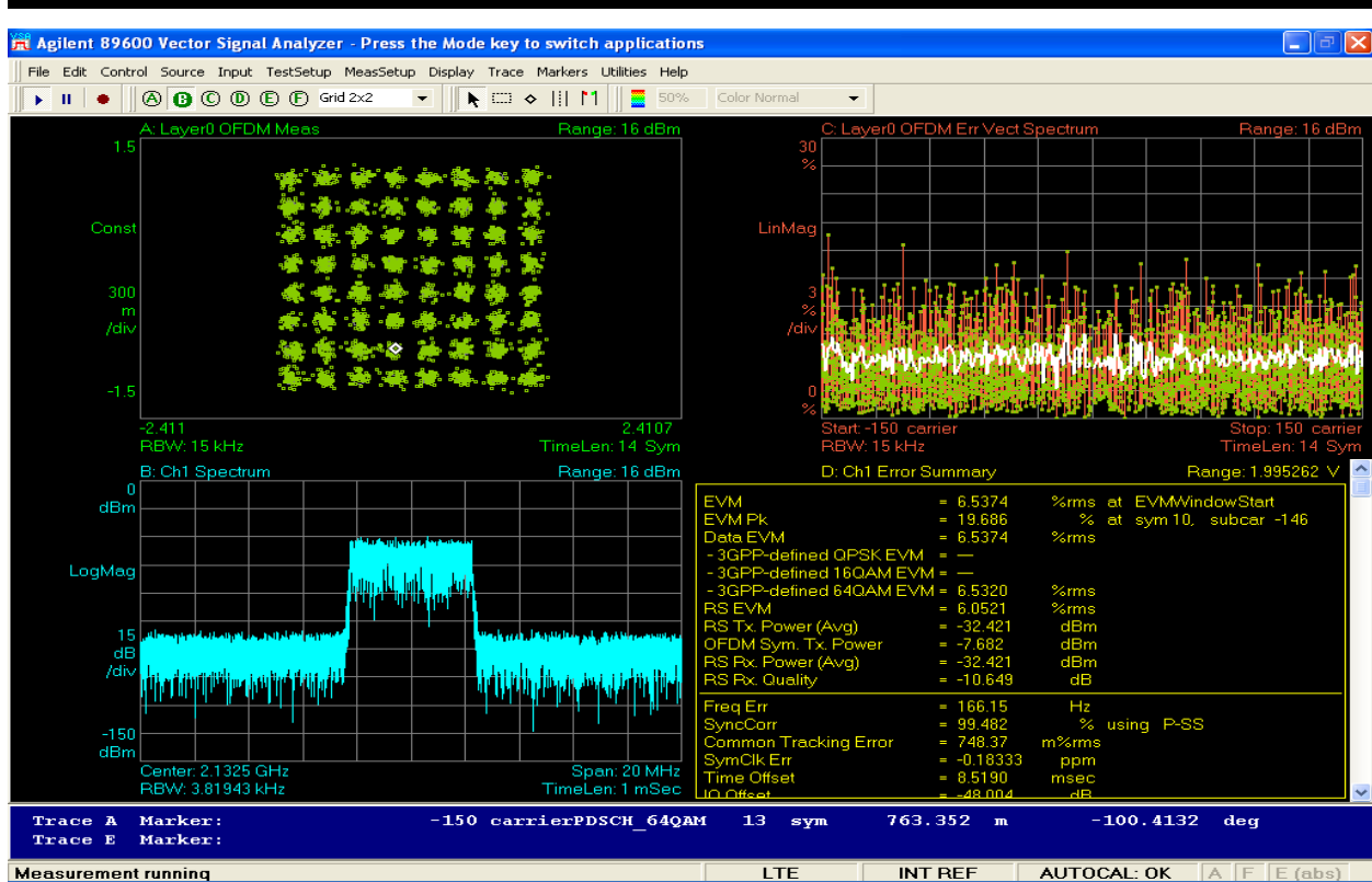
Figure 6-18: 5MHz BW Modulation TX2_64QAM at 2132.5MHz
