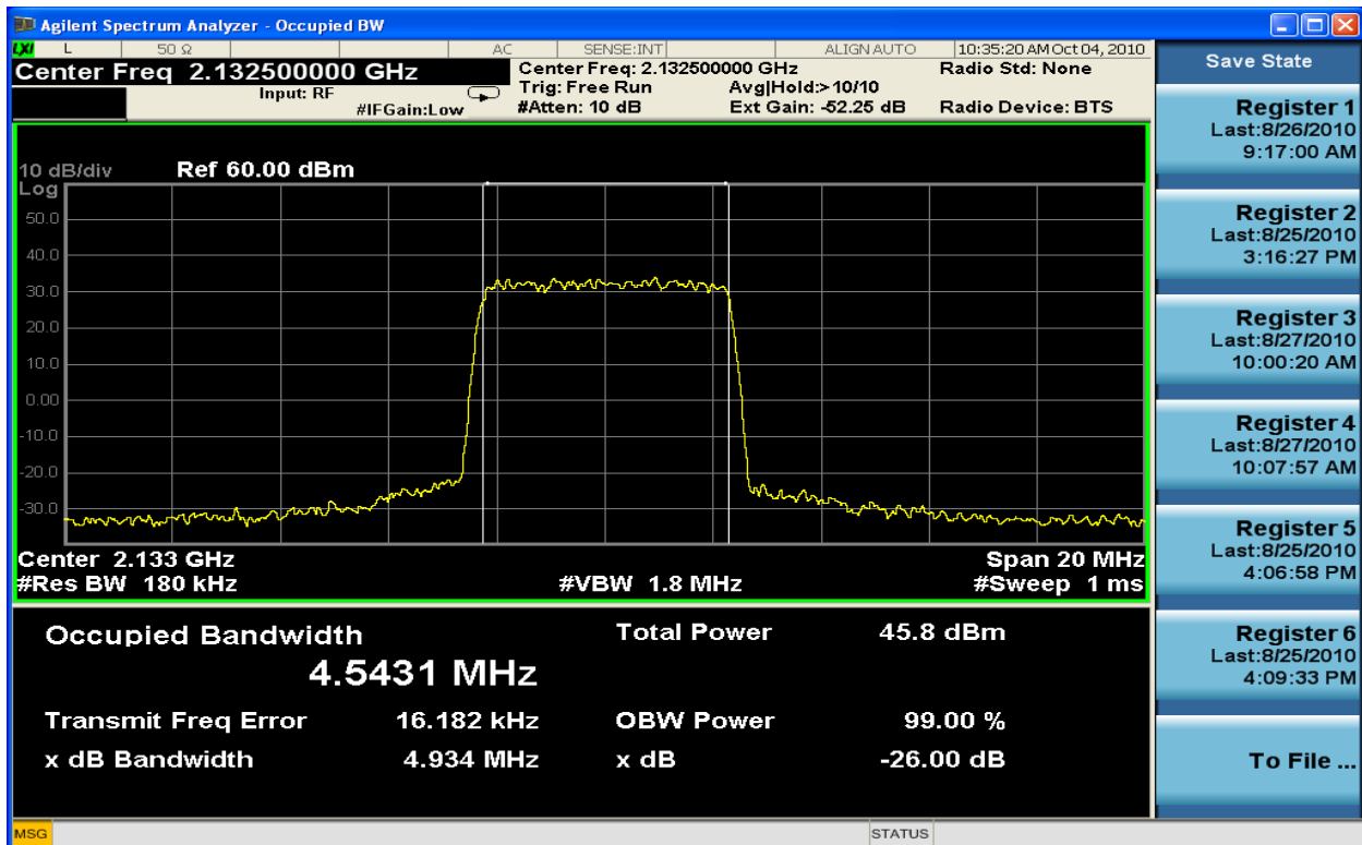
Figure 6-58: 5MHz Occupied Bandwidth TX2_QPSK at 2132.5 MHz
