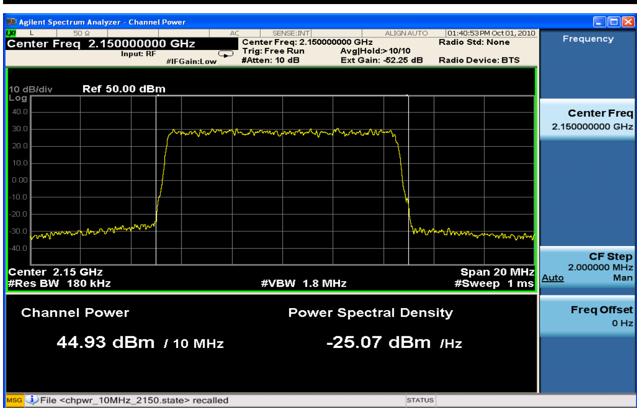
Figure 6-46 : 10MHz BW Channel Power TX1_16QAM at 2150.0 MHz
