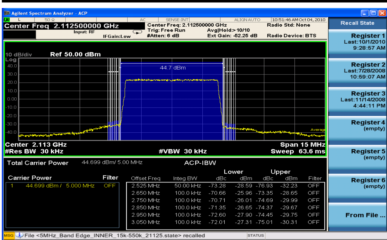
Figure 6-88 Spurious Emissions 2112.5MHz TX1_QPSK 5MHz Band Edge (ACP 15kHz – 550kHz)
