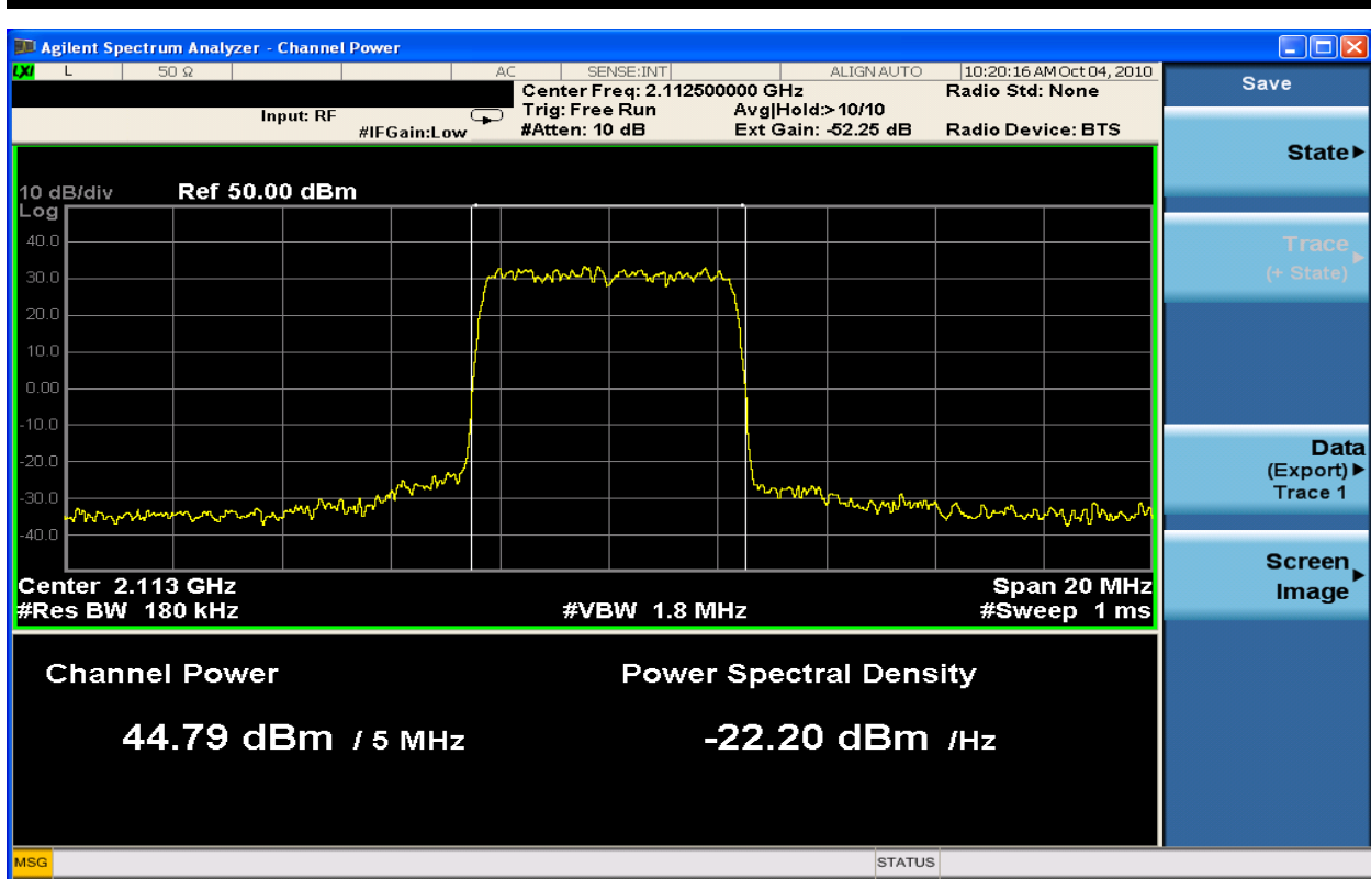
Figure 6-6: 5MHz BW Channel Power TX1_64QAM at 2112.5 MHz
