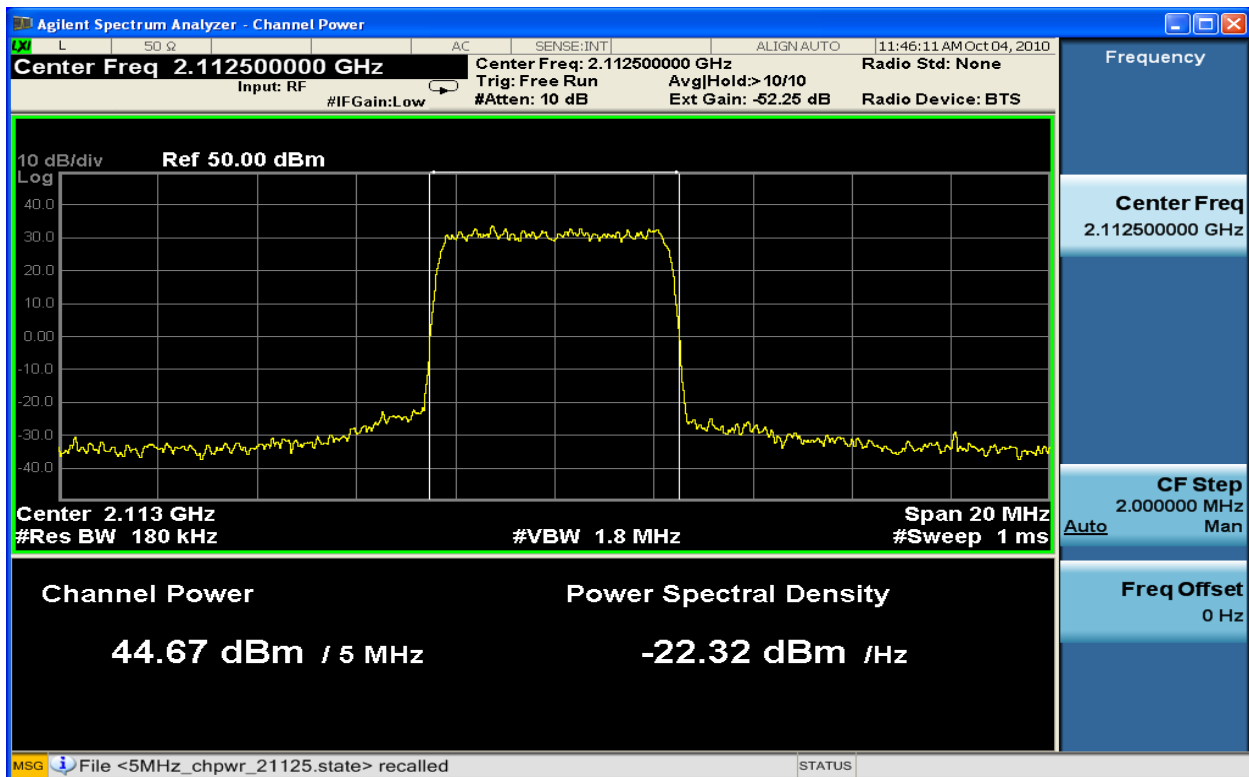
Figure 6-5: 5MHz BW Channel Power TX2_16QAM at 2112.5 MHz
