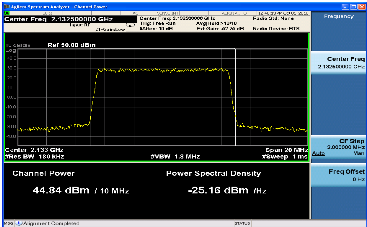
Figure 6-33 : 10MHz BW Channel Power TX1_QPSK at 2132.5 MHz
