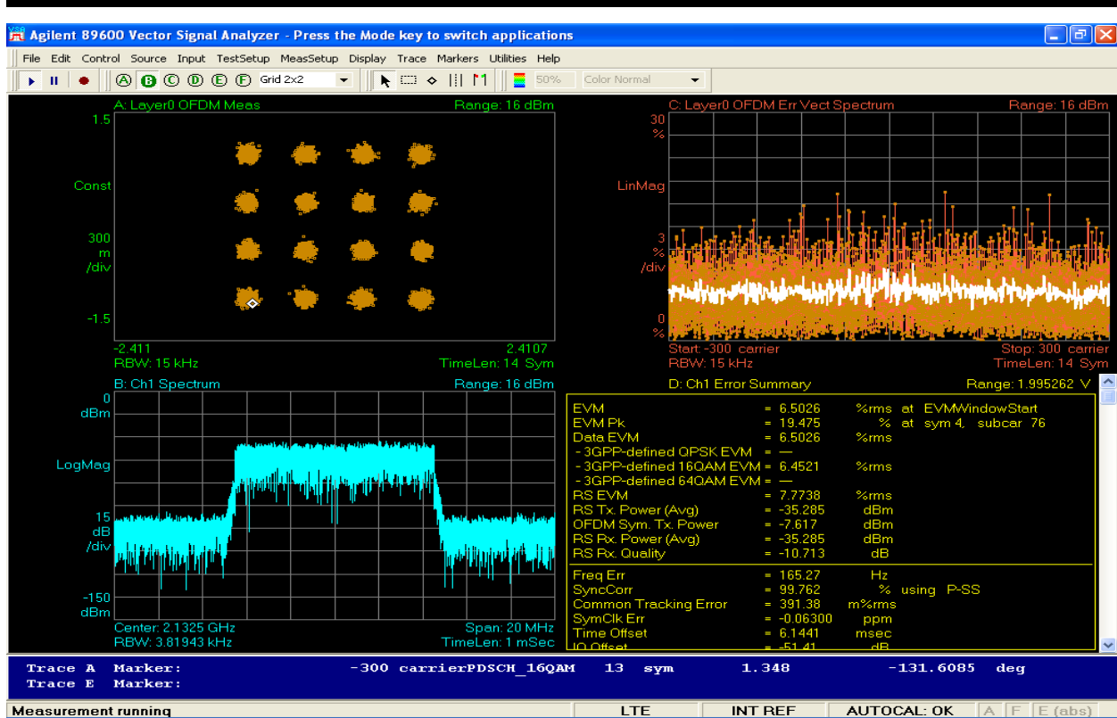
Figure 6-38 : 10MHz BW Modulation TX2_16QAM at 2132.5MHz
