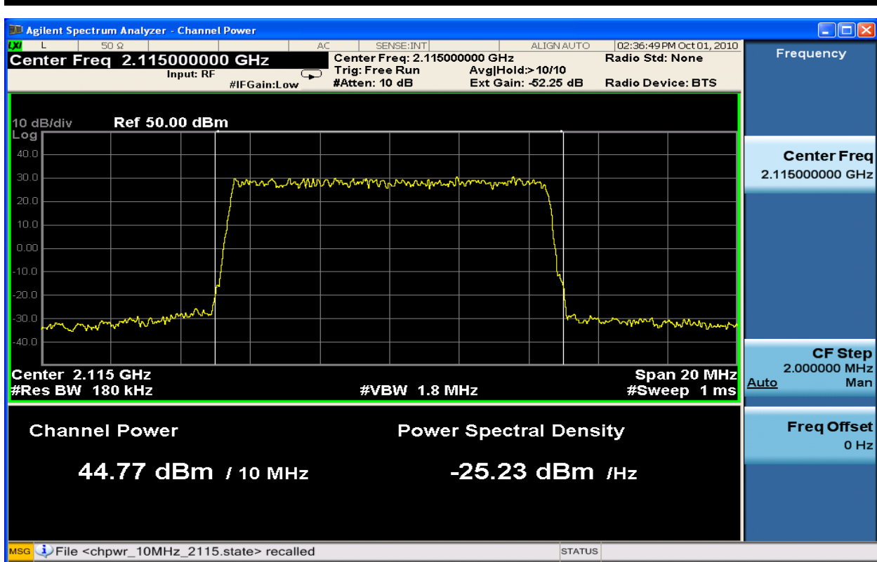
Figure 6-26 : 10MHz BW Channel Power TX1_QPSK at 2115.0 MHz
