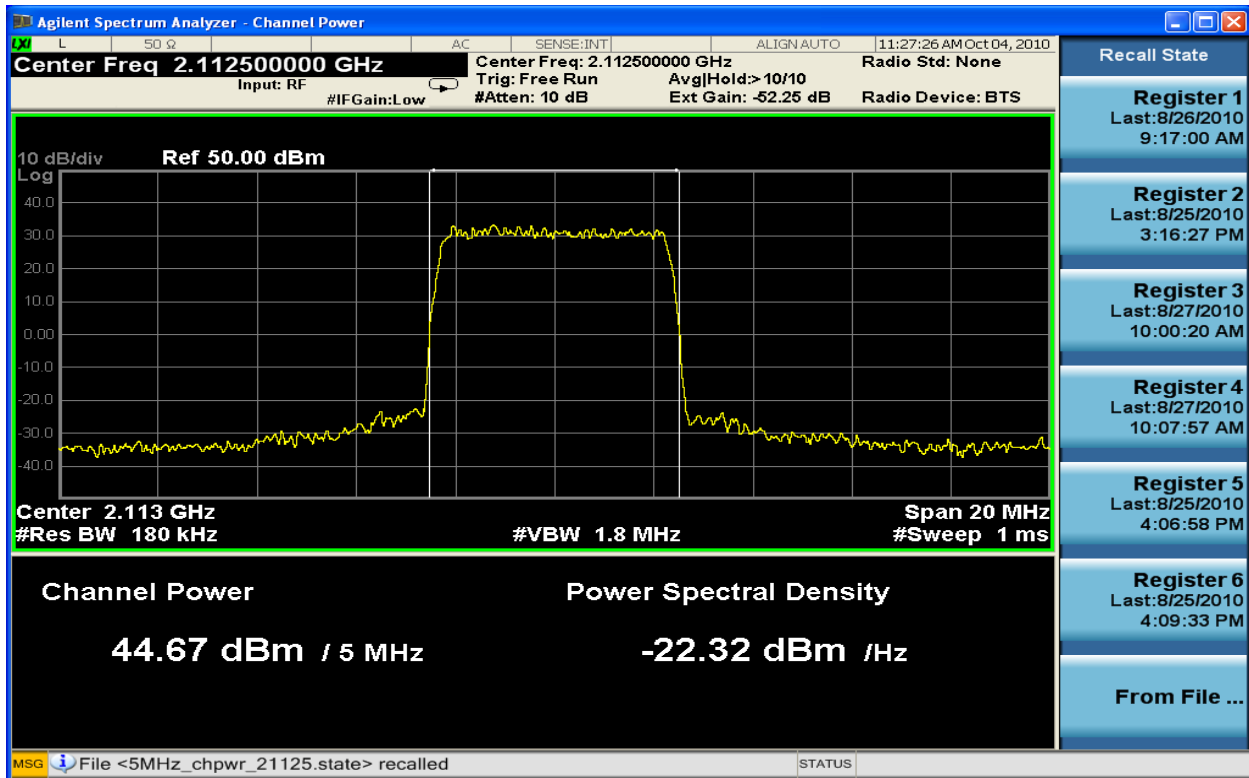
Figure 6-7: 5MHz BW Channel Power TX2_64QAM at 2112.5 MHz
