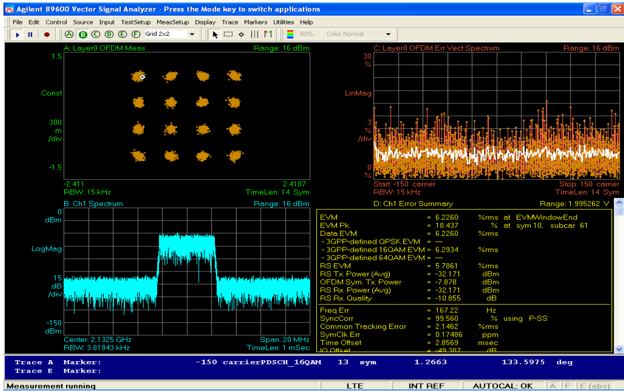
Figure 6-12: 5MHz BW Modulation TX1_16QAM at 2132.5MHz
