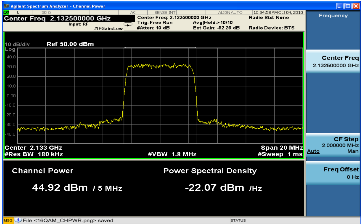
Figure 6-11 : 5MHz BW Channel Power TX2_QPSK at 2132.5 MHz
