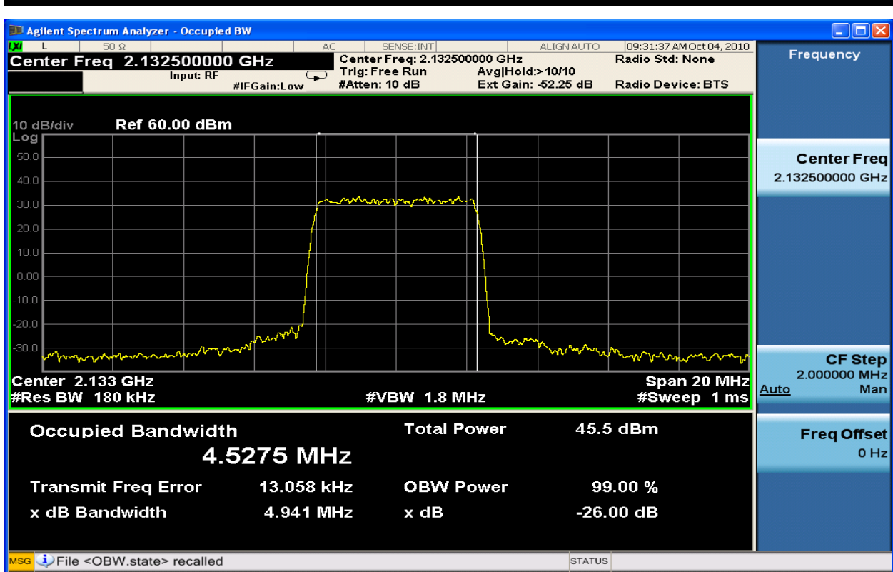
Figure 6-59: 5MHz Occupied Bandwidth TX1_16QAM at 2132.5 MHz
