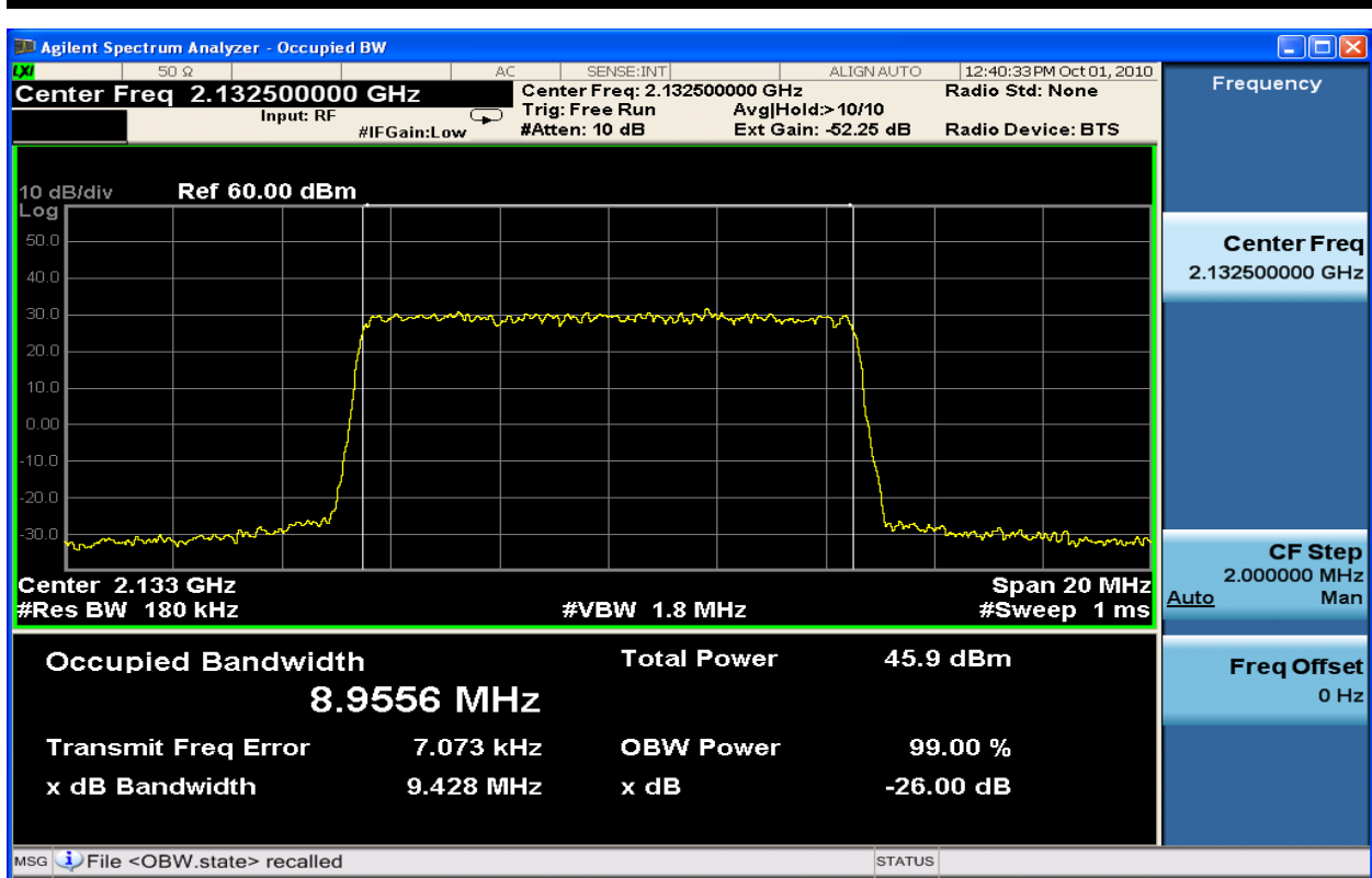
Figure 6-75: 10MHz Occupied Bandwidth TX1_QPSK at 2132.5 MHz
