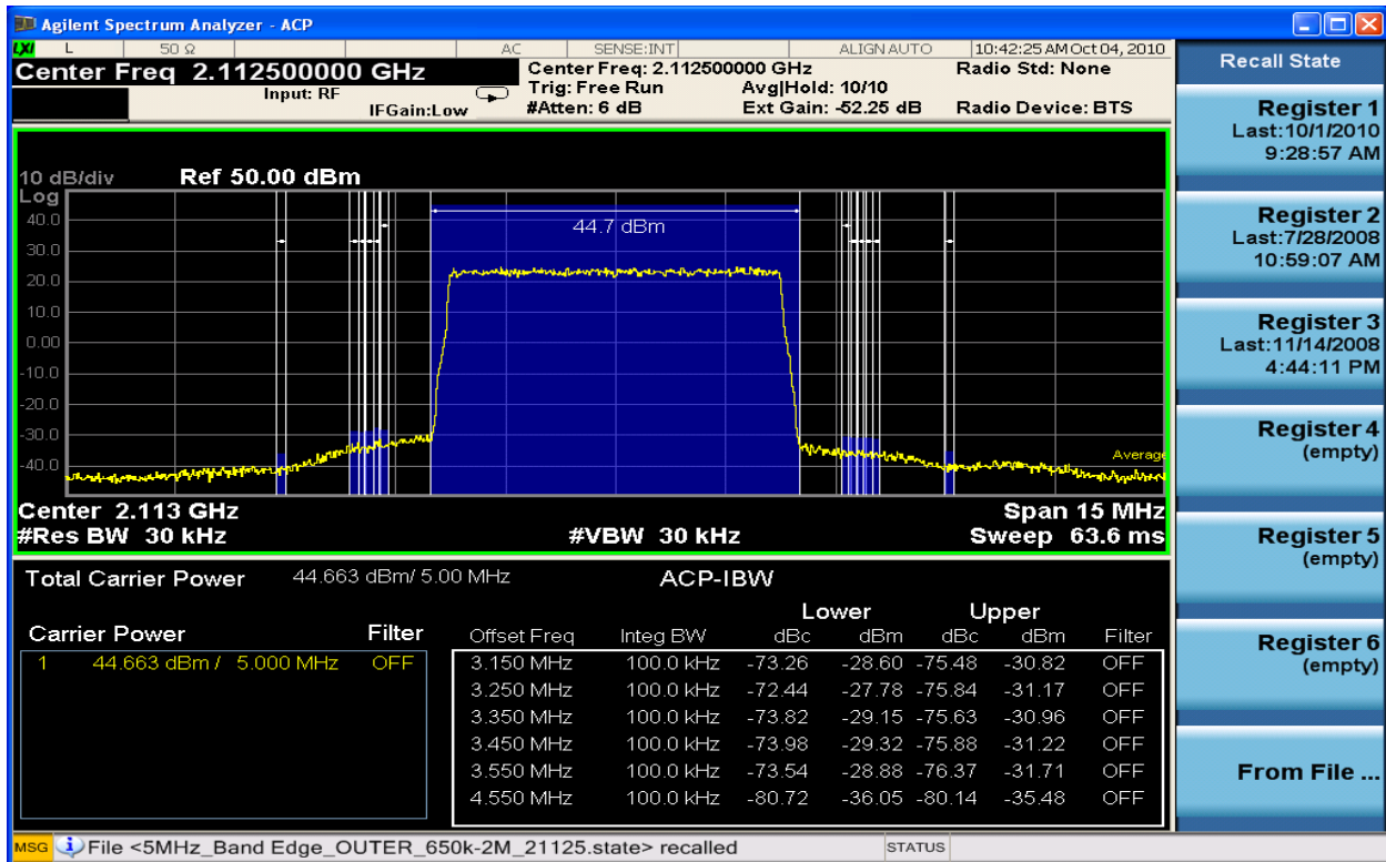
Figure 6-93 Spurious Emissions 2112.5MHz TX1_16QAM 5MHz Band Edge (ACP 650kHz – 2MHz)
