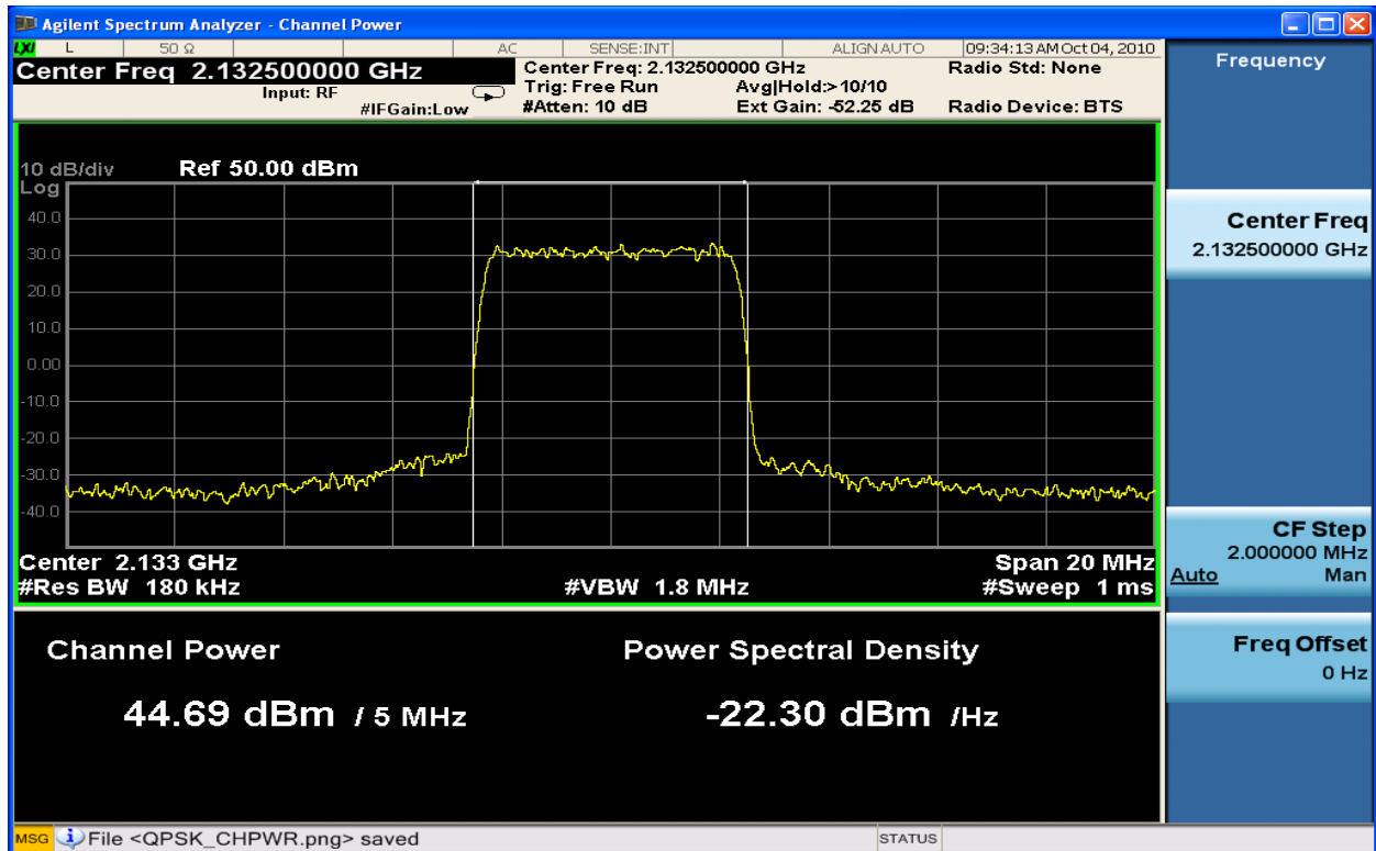
Figure 6-9 : 5MHz BW Channel Power TX1_QPSK at 2132.5 MHz
