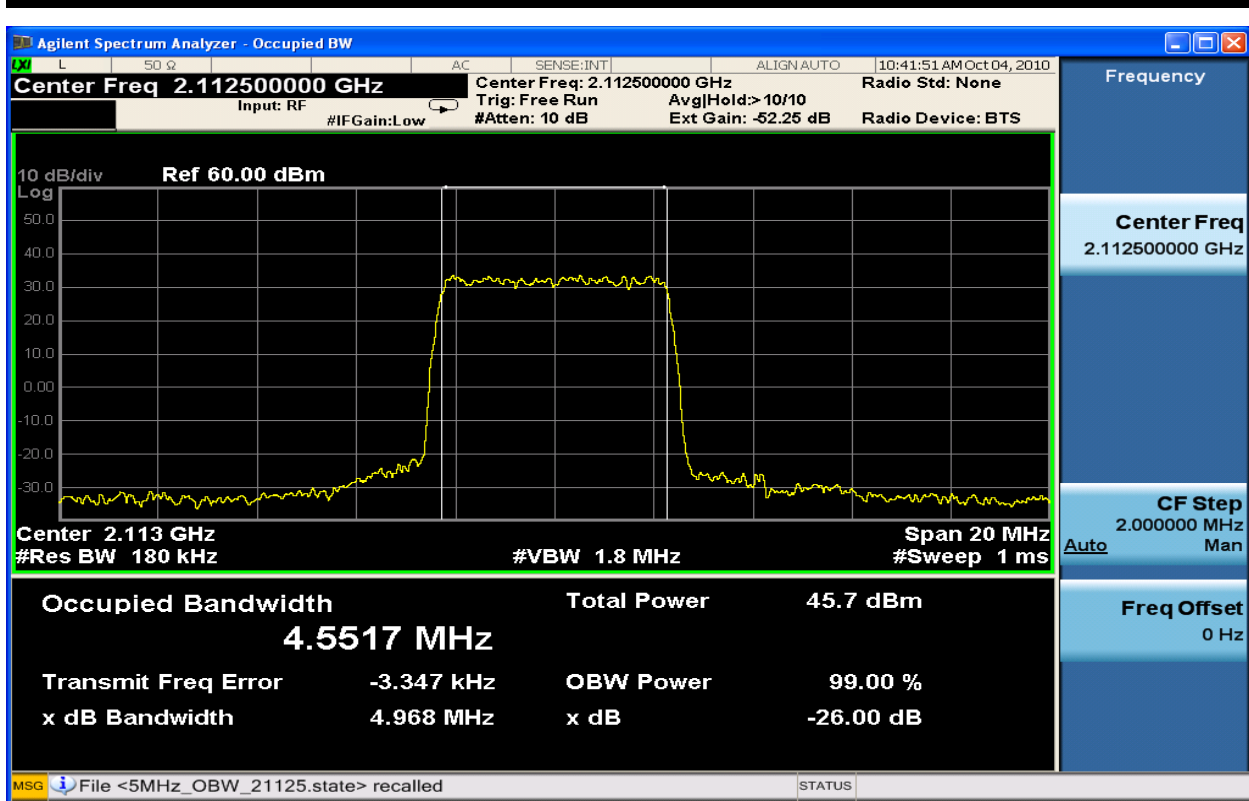
Figure 6-53: 5MHz Occupied Bandwidth TX1_16QAM at 2112.5 MHz
