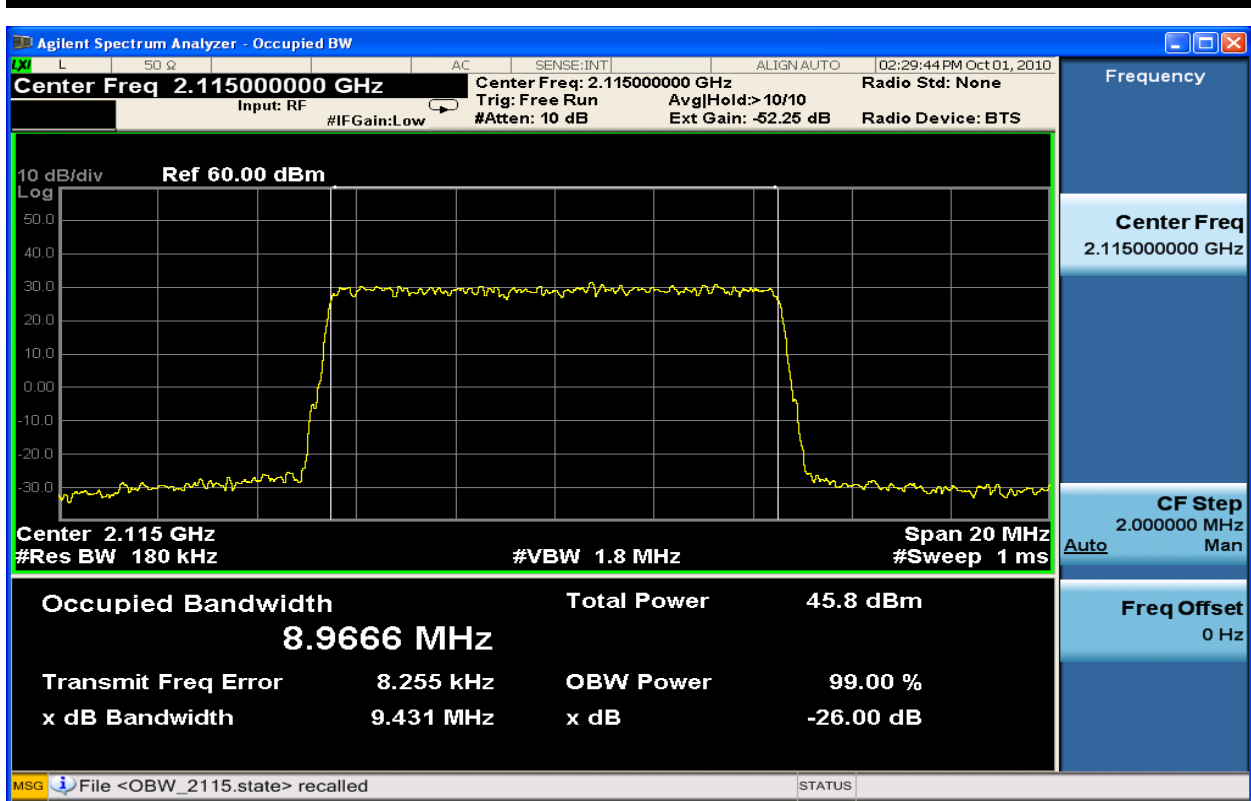
Figure 6-71: 10MHz Occupied Bandwidth TX1_16QAM at 2115.0 MHz
