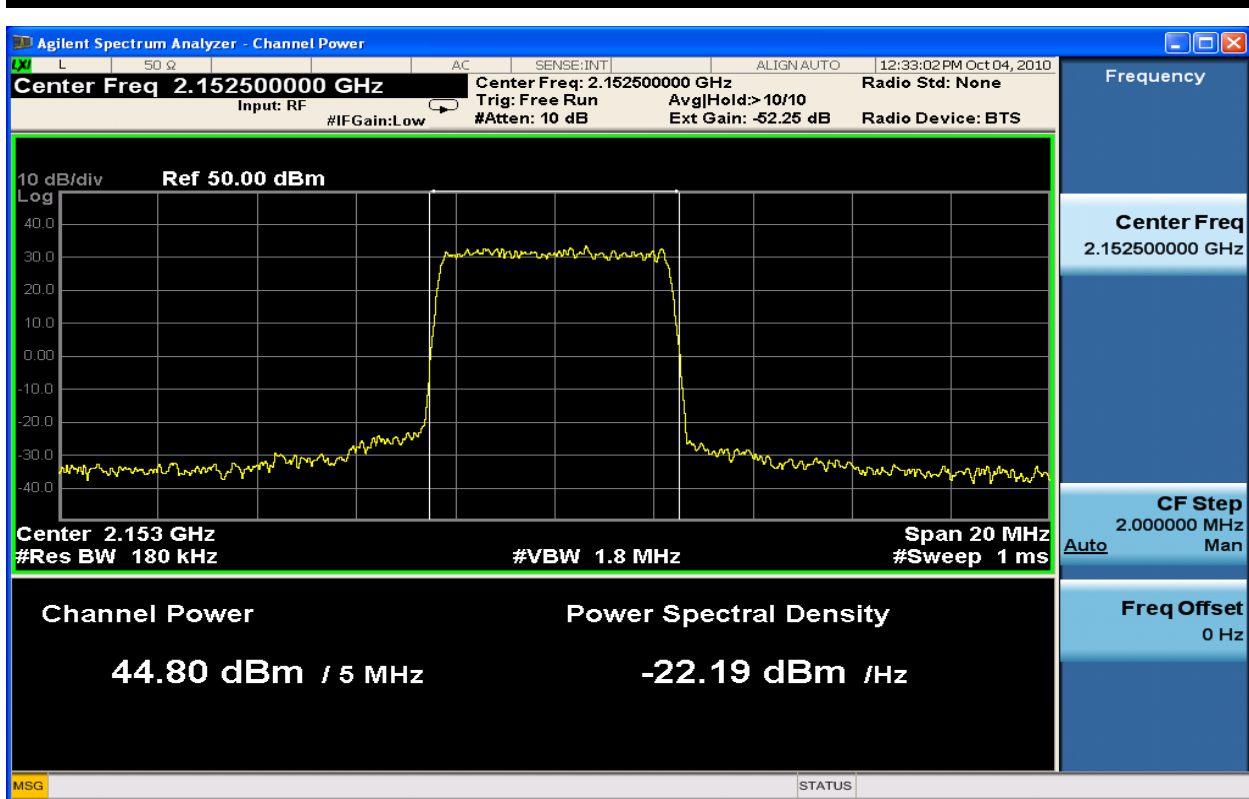
Figure 6-20 : 5MHz BW Channel Power TX1_QPSK at 2152.5 MHz
