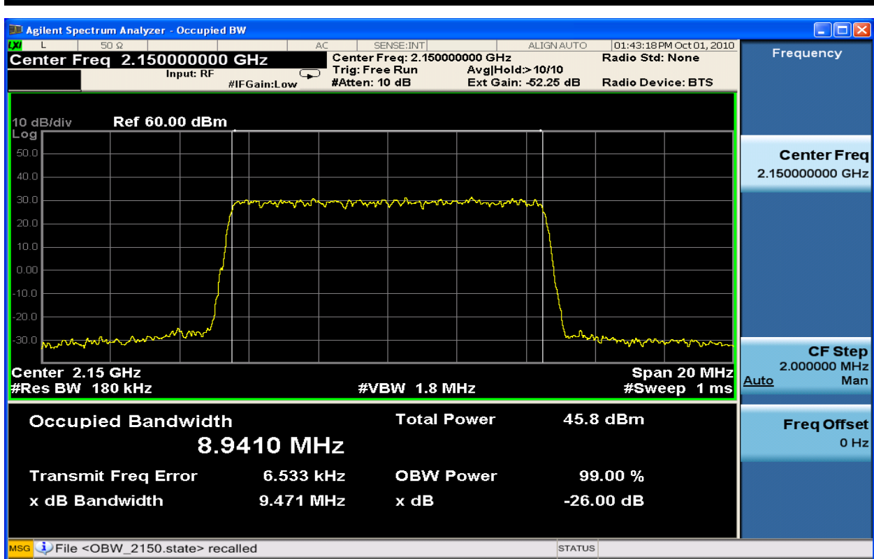
Figure 6-85: 10MHz Occupied Bandwidth TX1_64QAM at 2150.0 MHz
