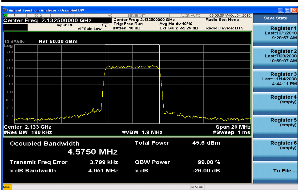
Figure 6-61: 5MHz Occupied Bandwidth TX1_64QAM at 2132.5 MHz
