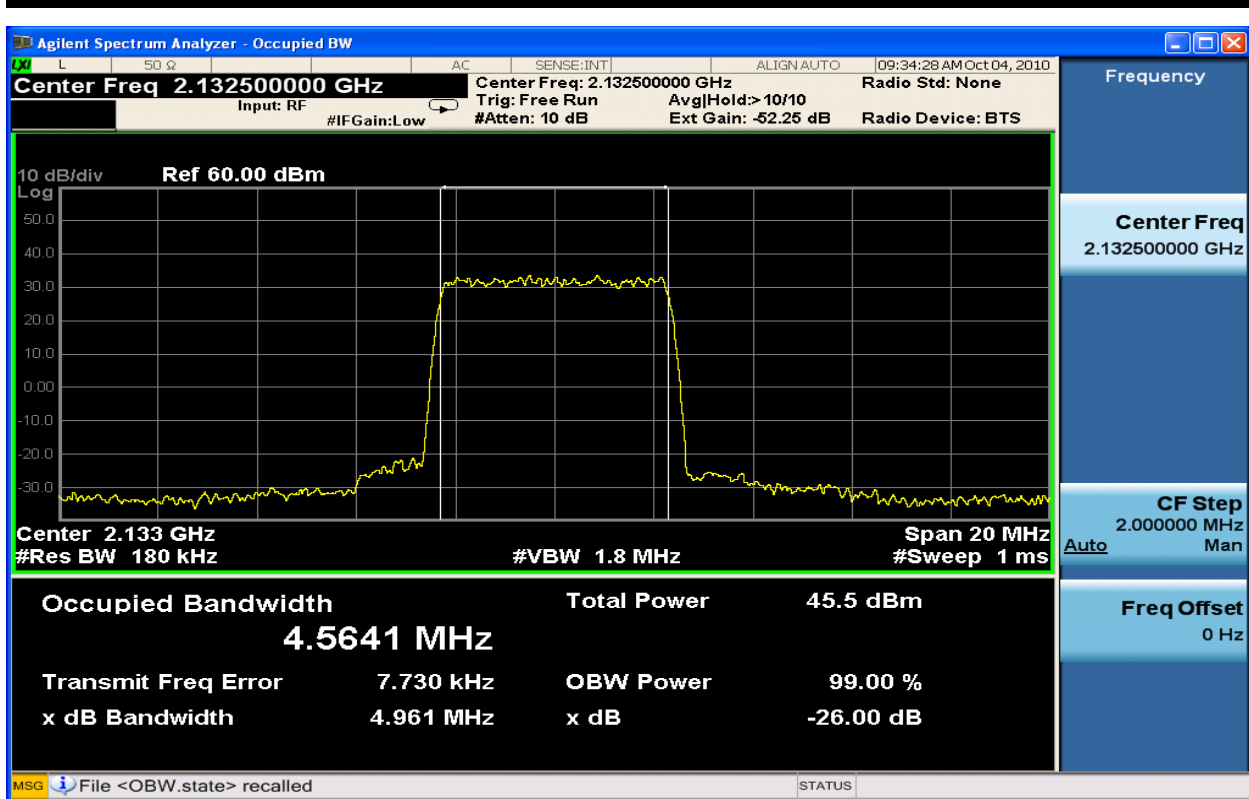
Figure 6-57: 5MHz Occupied Bandwidth TX1_QPSK at 2132.5 MHz
