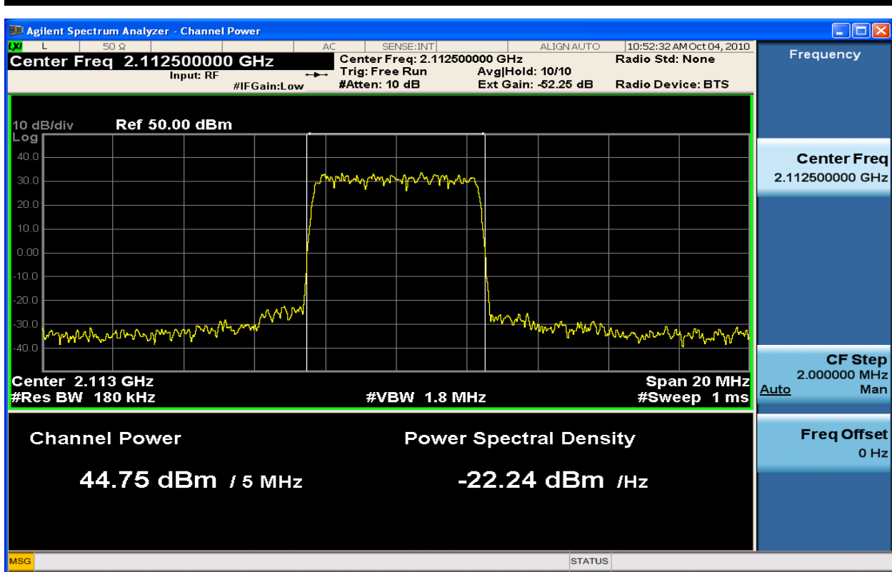
Figure 6-2: 5MHz BW Channel Power TX1_QPSK at 2112.5 MHz
