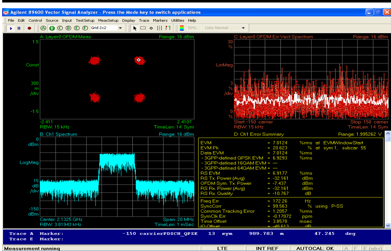
Figure 6-8: 5MHz BW Modulation TX1_QPSK at 2132.5MHz
