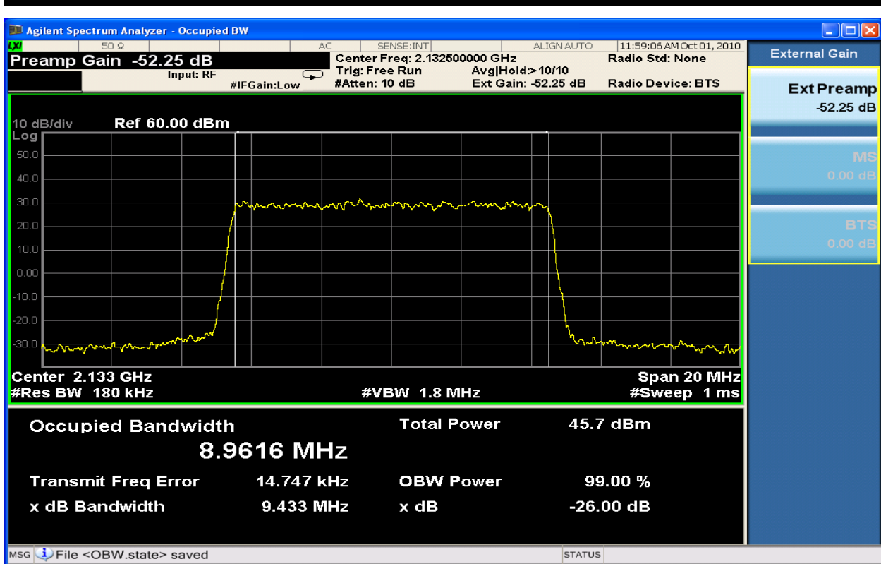
Figure 6-79: 10MHz Occupied Bandwidth TX1_64QAM at 2132.5 MHz
