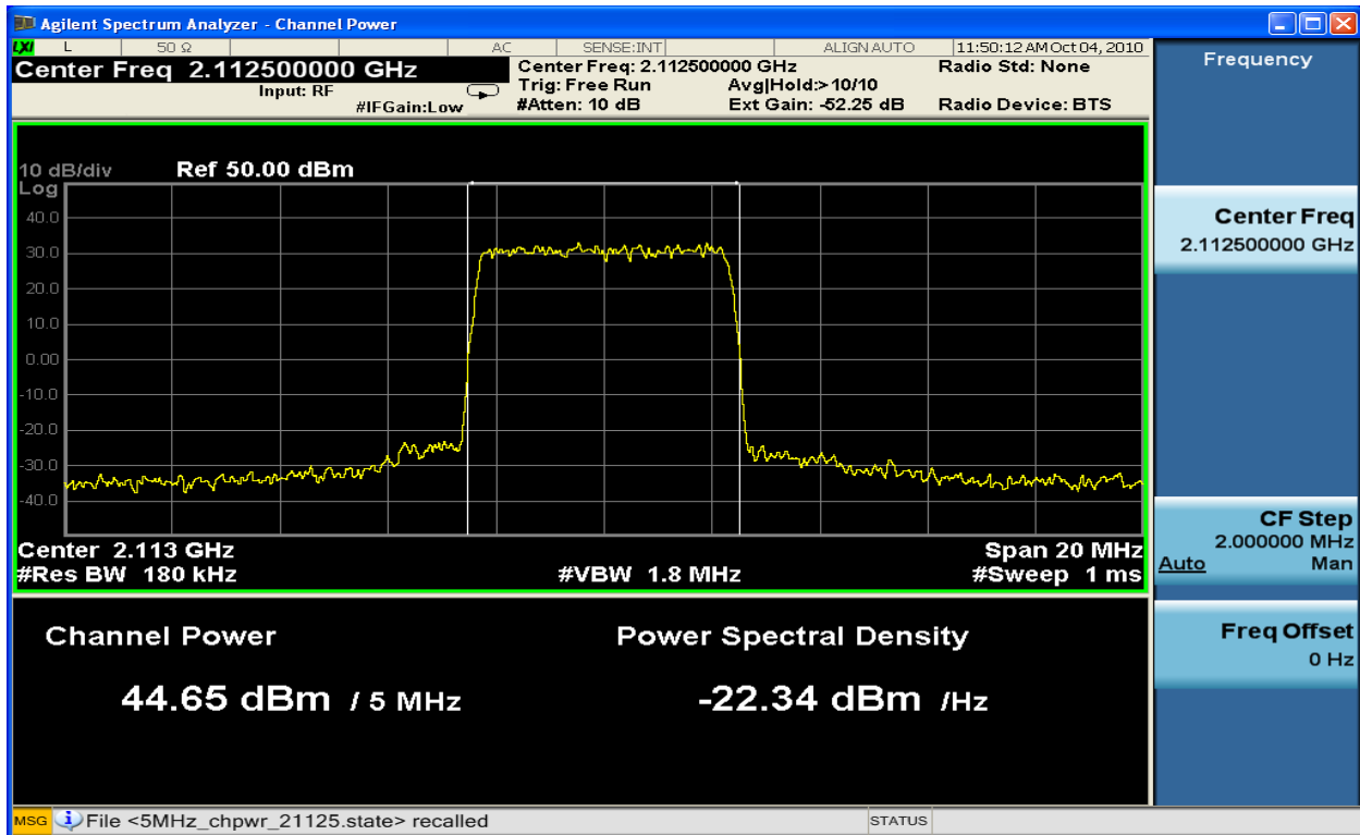
Figure 6-3: 5MHz BW Channel Power TX2_QPSK at 2112.5 MHz
