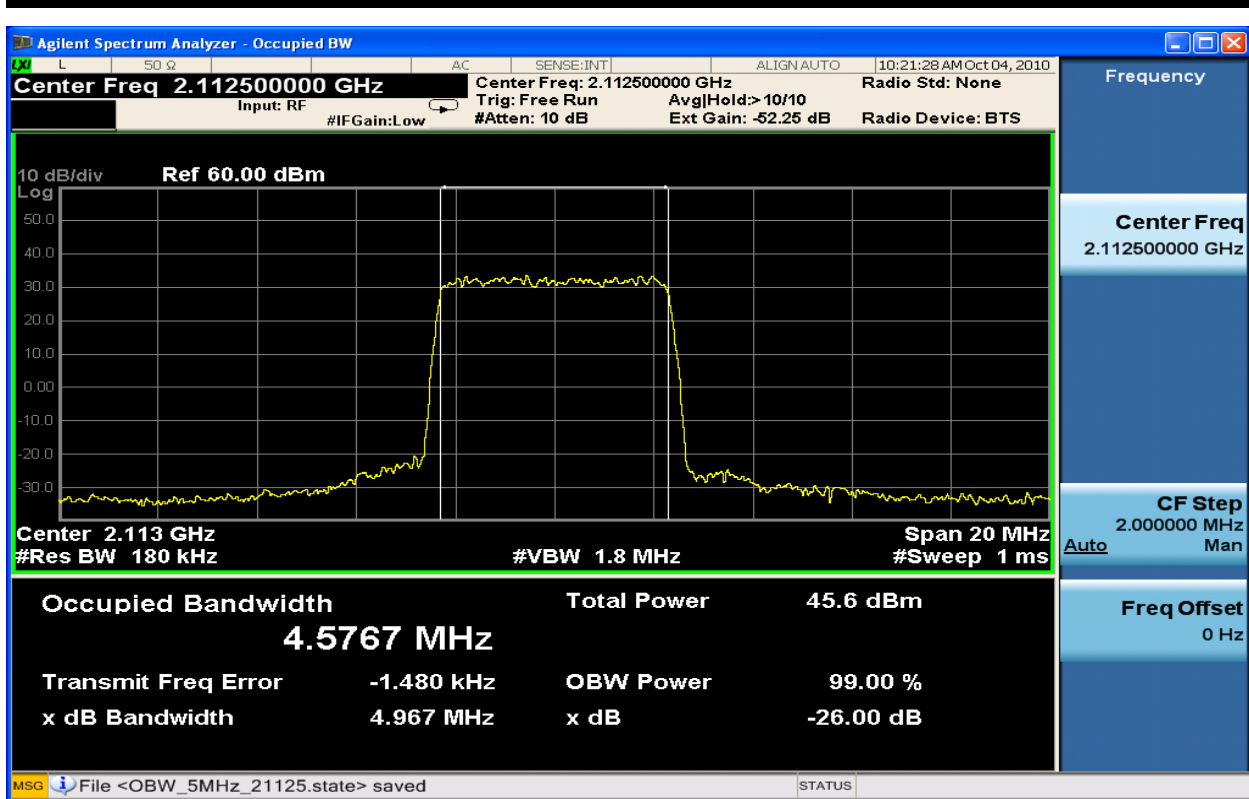
Figure 6-55: 5MHz Occupied Bandwidth TX1_64QAM at 2112.5 MHz
