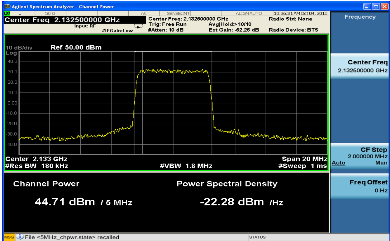
Figure 6-15 : 5MHz BW Channel Power TX2_16QAM at 2132.5 MHz
