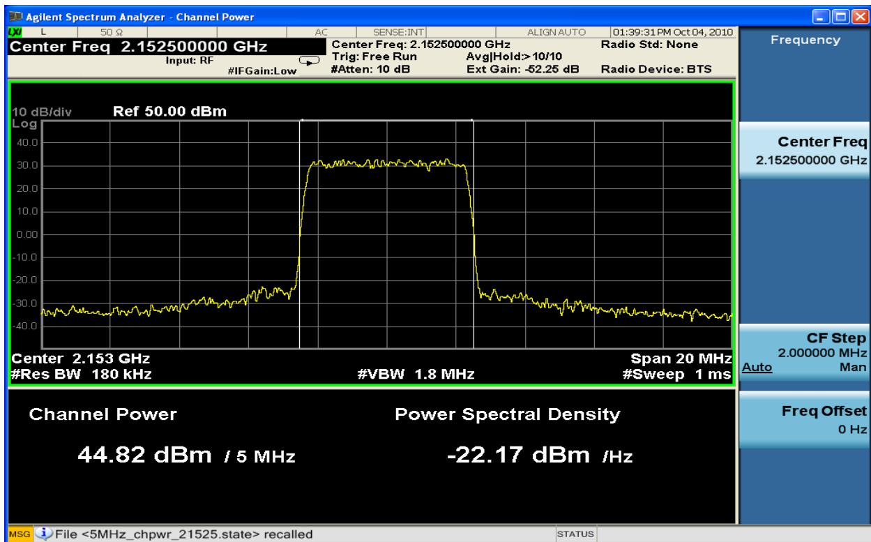
Figure 6-21 : 5MHz BW Channel Power TX2_QPSK at 2152.5 MHz
