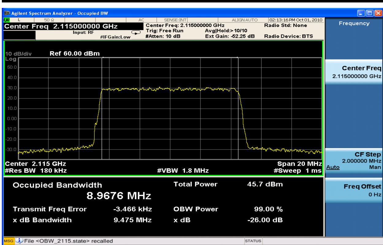
Figure 6-73: 10MHz Occupied Bandwidth TX1_64QAM at 2115.0 MHz
