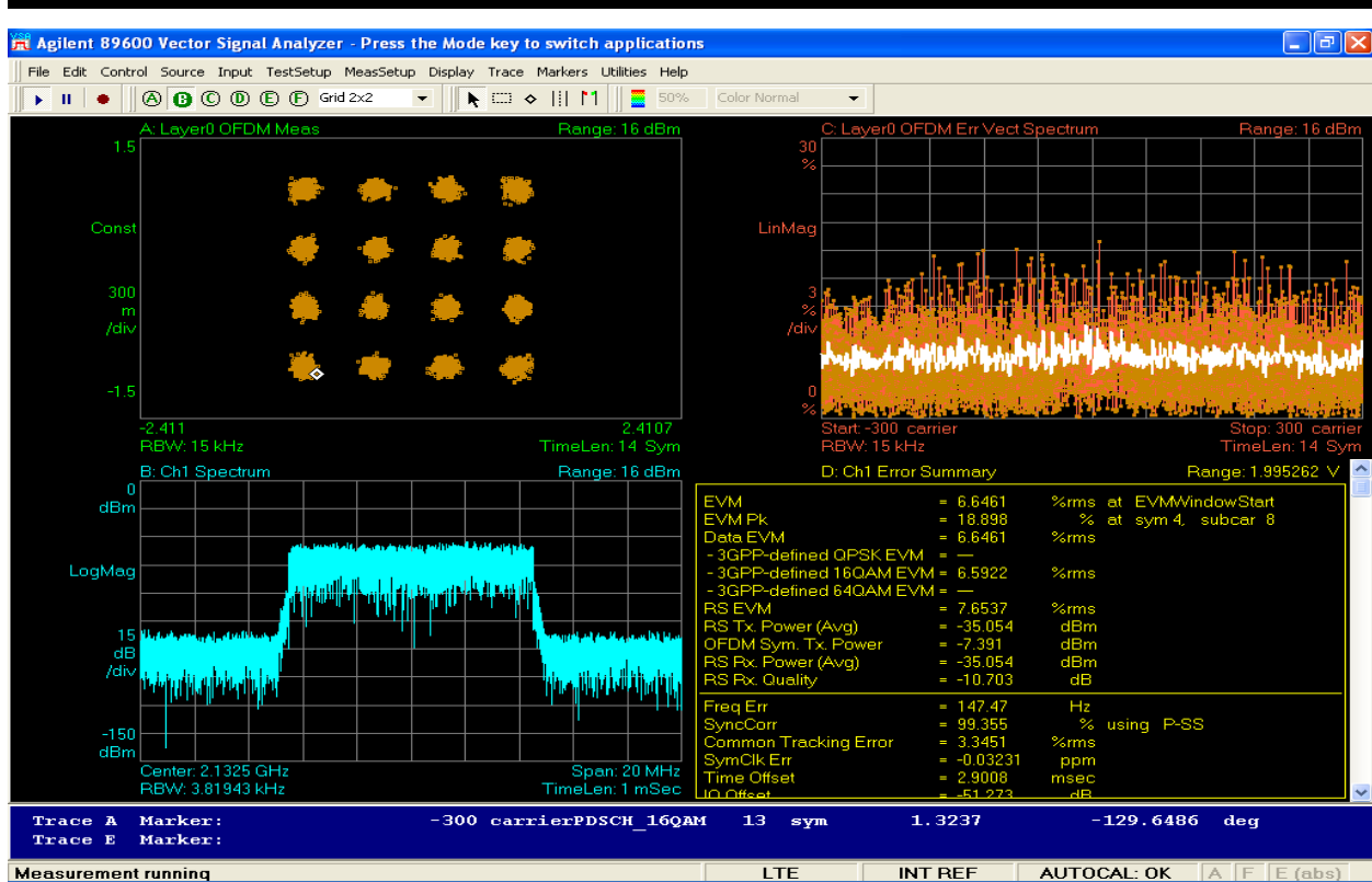
Figure 6-36 : 10MHz BW Modulation TX1_16QAM at 2132.5 MHz
