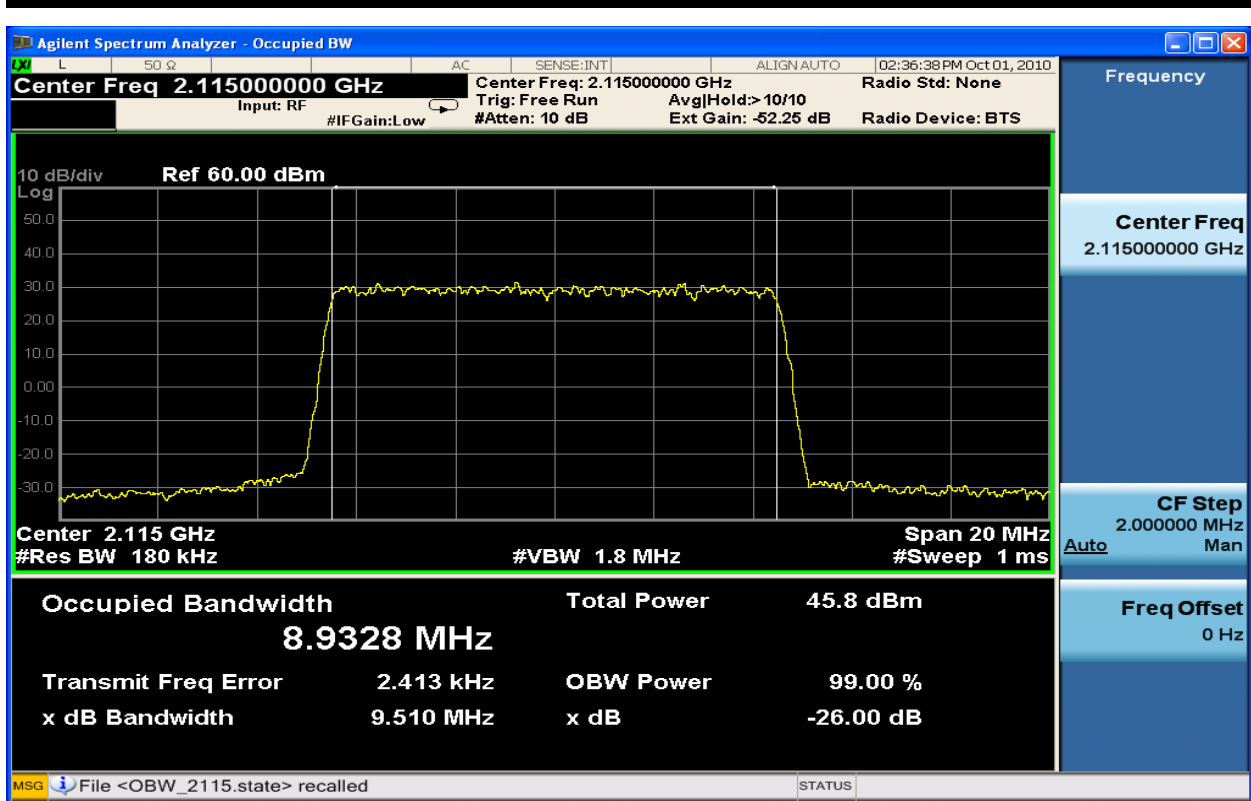
Figure 6-69: 10MHz Occupied Bandwidth TX1_QPSK at 2115.0 MHz
