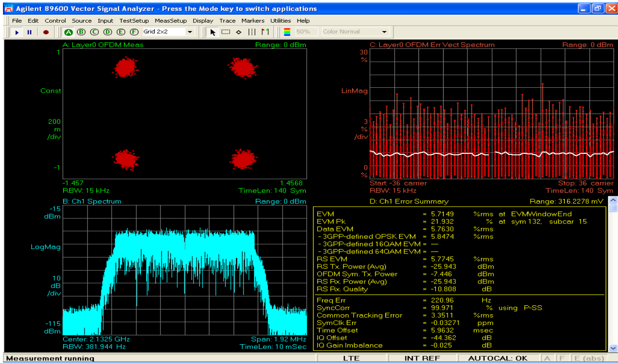
Figure 6-8: 1.4MHz BW Modulation TX1_QPSK at 2132.5 MHz
