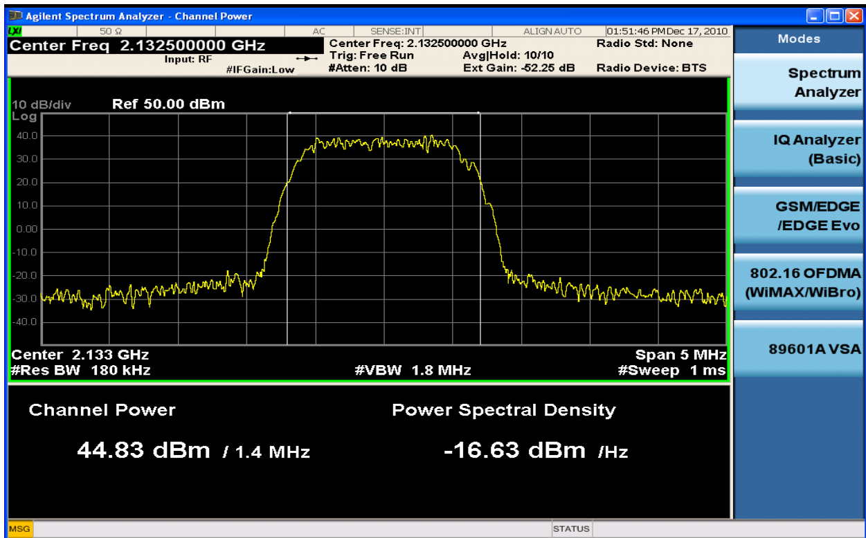
Figure 6-9 : 1.4MHz BW Channel Power TX1_QPSK at 2132.5 MHz
