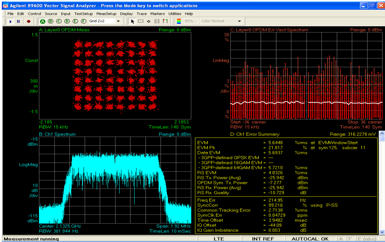
Figure 6-18: 1.4MHz BW Modulation TX2_64QAM at 2132.5 MHz
