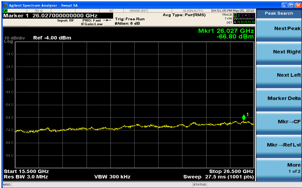
Figure 6-203 Spurious Emission TX1 64QAM 2115.0MHz - 10MHz (15.5GHz – 26.5GHz)
