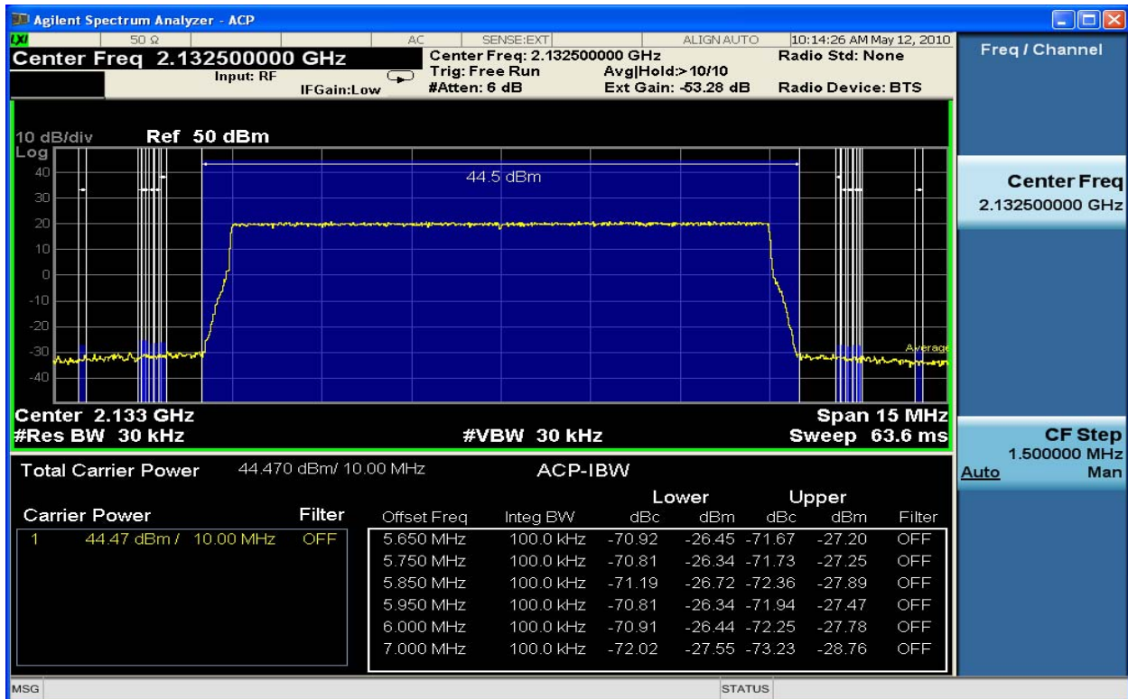
Figure 6-161 Spurious Emissions 2132.5MHz TX1_QPSK 10MHz Band Edge (ACP 650kHz – 2MHz)
