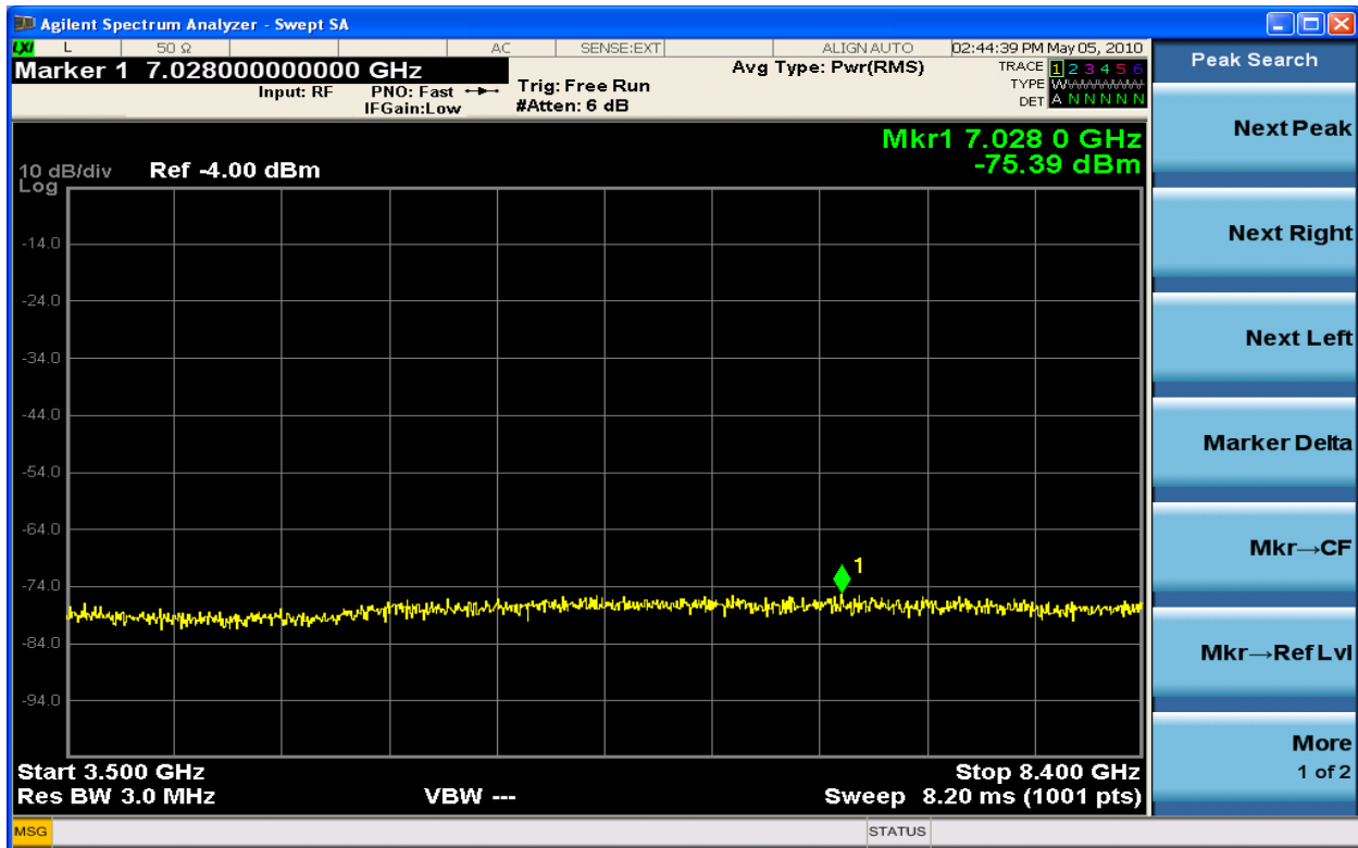
Figure 6-194 Spurious Emission TX2 64QAM 2115.0MHz - 10MHz (3.5GHz – 8.4GHz)
