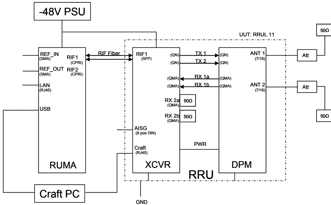
Figure 6-209 RRU EMC Set Up / Configuration
