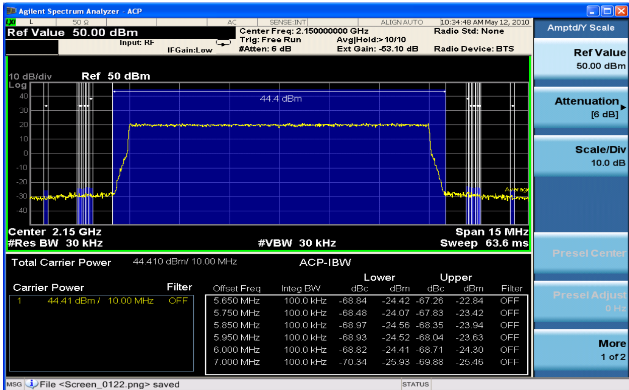
Figure 6-183 Spurious Emissions 2150.0MHz TX2_64QAM 10MHz Band Edge (ACP 650kHz – 2MHz)
