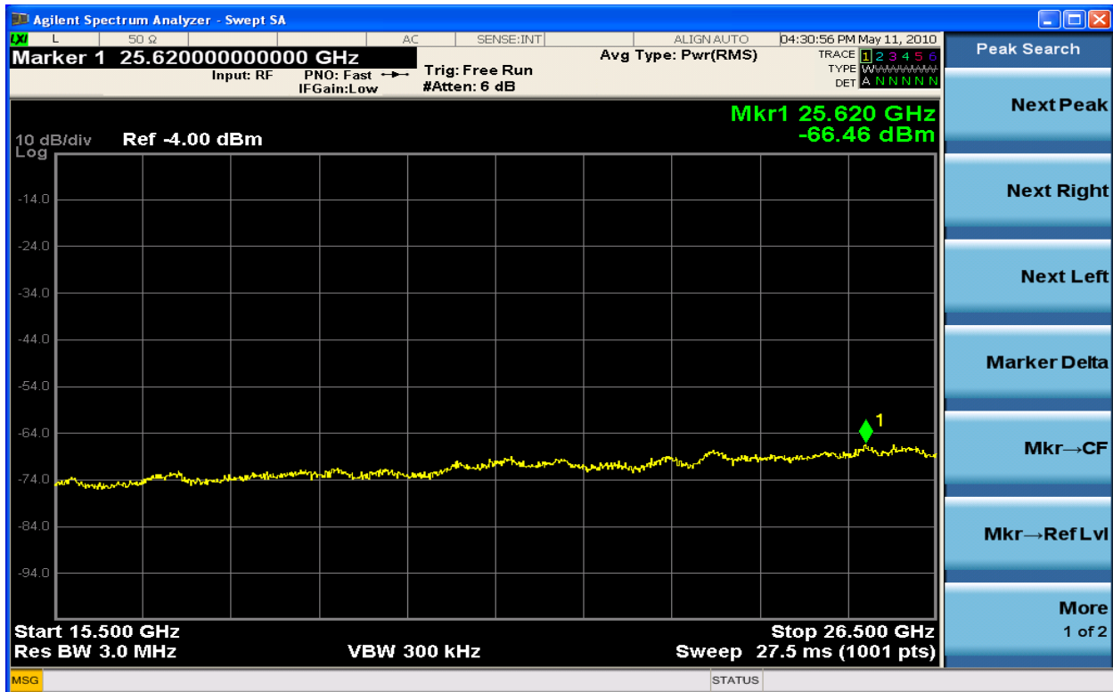
Figure 6-205 MXA (TX2) Noise Floor Reference (15.5GHz – 26.5GHz)
