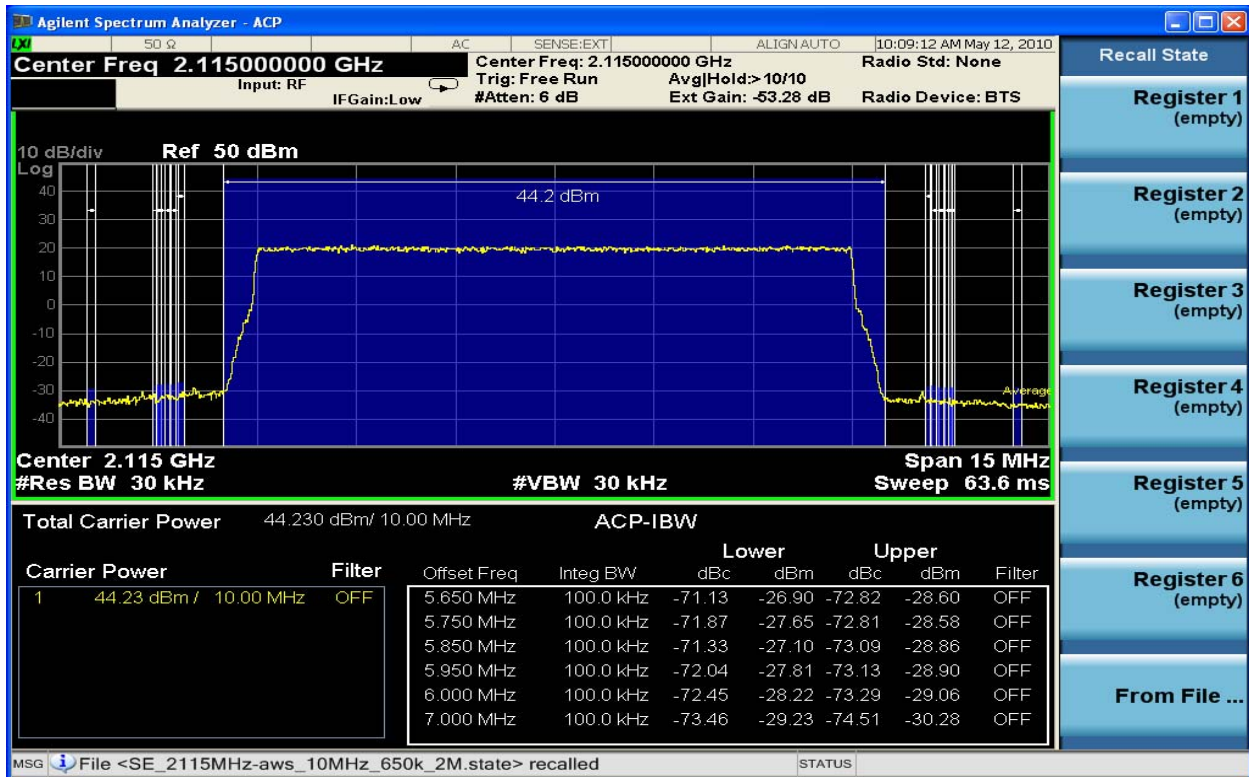
Figure 6-157 Spurious Emissions 2115.0MHz TX1_64QAM 10MHz Band Edge (ACP 650kHz – 2MHz)
