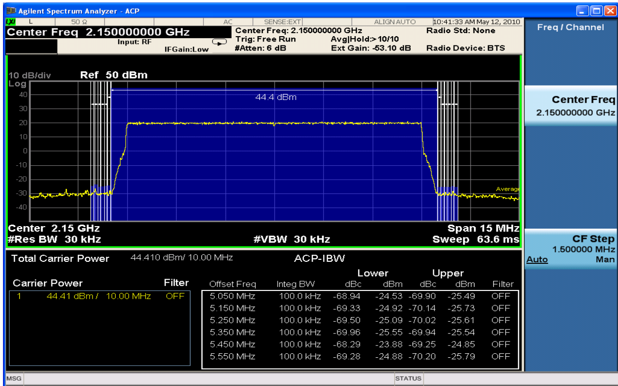
Figure 6-174 Spurious Emissions 2150.0MHz TX2_QPSK 10MHz Band Edge (ACP 15kHz – 550KHz)
