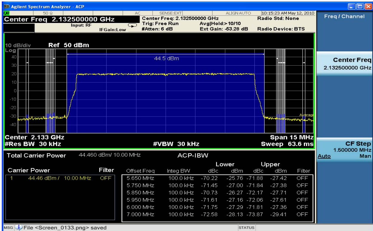
Figure 6-165 Spurious Emissions 2132.5MHz TX1_16QAM 10MHz Band Edge (ACP 650kHz – 2MHz)
