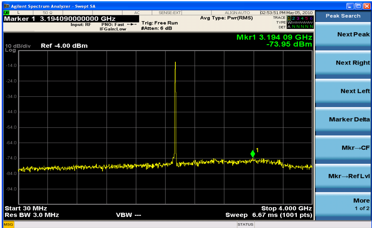
Figure 6-189 Spurious Emission TX2 64QAM 2150.0MHz - 10MHz (30MHz - 4GHz)
