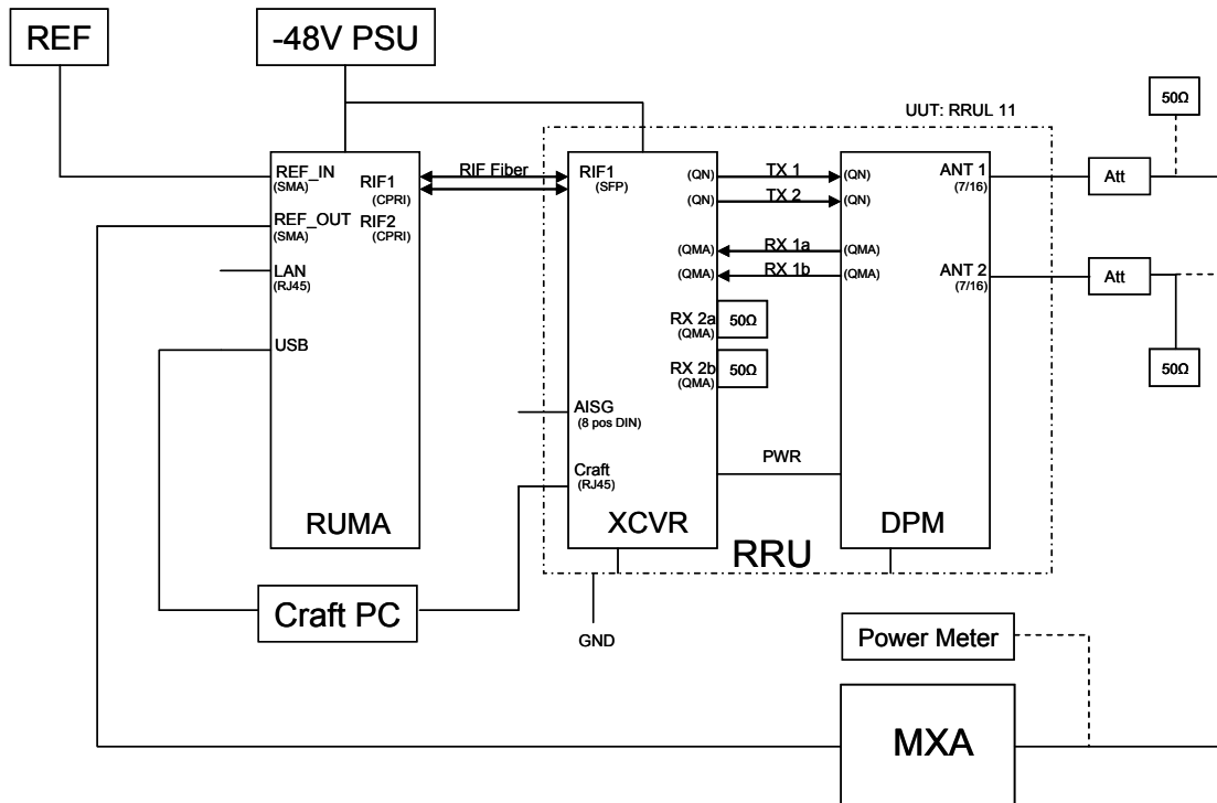
Figure 6-211 RRU Stability Set Up / Configuration
