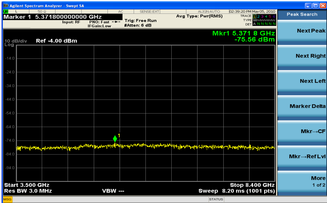
Figure 6-191 Spurious Emission TX1 64QAM 2115.0MHz - 10MHz (3.5GHz – 8.4GHz)
