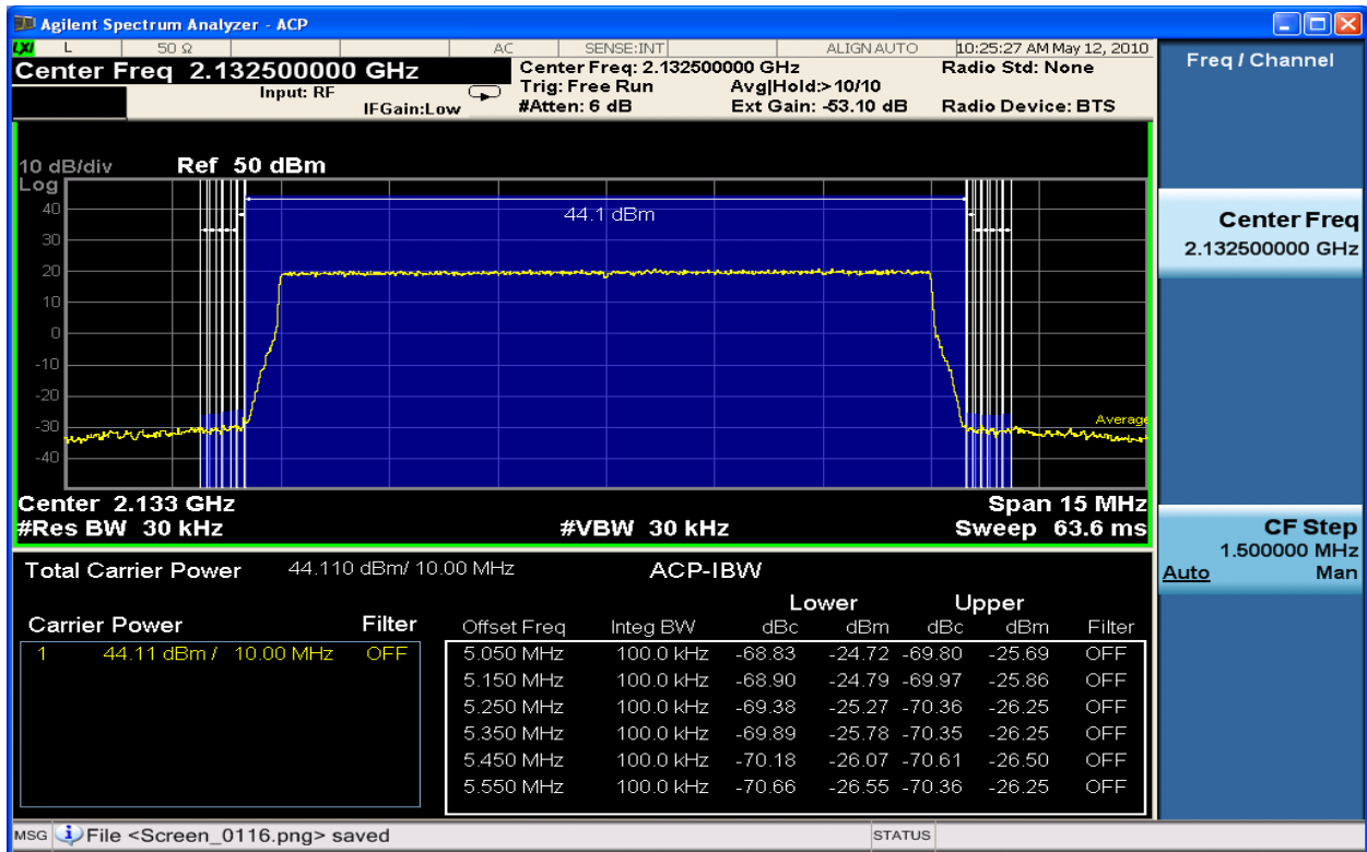
Figure 6-162 Spurious Emissions 2132.5MHz TX2_QPSK 10MHz Band Edge (ACP 15kHz – 550KHz)
