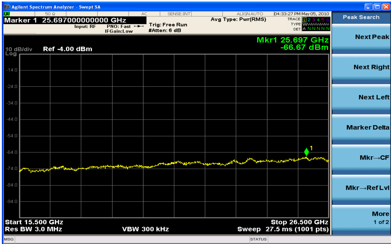
Figure 6-204 Spurious Emission TX1 64QAM 2150.0MHz – 10MHz (15.5GHz – 26.5GHz)
