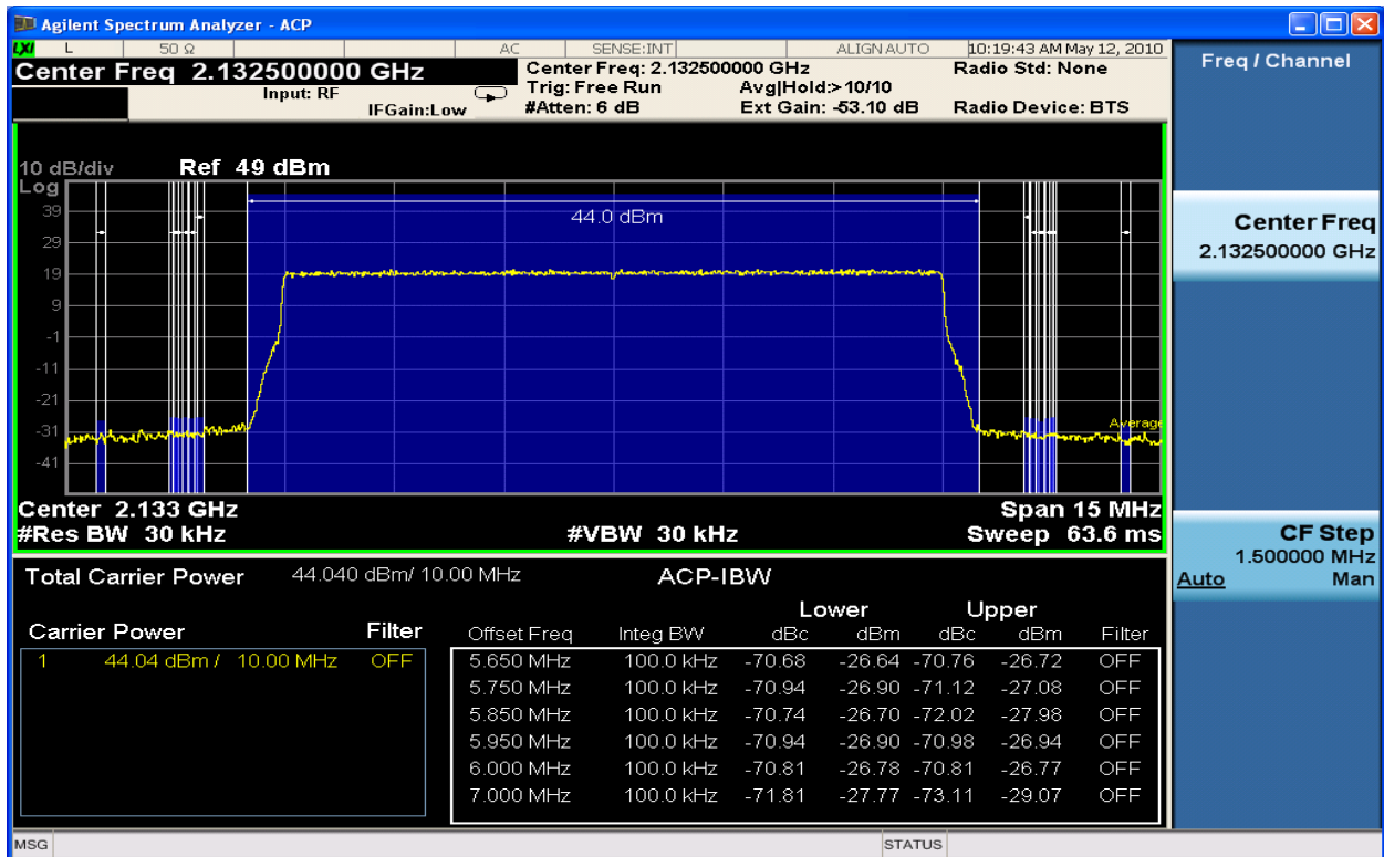
Figure 6-163 Spurious Emissions 2132.5MHz TX2_QPSK 10MHz Band Edge (ACP 650kHz – 2MHz)
