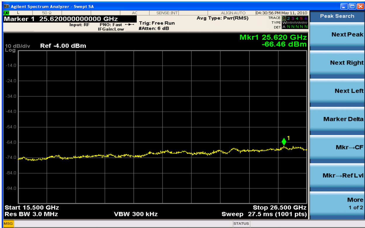
Figure 6-202 MXA (TX1) Noise Floor Reference (15.5GHz – 26.5GHz)
