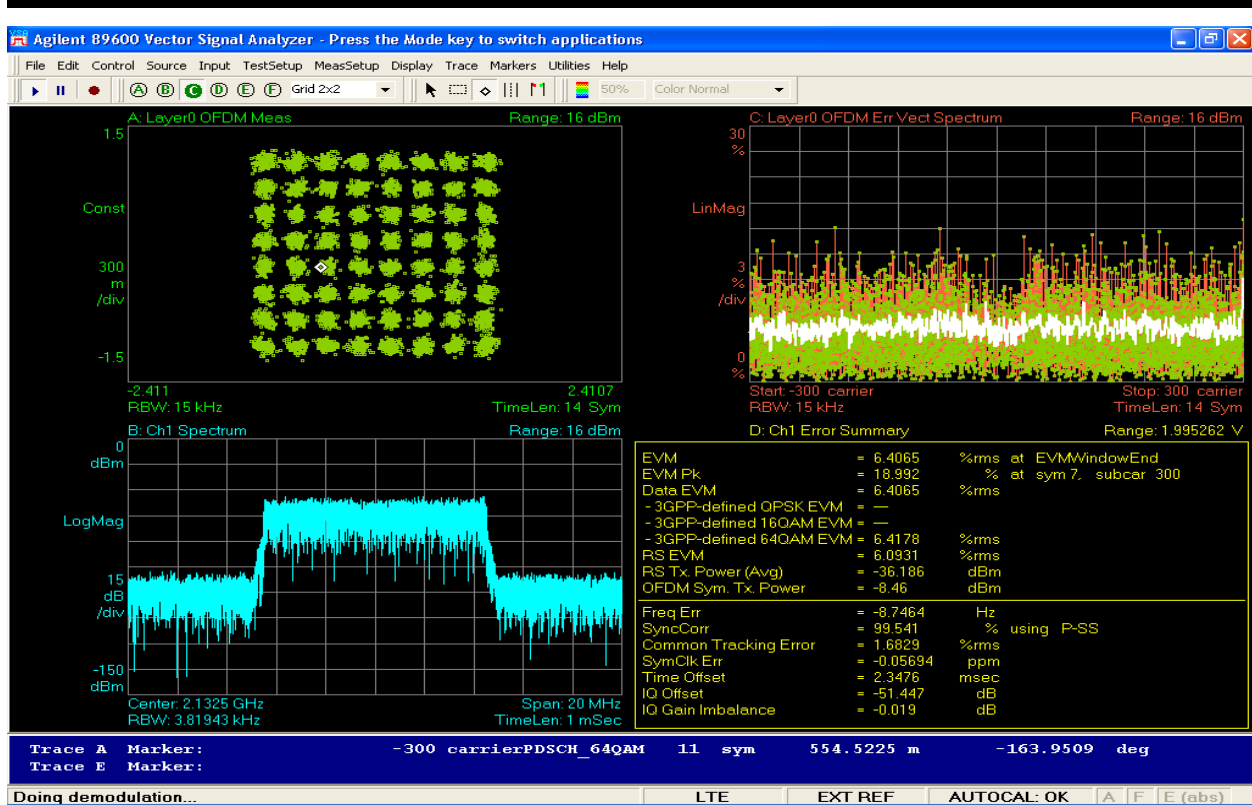
Figure 6-218 Stability 10MHz @ +30C
