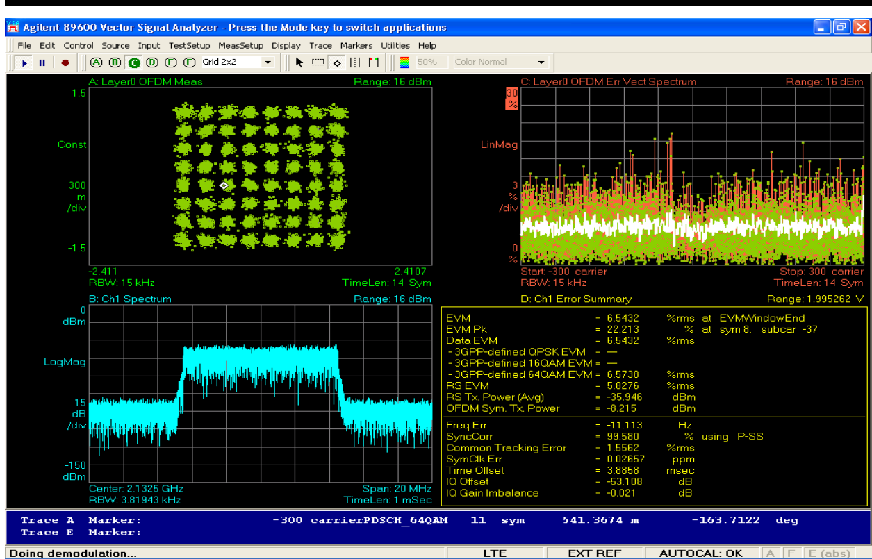
Figure 6-212 Stability - 10MHz @ -30C
