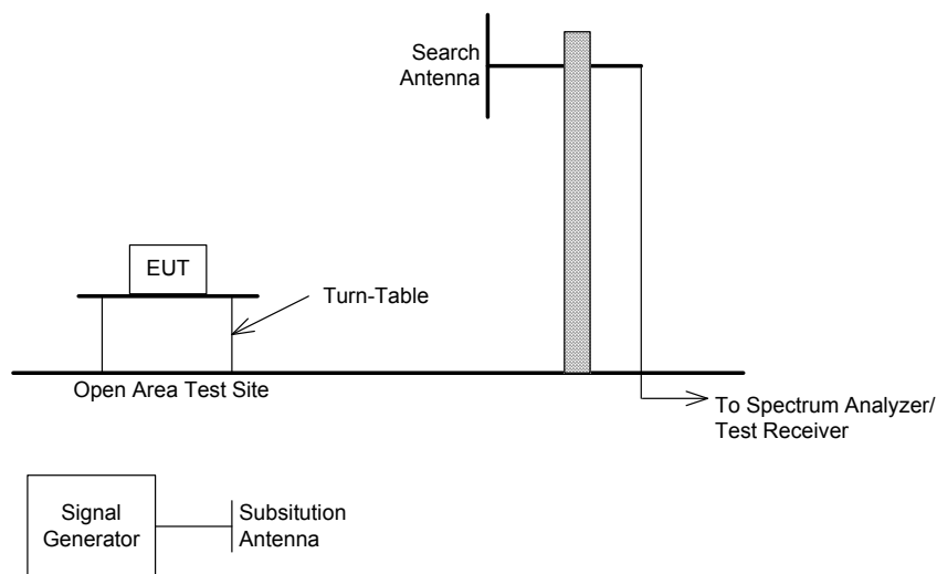
Figure 6-208 RRU Field Strength Set Up / Configuration
