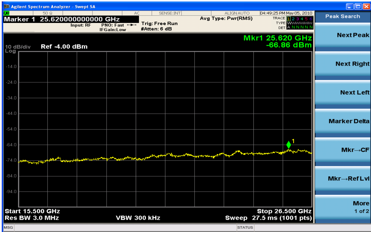
Figure 6-206 Spurious Emission TX2 64QAM 2115.0MHz - 10MHz (15.5GHz – 26.5GHz)
