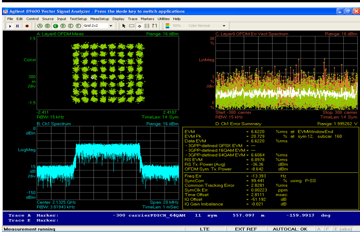
Figure 6-220 Stability 10MHz @ +50C
