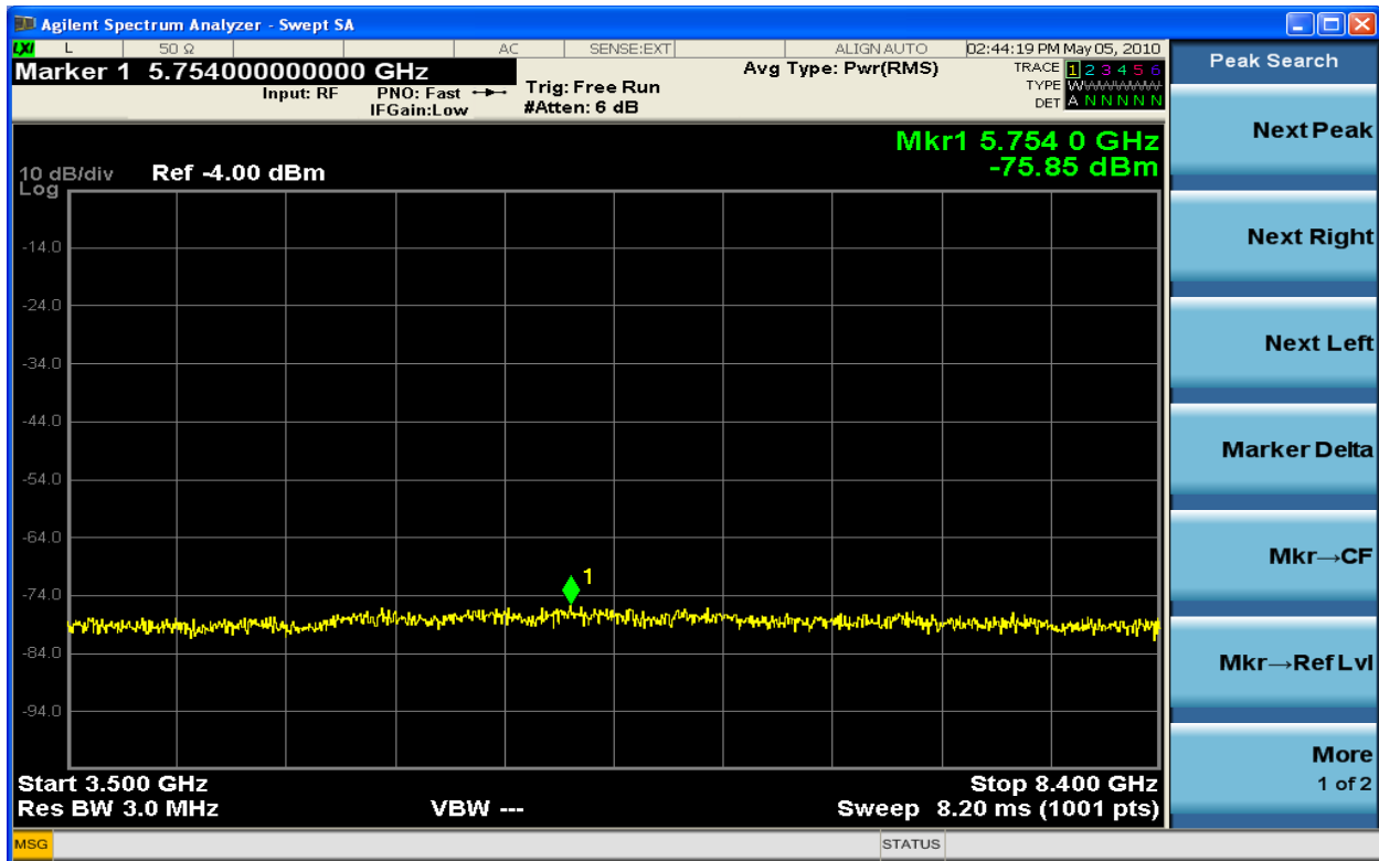
Figure 6-192 Spurious Emission TX1 64QAM 2150.0MHz - 10MHz (3.5GHz – 8.4GHz)
