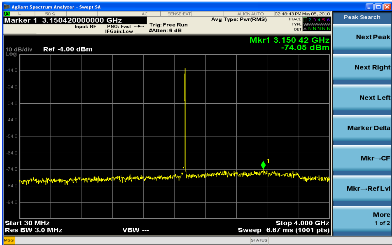
Figure 6-186 Spurious Emission TX1 64QAM 2150.0MHz - 10MHz (30MHz - 4GHz)
