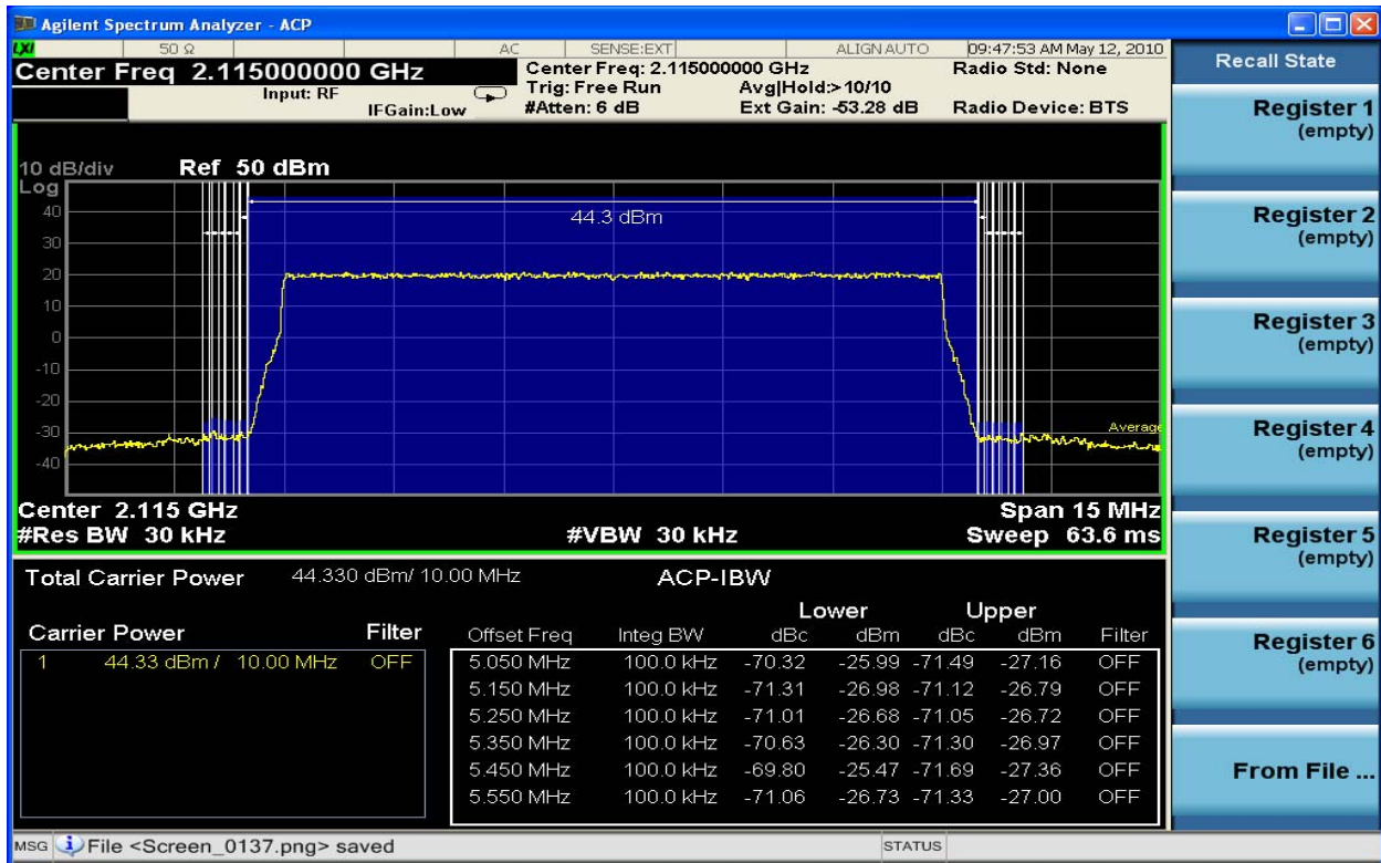
Figure 6-156 Spurious Emissions 2115.0MHz TX1_64QAM 10MHz Band Edge (ACP 15kHz – 550KHz)
