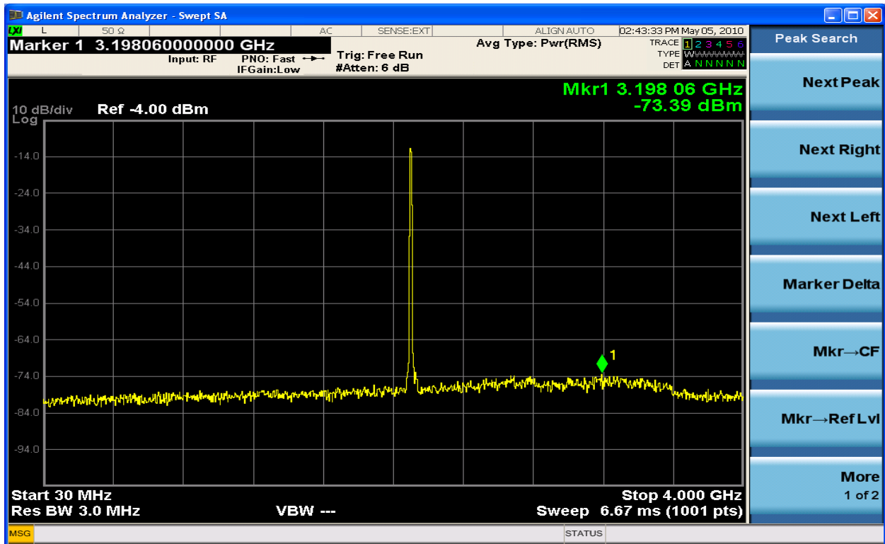
Figure 6-188 Spurious Emission TX2 64QAM 2115.0MHz - 10MHz (30MHz - 4GHz)
