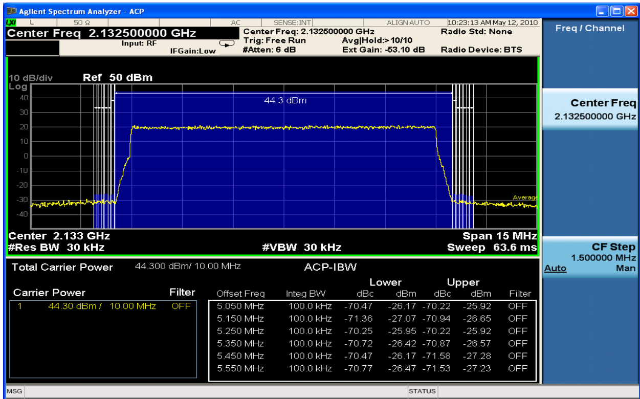
Figure 6-170 Spurious Emissions 2132.5MHz TX2_64QAM 10MHz Band Edge (ACP 15kHz – 550kHz)
