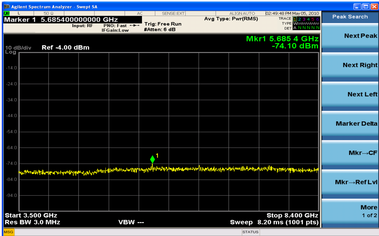
Figure 6-195 Spurious Emission TX2 64QAM 2150.0MHz – 10MHz (3.5GHz – 8.4GHz)
