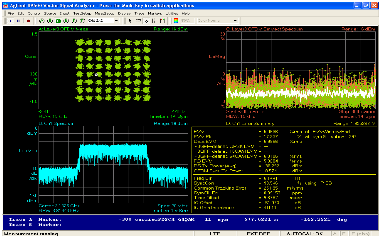
Figure 6-217 Stability 10MHz @ +20C
