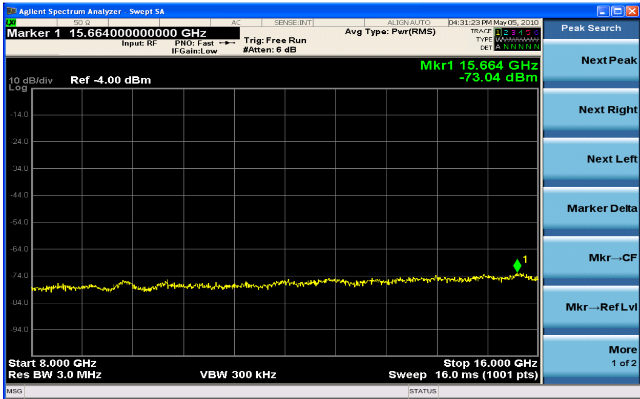
Figure 6-198 Spurious Emission TX1 64QAM 2150.0MHz – 10MHz (8GHz- 16GHz)
