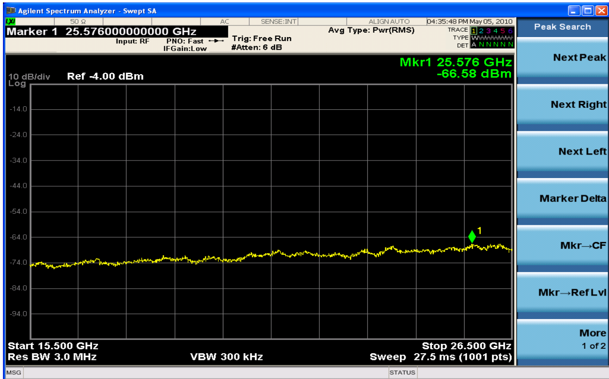
Figure 6-207 Spurious Emission TX2 64QAM 2150.0MHz – 10MHz (15.5GHz – 26.5GHz)
