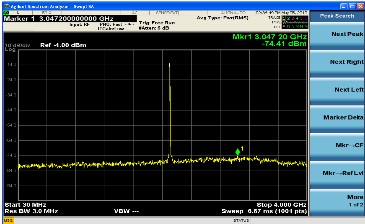
Figure 6-185 Spurious Emission TX1 64QAM 2115.0MHz - 10MHz (30MHz - 4GHz)
