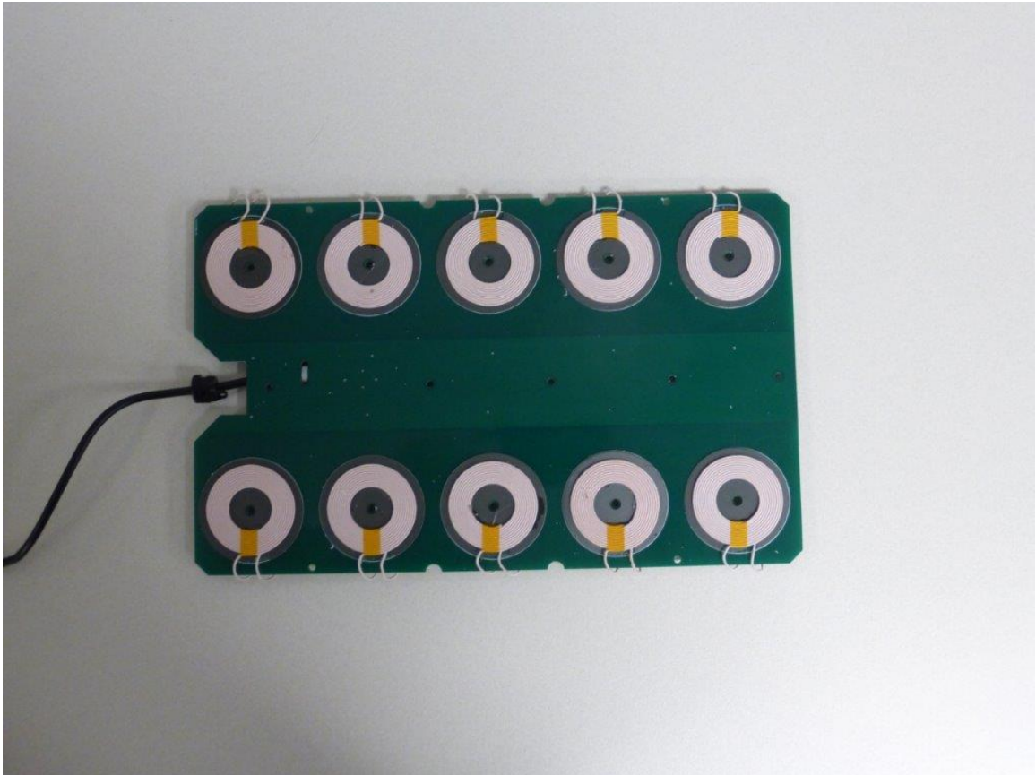
Figure 2- Antenna side of Wi-Fi Tag Charger
