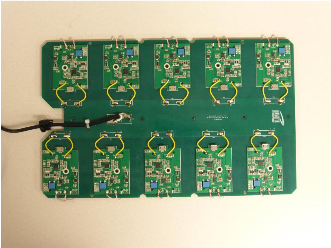
Figure 1- Qi Module side of Wi-Fi Tag Charger
