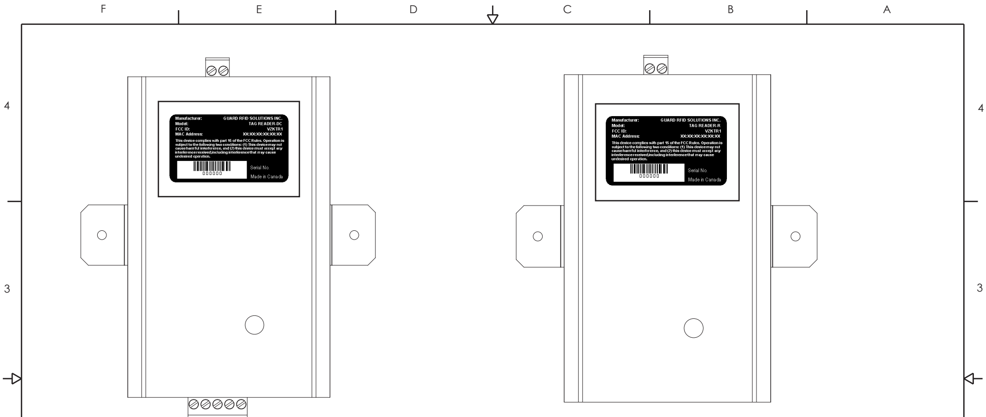
A. TAG READER- DC, FCC/SN LABEL PLACEMENT LOCATION
