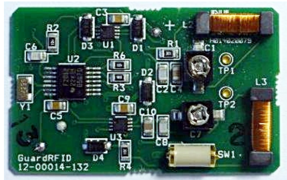
- EUT: Internal View, Top without Battery
