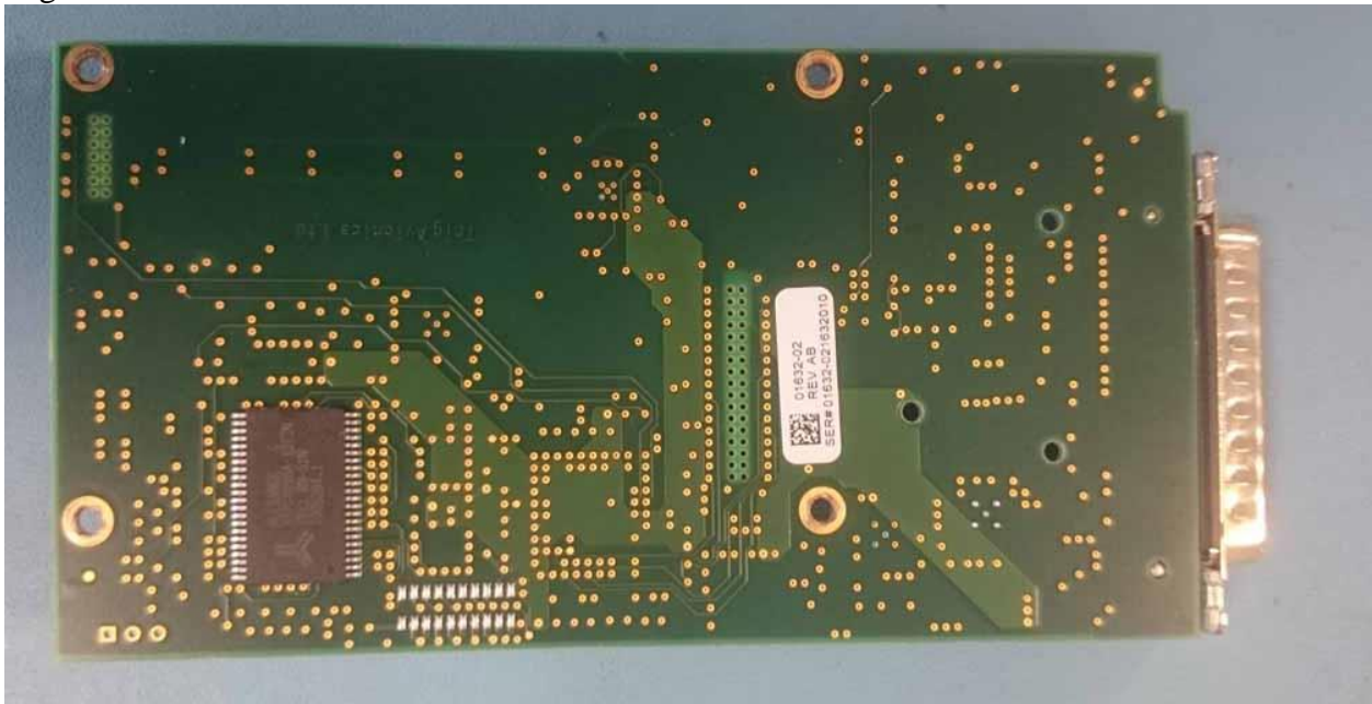
Digital Bottom
