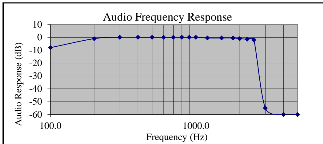
Figure 3 Audio Frequency Response / Modulation Characteristics
