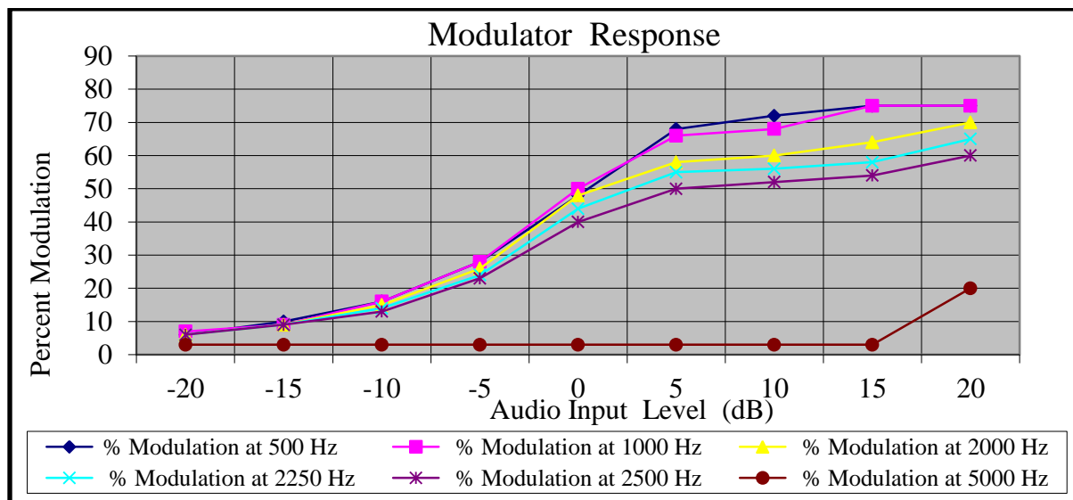
Figure 2 Modulation Characteristics
