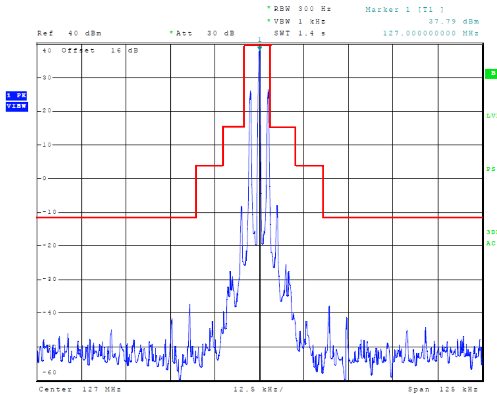
Figure 10 Emission Mask
