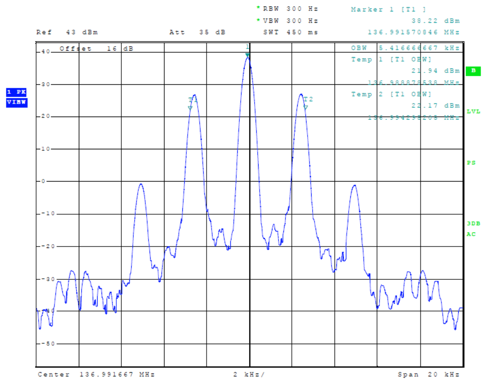
Figure 8 Occupied Band Width Carrier frequency 136.992
