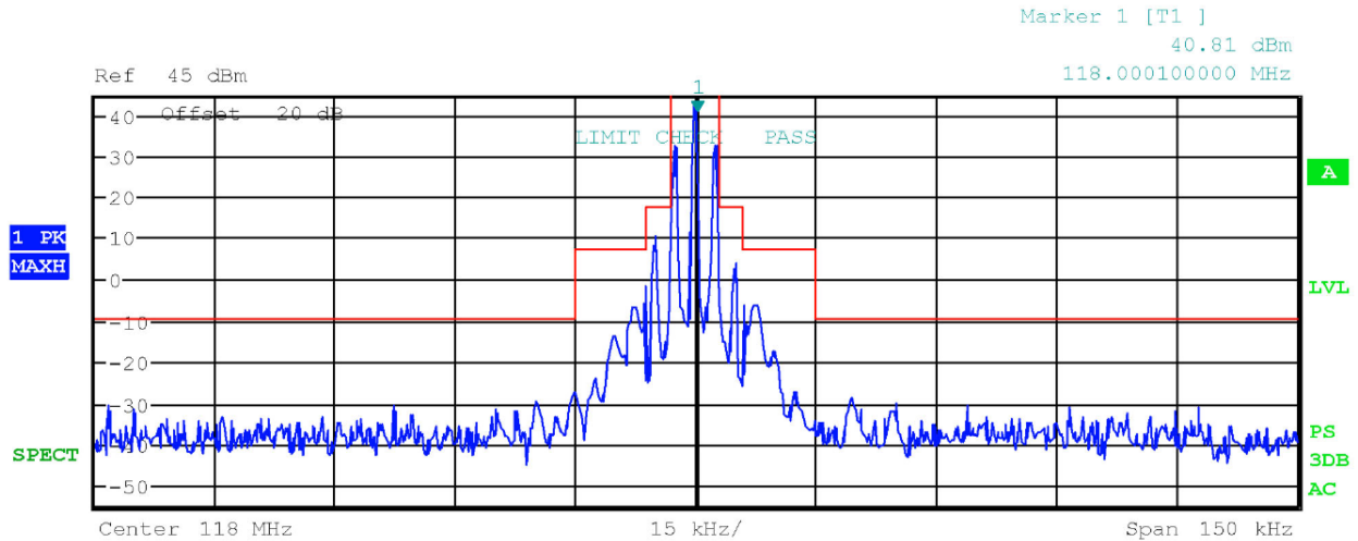
Figure 7 Spectral Emission Mask at Antenna Terminal
