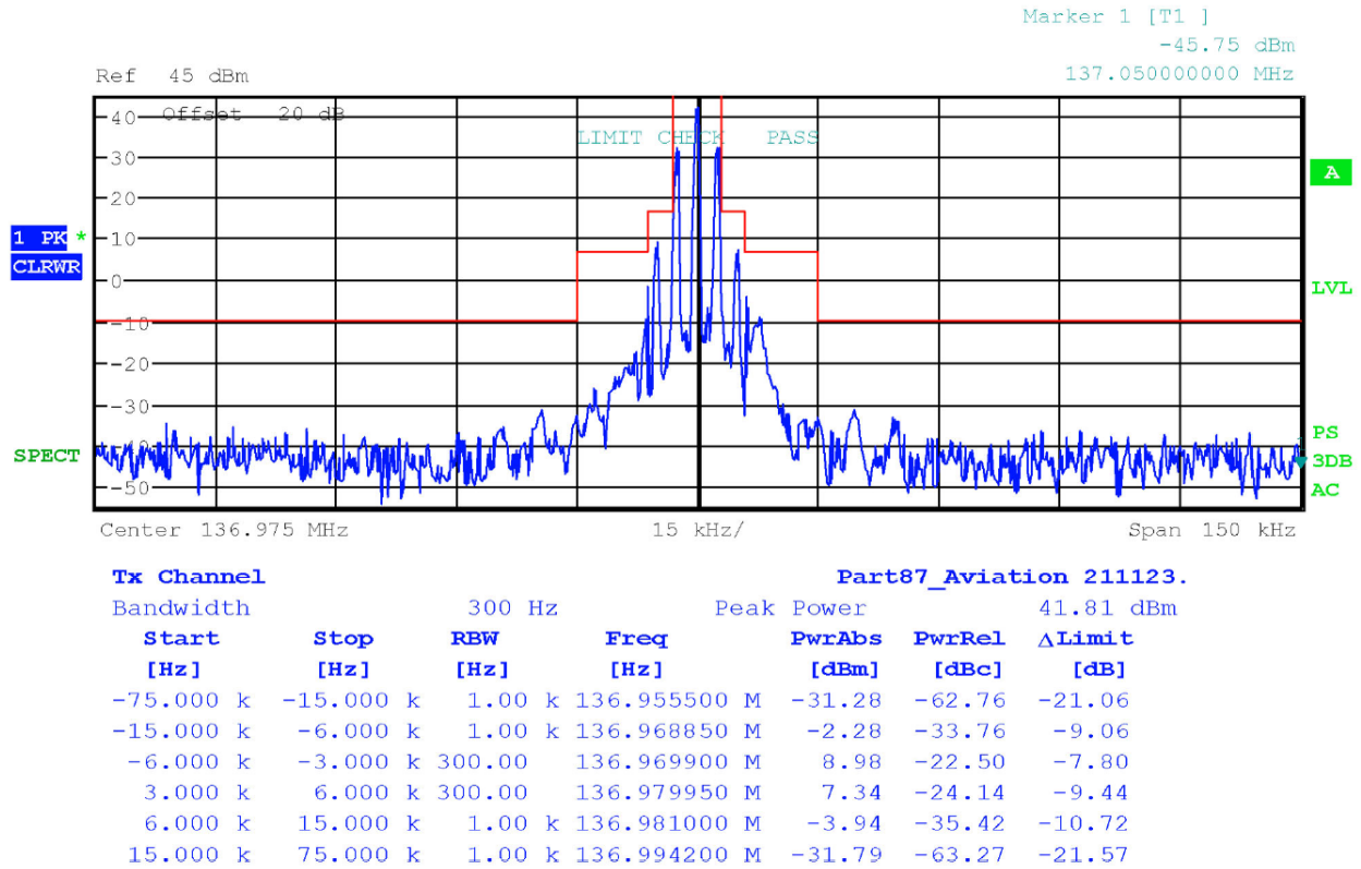
Figure 6 Spurious Emissions at Antenna Terminal
