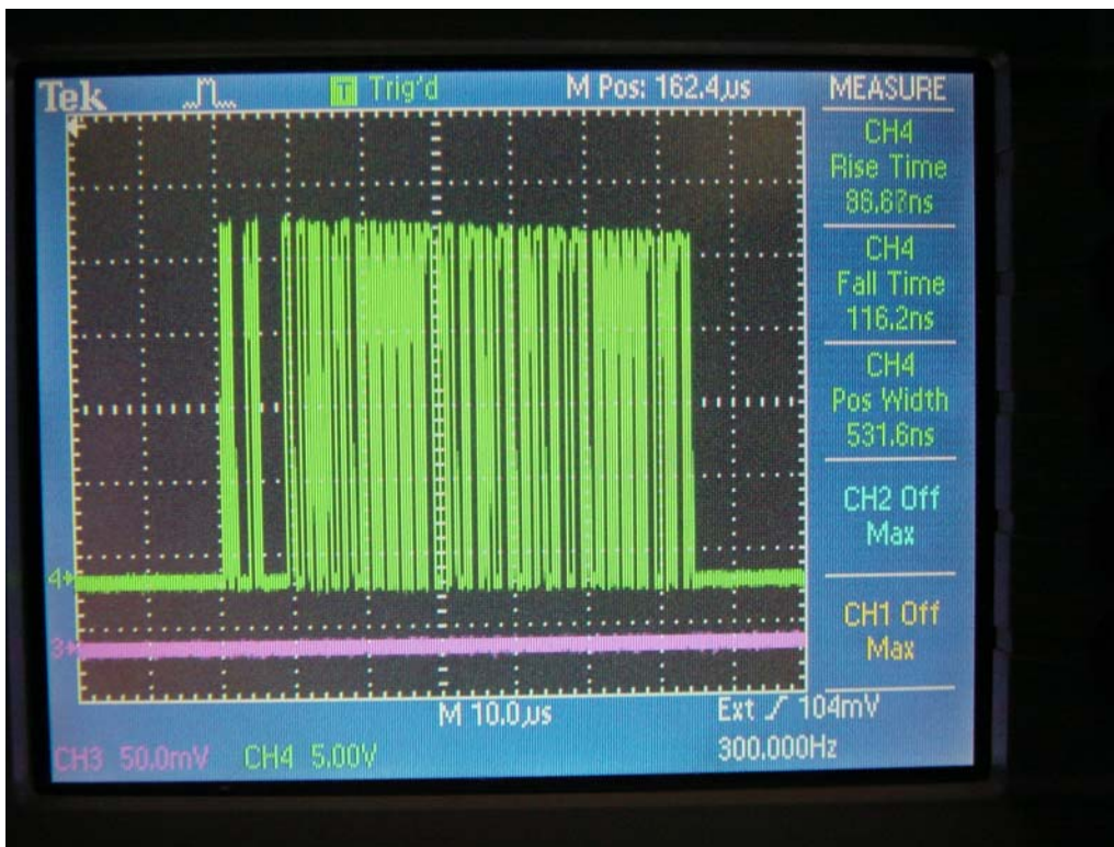
Figure 3 Modulation characteristics
