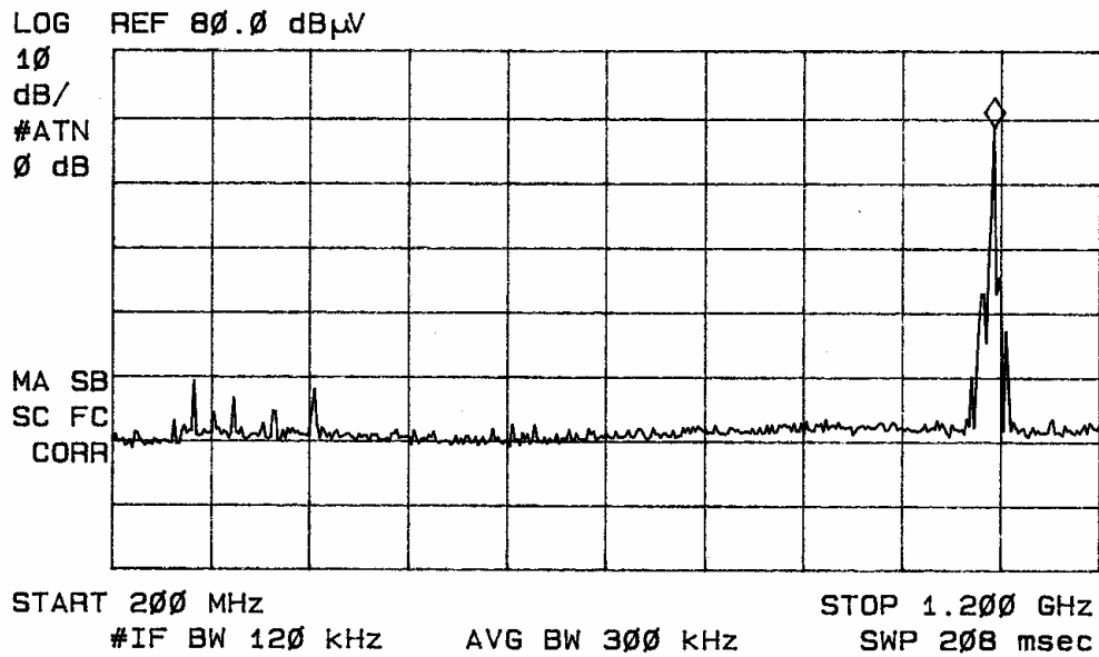
Figure 9 Radiated emissions taken at 1 meter in screen room.
