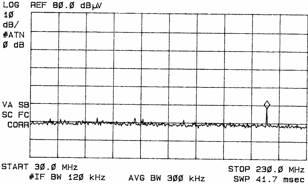
Figure 8 Radiated emissions taken at 1 meter in screen room.
